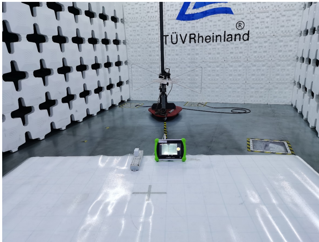
Photograph 3: Set-up photo for Radiated Emissions Below 1GHz
