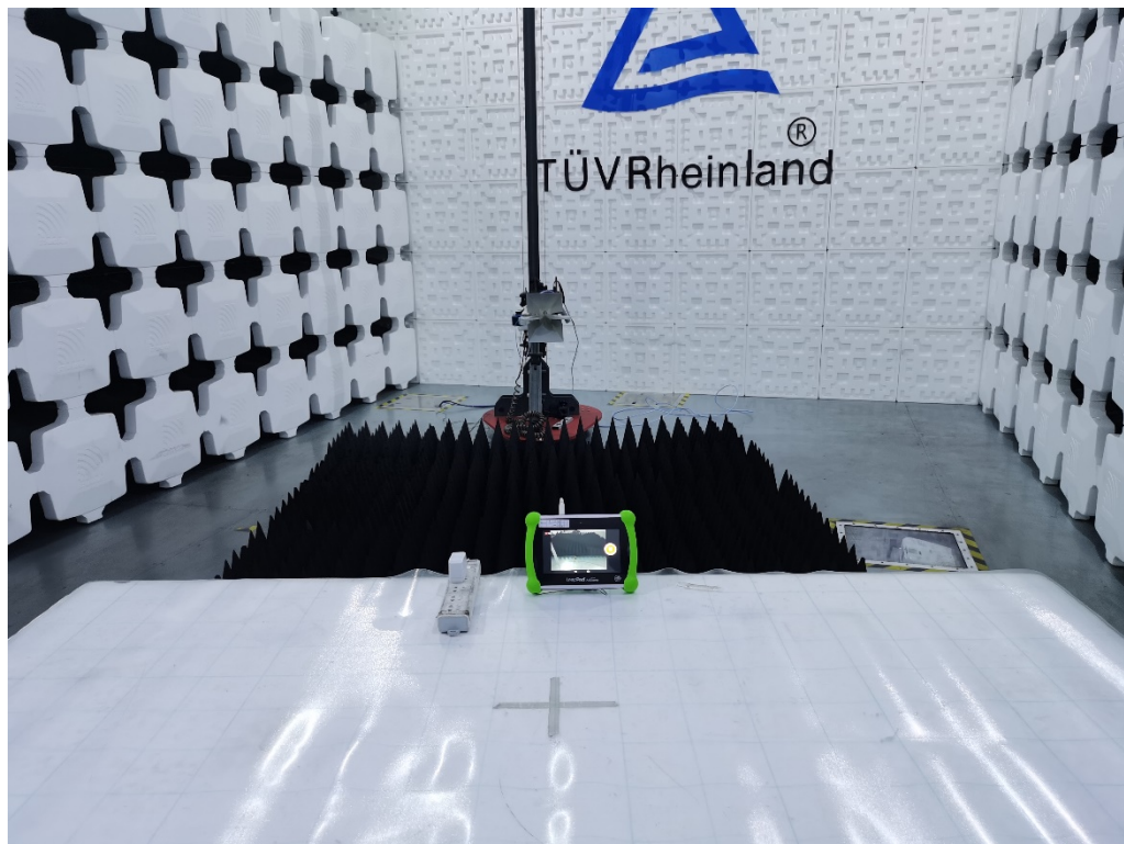
Photograph 4: Set-up photo for Radiated Emissions Above 1GHz
