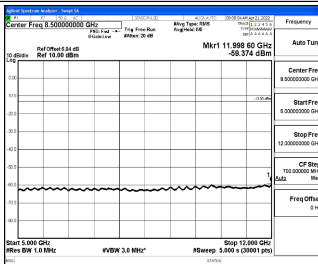
Band26-3MHz-QPSK-26805-1-0-Low-5000-12000--59.37-PASS
