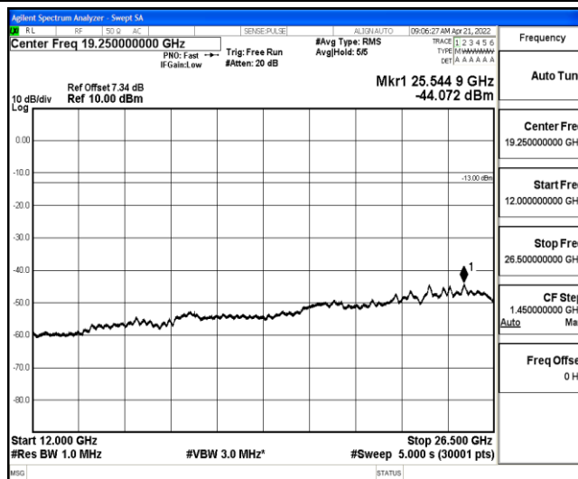
Band26-3MHz-16QAM-26915-1-0-Low-12000-26500--44.07-PASS
