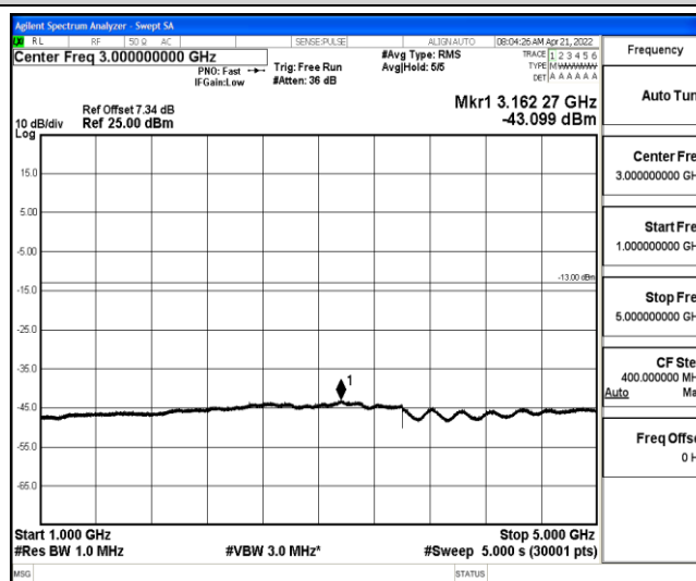
Band26-5MHz-16QAM-26915-1-0-Low-1000-5000--43.1-PASS
