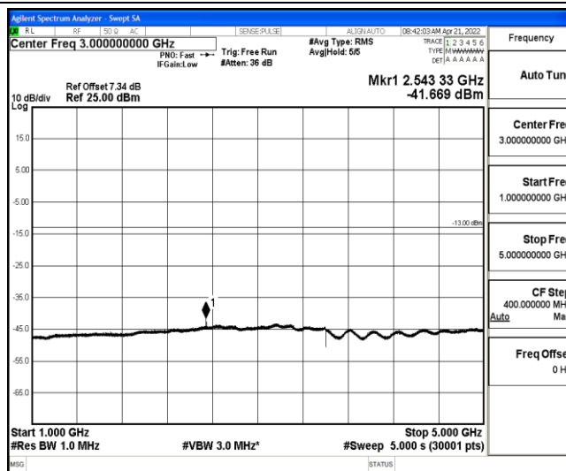
Band26-1.4MHz-16QAM-27033-1-0-High-1000-5000--41.67-PASS
