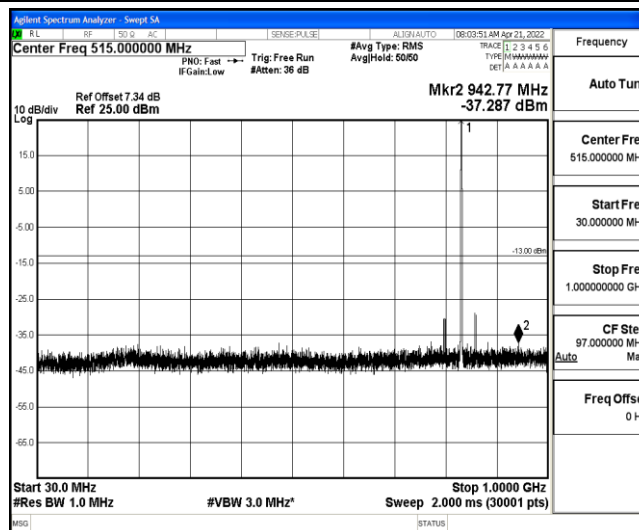
Band26-5MHz-16QAM-26915-1-0-Low-30-1000--37.29-PASS
