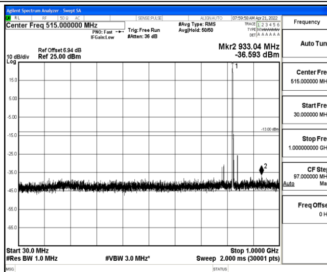
Band26-5MHz-16QAM-26815-1-0-Low-30-1000--36.59-PASS
