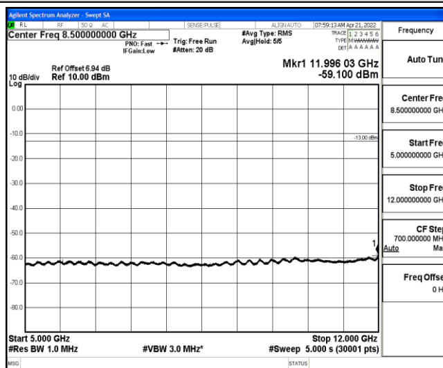
Band26-5MHz-QPSK-26815-1-0-Low-5000-12000--59.1-PASS
