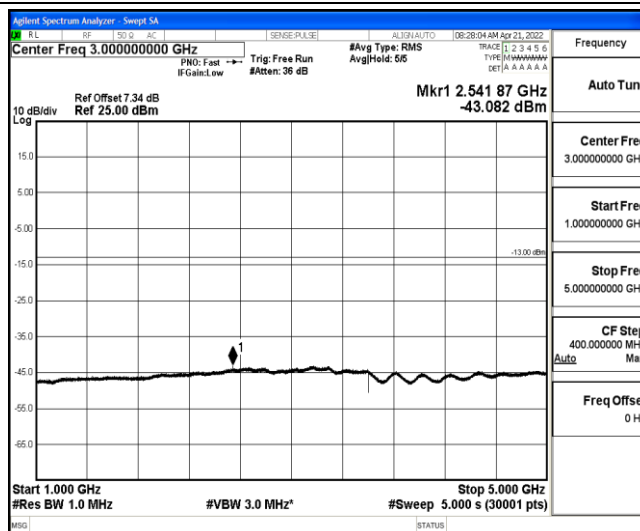
Band26-10MHz-QPSK-26990-1-0-High-1000-5000--43.08-PASS
