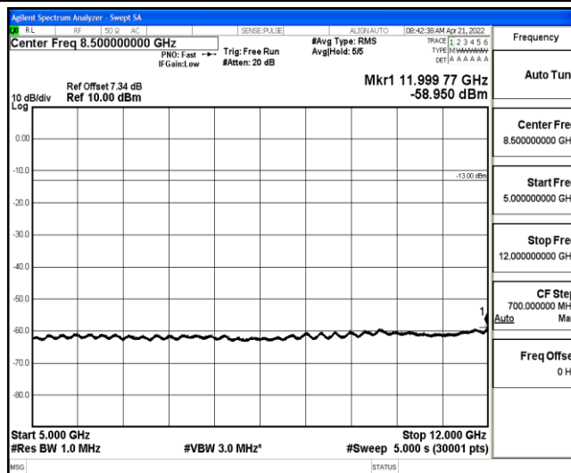
Band26-1.4MHz-16QAM-27033-1-0-High-5000-12000--58.95-PASS
