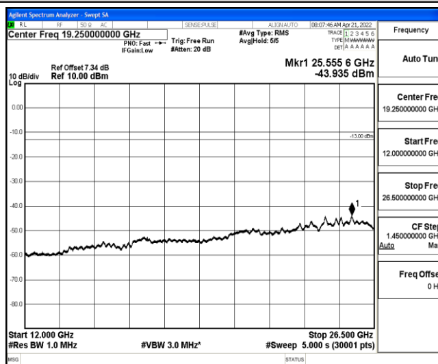
Band26-5MHz-QPSK-27015-1-0-High-12000-26500--43.94-PASS
