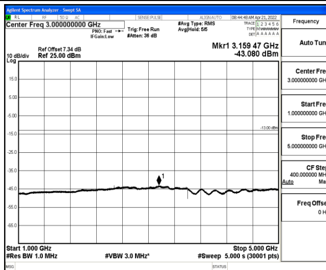
Band26-15MHz-QPSK-26865-1-0-Low-1000-5000--43.08-PASS
