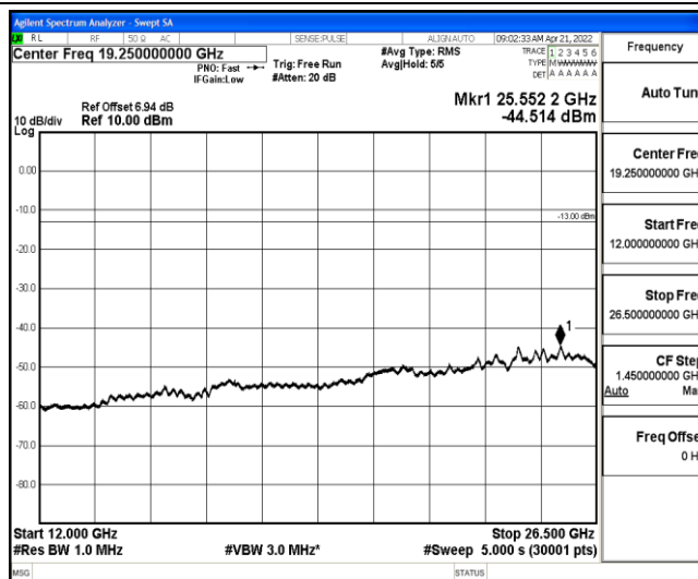
Band26-3MHz-16QAM-26805-1-0-Low-12000-26500--44.51-PASS
