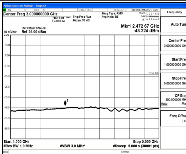
Band26-1.4MHz-16QAM-26797-1-0-Low-1000-5000--43.22-PASS
