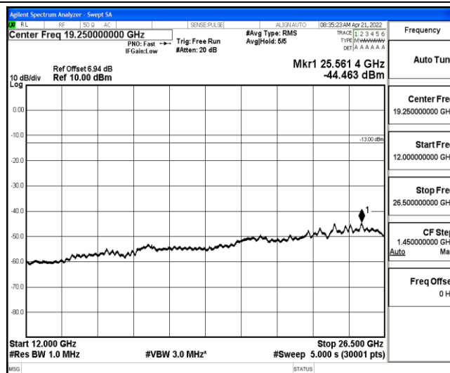
Band26-1.4MHz-16QAM-26797-1-0-Low-12000-26500--44.46-PASS
