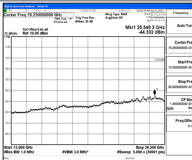
Band26-3MHz-QPSK-26805-1-0-Low-12000-26500--44.33-PASS
