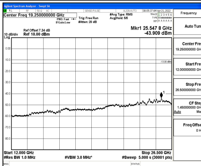
Band26-5MHz-16QAM-26915-1-0-Low-12000-26500--43.91-PASS
