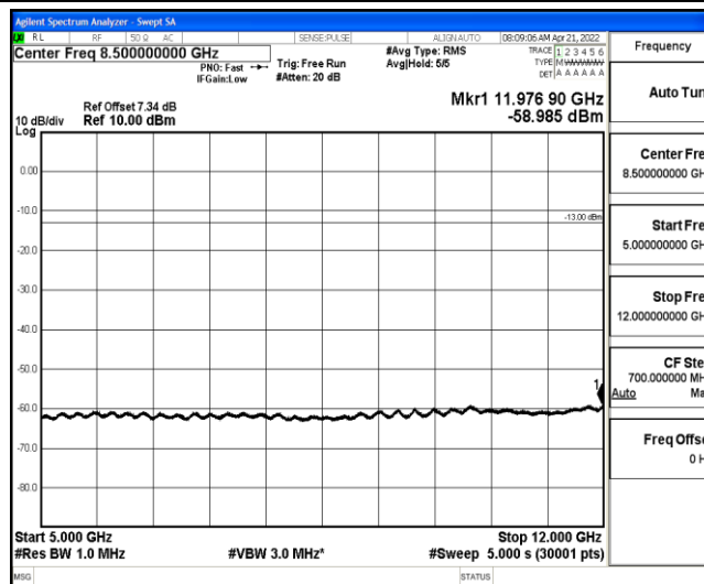
Band26-5MHz-16QAM-27015-1-0-High-5000-12000--58.99-PASS
