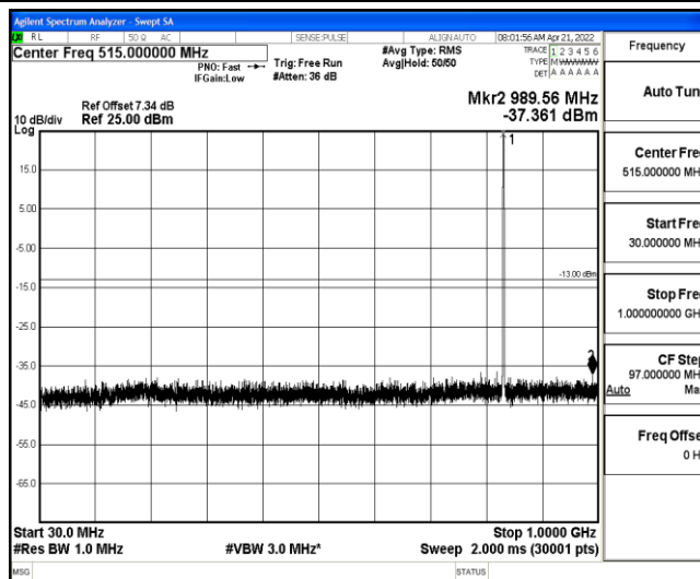
Band26-5MHz-QPSK-26915-1-0-Low-30-1000--37.36-PASS
