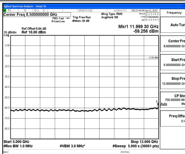
Band26-10MHz-16QAM-26840-1-0-Low-5000-12000--59.26-PASS
