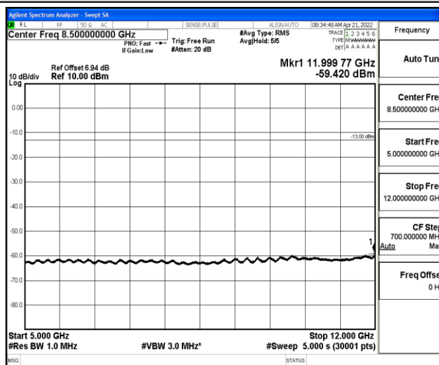
Band26-1.4MHz-16QAM-26797-1-0-Low-5000-12000--59.42-PASS
