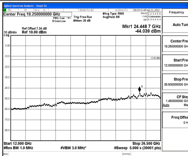
Band26-5MHz-QPSK-26915-1-0-Low-12000-26500--44.04-PASS
