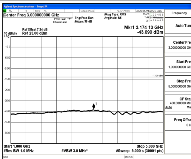
Band26-10MHz-16QAM-26915-1-0-Low-1000-5000--43.09-PASS
