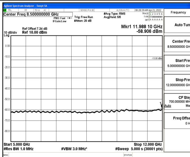
Band26-10MHz-QPSK-26990-1-0-High-5000-12000--58.91-PASS
