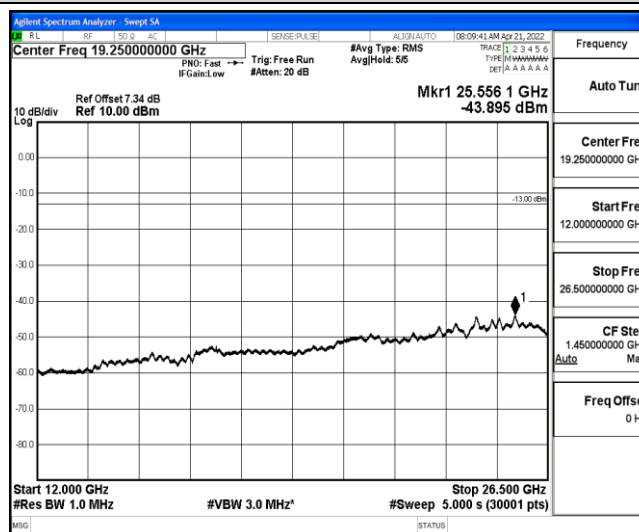
Band26-5MHz-16QAM-27015-1-0-High-12000-26500--43.9-PASS
