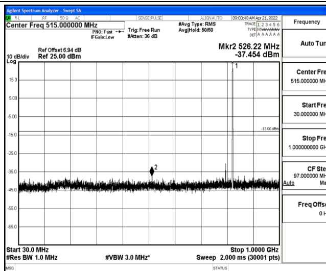
Band26-3MHz-16QAM-26805-1-0-Low-30-1000--37.45-PASS
