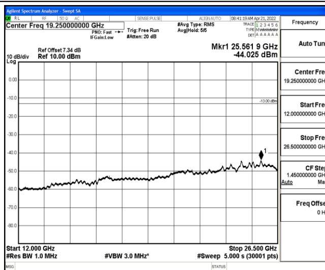
Band26-1.4MHz-QPSK-27033-1-0-High-12000-26500--44.03-PASS
