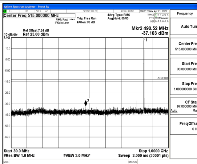
Band26-3MHz-QPSK-27025-1-0-High-30-1000--37.18-PASS
