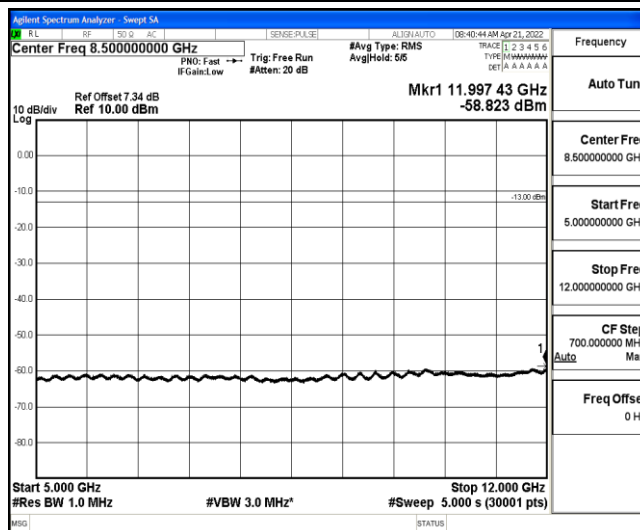
Band26-1.4MHz-QPSK-27033-1-0-High-5000-12000--58.82-PASS
