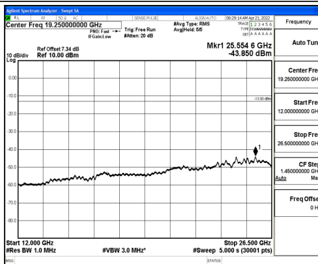
Band26-10MHz-QPSK-26990-1-0-High-12000-26500--43.85-PASS
