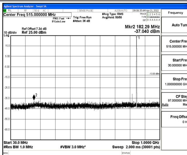
Band26-3MHz-16QAM-27025-1-0-High-30-1000--37.04-PASS
