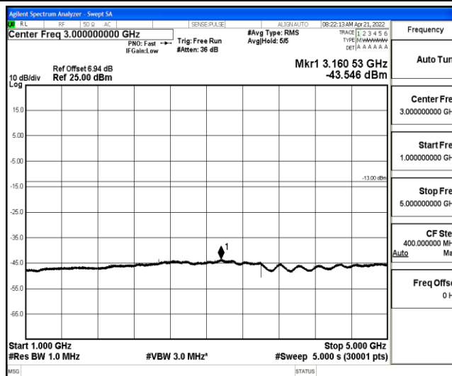
Band26-10MHz-16QAM-26840-1-0-Low-1000-5000--43.55-PASS
