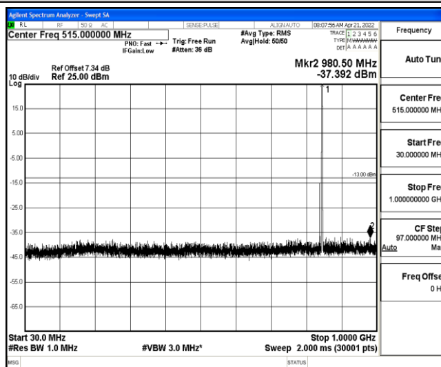
Band26-5MHz-16QAM-27015-1-0-High-30-1000--37.39-PASS
