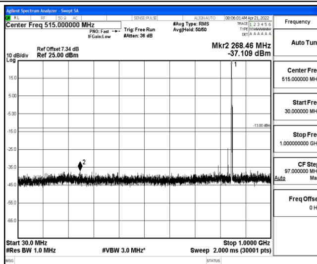
Band26-5MHz-QPSK-27015-1-0-High-30-1000--37.11-PASS
