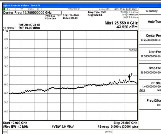
Band26-10MHz-16QAM-26990-1-0-High-12000-26500--43.92-PASS
