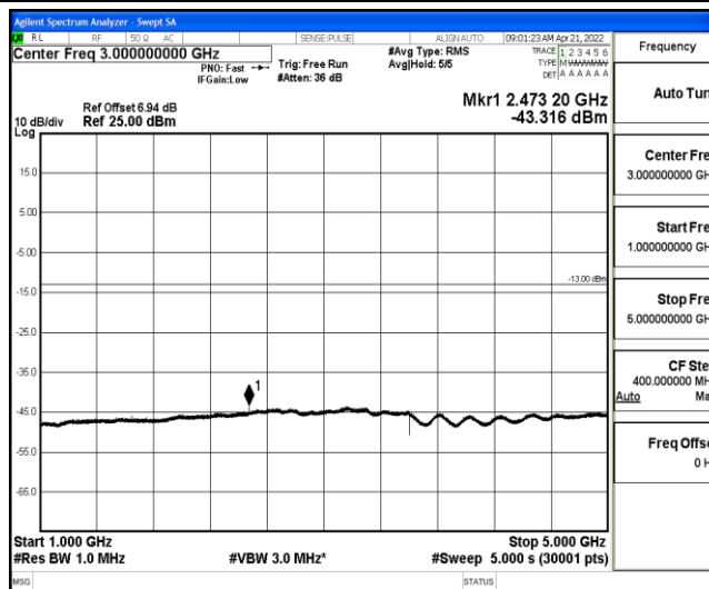
Band26-3MHz-16QAM-26805-1-0-Low-1000-5000--43.32-PASS
