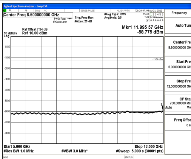
Band26-10MHz-QPSK-26915-1-0-Low-5000-12000--58.78-PASS
