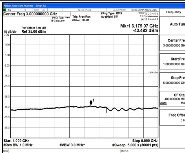
Band26-5MHz-QPSK-26815-1-0-Low-1000-5000--43.48-PASS
