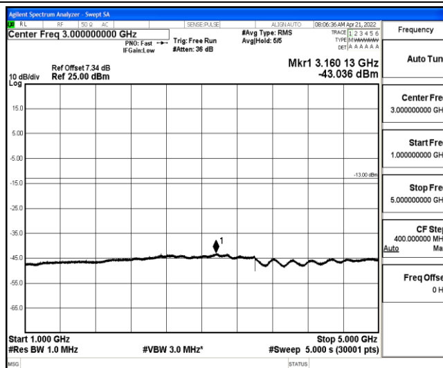
Band26-5MHz-QPSK-27015-1-0-High-1000-5000--43.04-PASS
