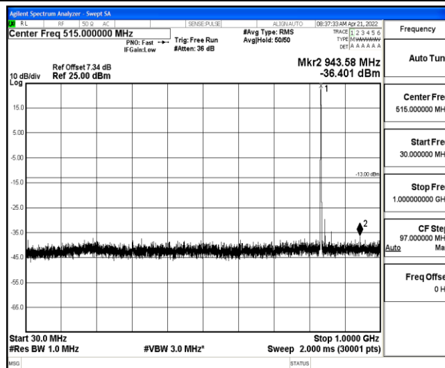
Band26-1.4MHz-16QAM-26915-1-0-Low-30-1000--36.4-PASS
