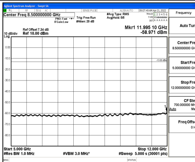
Band26-3MHz-QPSK-27025-1-0-High-5000-12000--58.97-PASS
