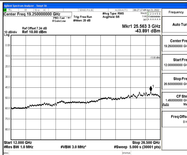
Band26-10MHz-16QAM-26915-1-0-Low-12000-26500--43.89-PASS
