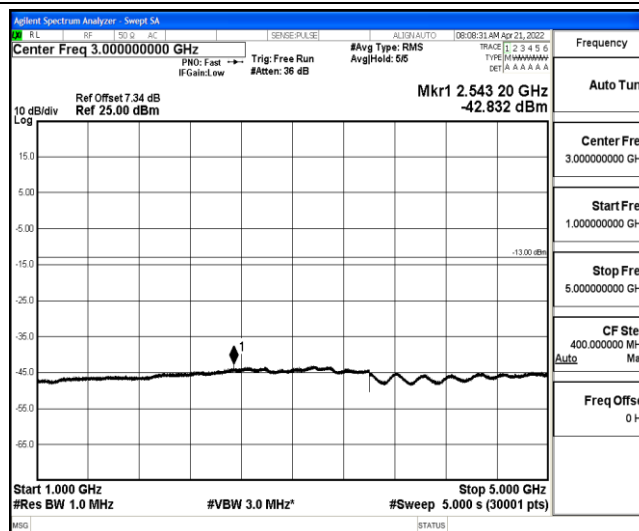
Band26-5MHz-16QAM-27015-1-0-High-1000-5000--42.83-PASS
