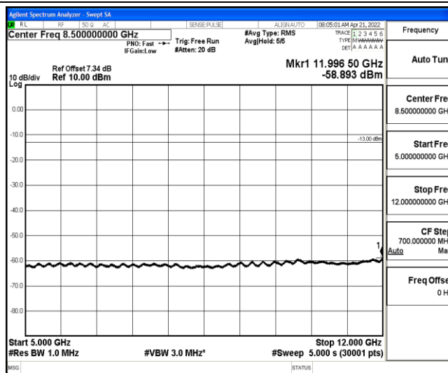
Band26-5MHz-16QAM-26915-1-0-Low-5000-12000--58.89-PASS
