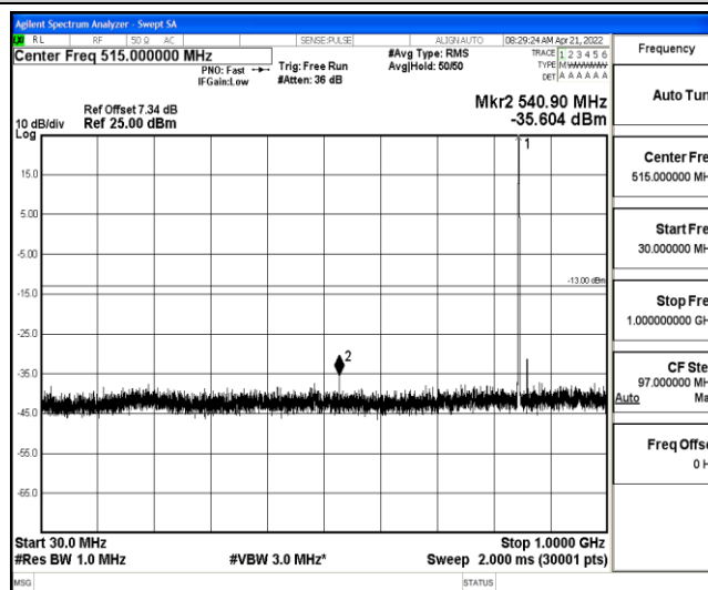
Band26-10MHz-16QAM-26990-1-0-High-30-1000--35.6-PASS
