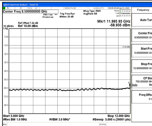
Band26-3MHz-16QAM-27025-1-0-High-5000-12000--58.94-PASS
