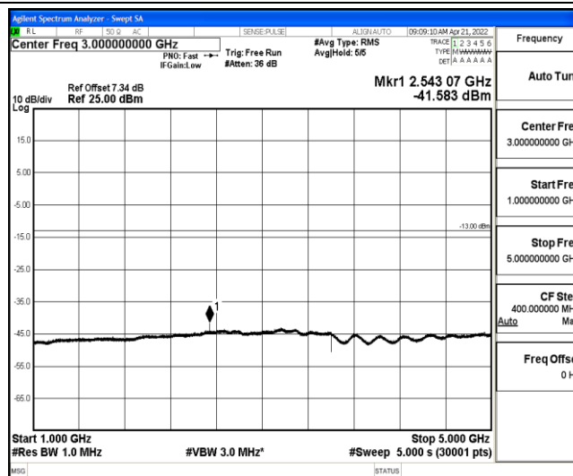
Band26-3MHz-16QAM-27025-1-0-High-1000-5000--41.58-PASS
