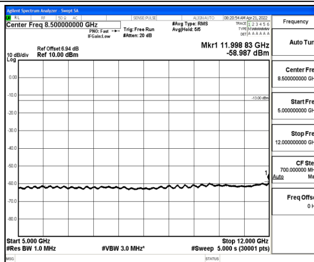
Band26-10MHz-QPSK-26840-1-0-Low-5000-12000--58.99-PASS
