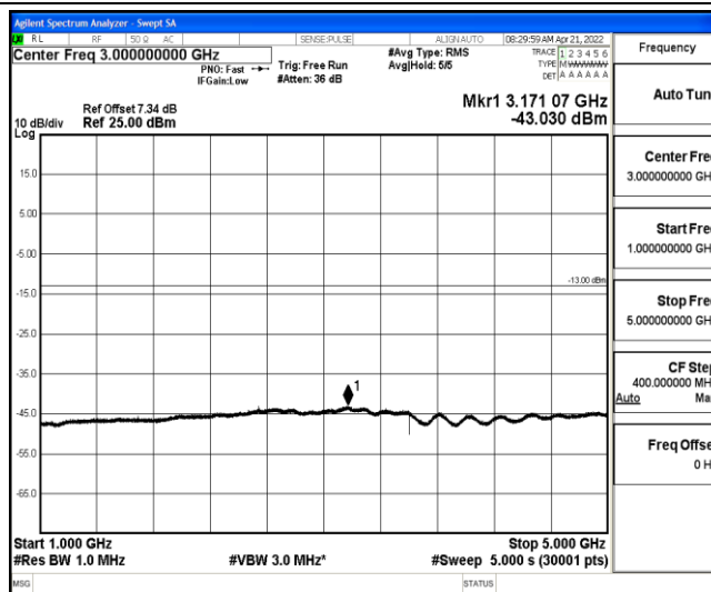
Band26-10MHz-16QAM-26990-1-0-High-1000-5000--43.03-PASS
