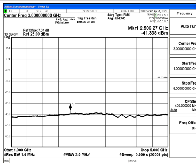
Band26-3MHz-QPSK-26915-1-0-Low-1000-5000--41.34-PASS
