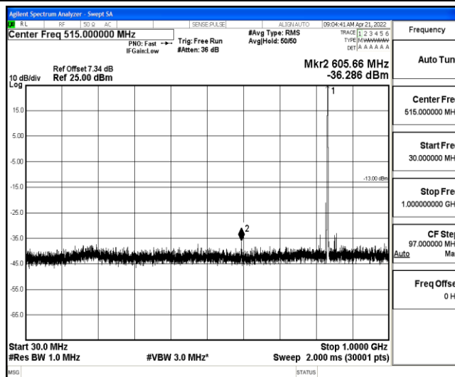
Band26-3MHz-16QAM-26915-1-0-Low-30-1000--36.29-PASS
