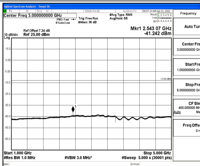
Band26-3MHz-QPSK-27025-1-0-High-1000-5000--41.24-PASS
