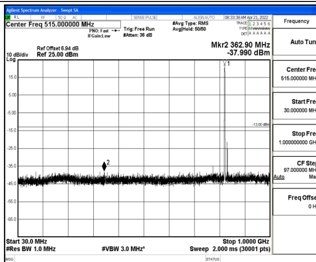
Band26-1.4MHz-16QAM-26797-1-0-Low-30-1000--37.99-PASS
