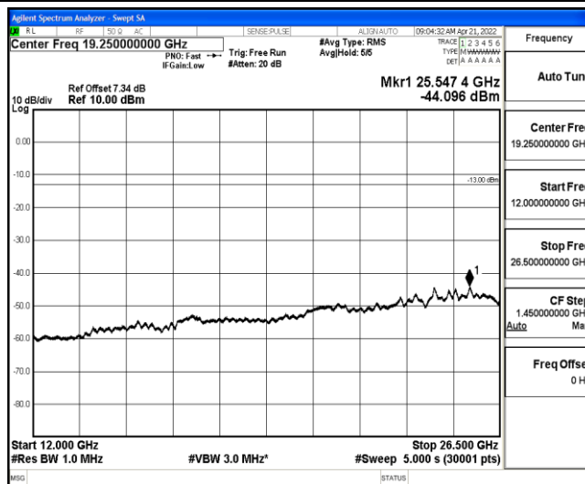
Band26-3MHz-QPSK-26915-1-0-Low-12000-26500--44.1-PASS
