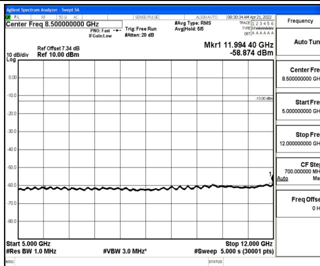
Band26-10MHz-16QAM-26990-1-0-High-5000-12000--58.87-PASS
