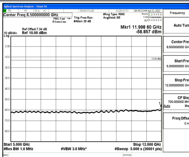
Band26-15MHz-QPSK-26865-1-0-Low-5000-12000--58.86-PASS
