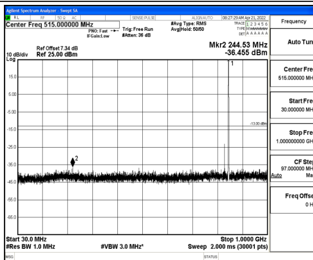
Band26-10MHz-QPSK-26990-1-0-High-30-1000--36.46-PASS
