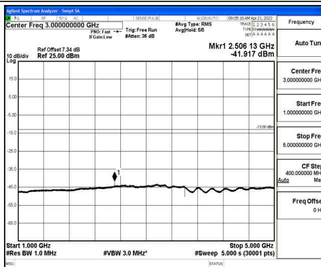
Band26-3MHz-16QAM-26915-1-0-Low-1000-5000--41.92-PASS
