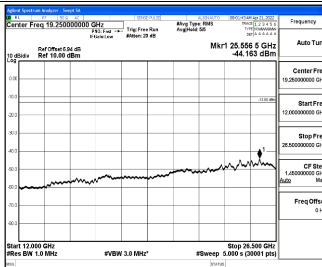
Band26-5MHz-16QAM-26815-1-0-Low-12000-26500--44.16-PASS
