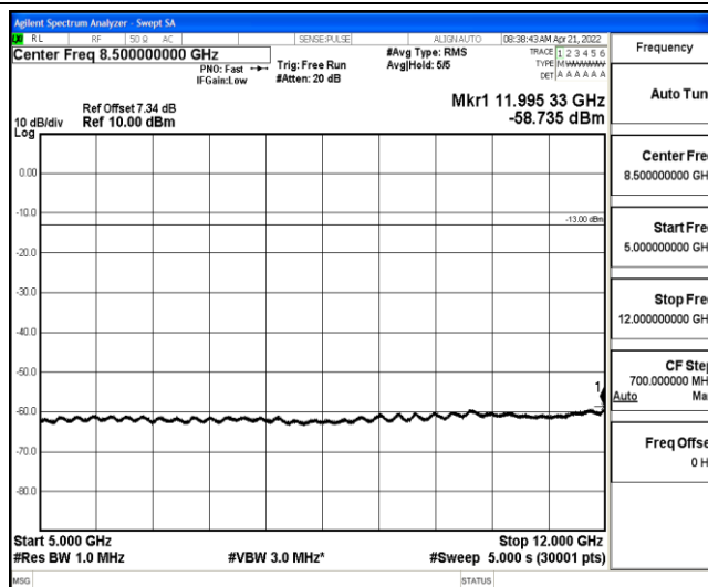
Band26-1.4MHz-16QAM-26915-1-0-Low-5000-12000--58.74-PASS
