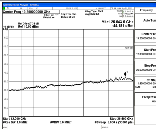
Band26-1.4MHz-16QAM-26915-1-0-Low-12000-26500--44.18-PASS
