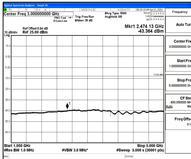
Band26-10MHz-QPSK-26840-1-0-Low-1000-5000--43.36-PASS
