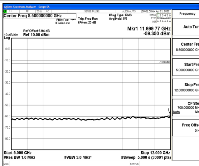
Band26-3MHz-16QAM-26805-1-0-Low-5000-12000--59.35-PASS
