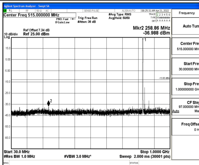
Band26-10MHz-16QAM-26915-1-0-Low-30-1000--36.99-PASS
