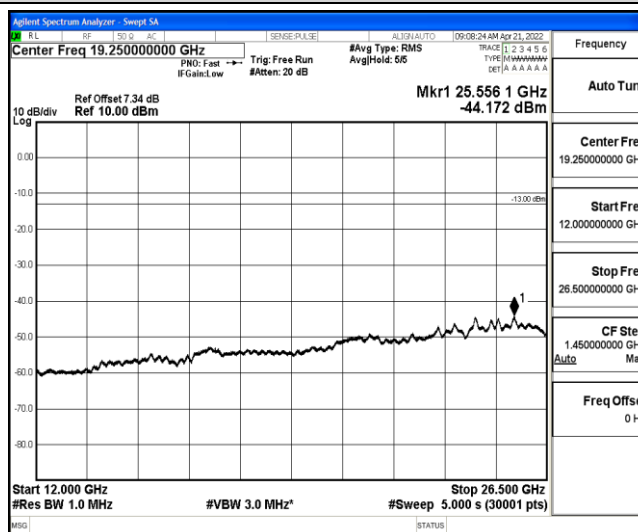
Band26-3MHz-QPSK-27025-1-0-High-12000-26500--44.17-PASS
