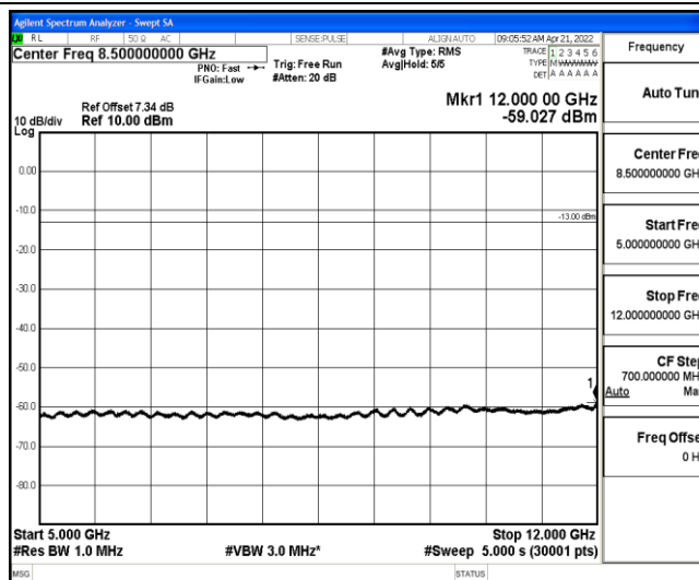
Band26-3MHz-16QAM-26915-1-0-Low-5000-12000--59.03-PASS
