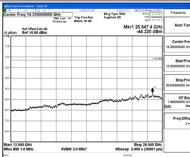
Band26-10MHz-16QAM-26840-1-0-Low-12000-26500--44.22-PASS
