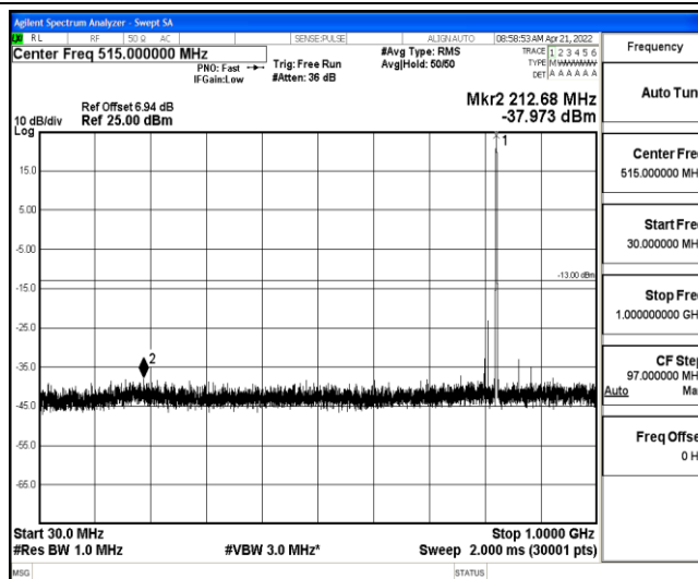
Band26-3MHz-QPSK-26805-1-0-Low-30-1000--37.97-PASS
