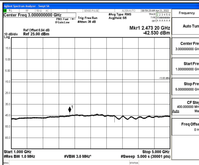
Band26-3MHz-QPSK-26805-1-0-Low-1000-5000--42.53-PASS
