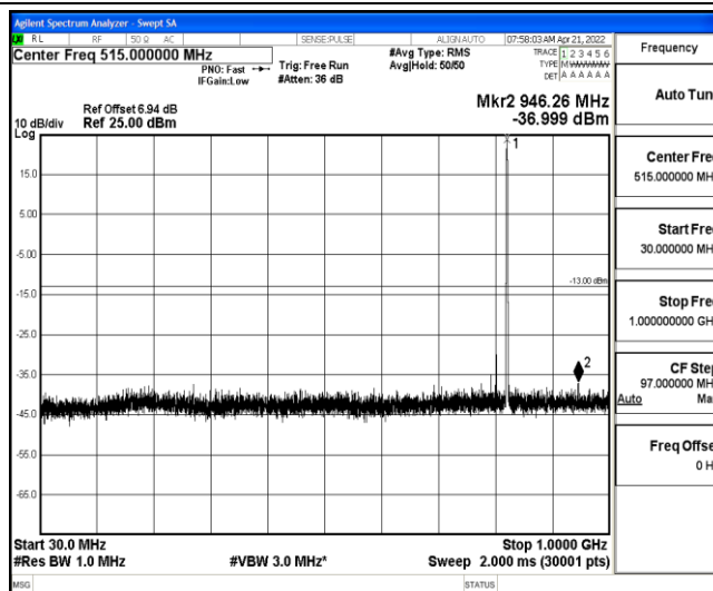
Band26-5MHz-QPSK-26815-1-0-Low-30-1000--37-PASS
