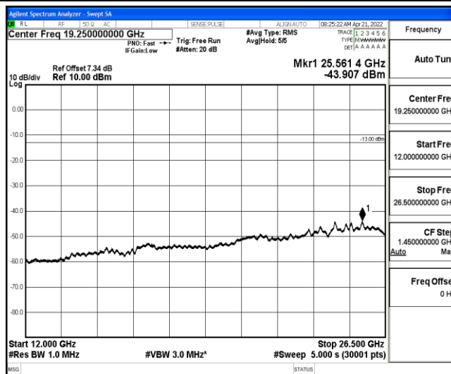
Band26-10MHz-QPSK-26915-1-0-Low-12000-26500--43.91-PASS
