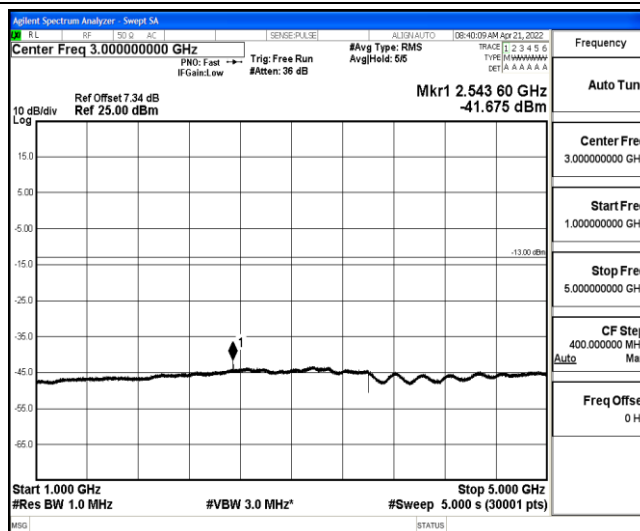
Band26-1.4MHz-QPSK-27033-1-0-High-1000-5000--41.68-PASS
