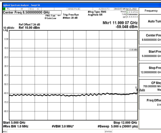
Band26-3MHz-QPSK-26915-1-0-Low-5000-12000--59.05-PASS
