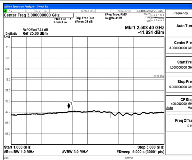
Band26-1.4MHz-16QAM-26915-1-0-Low-1000-5000--41.92-PASS
