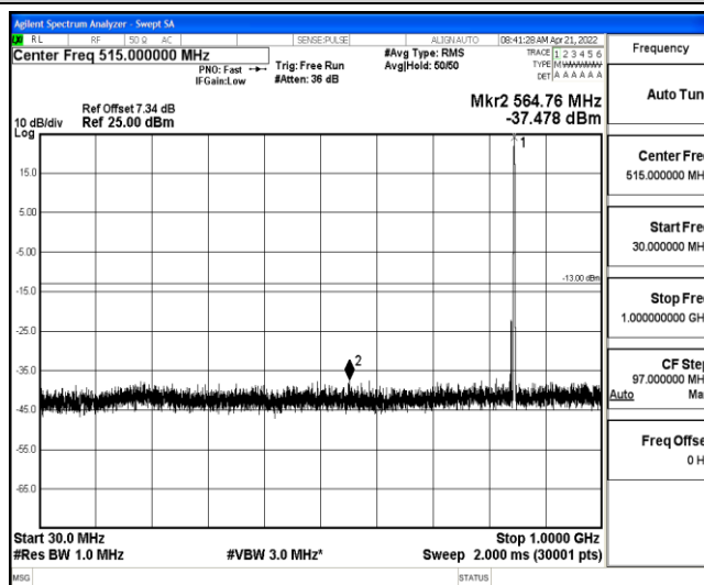
Band26-1.4MHz-16QAM-27033-1-0-High-30-1000--37.48-PASS
