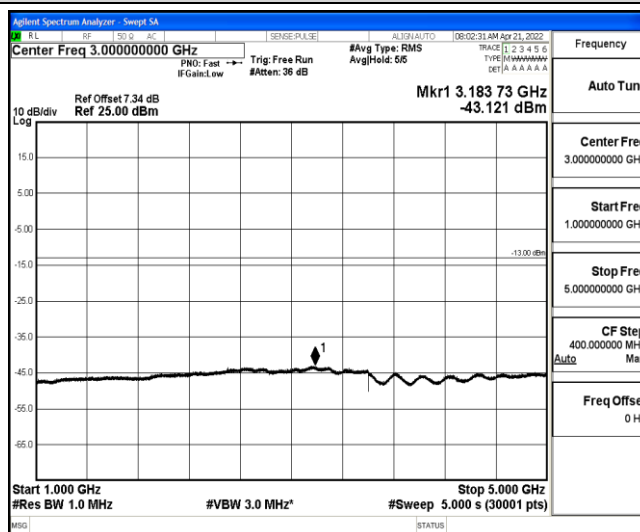
Band26-5MHz-QPSK-26915-1-0-Low-1000-5000--43.12-PASS
