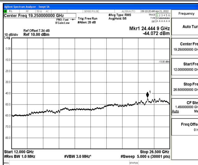
Band26-3MHz-16QAM-27025-1-0-High-12000-26500--44.07-PASS
