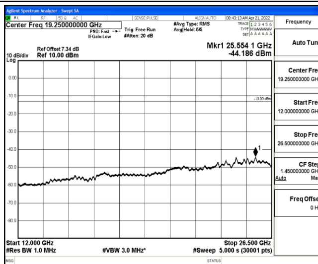
Band26-1.4MHz-16QAM-27033-1-0-High-12000-26500--44.19-PASS
