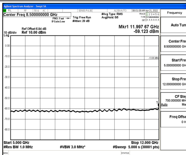
Band26-5MHz-16QAM-26815-1-0-Low-5000-12000--59.12-PASS
