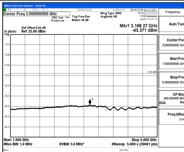
Band26-5MHz-16QAM-26815-1-0-Low-1000-5000--43.37-PASS
