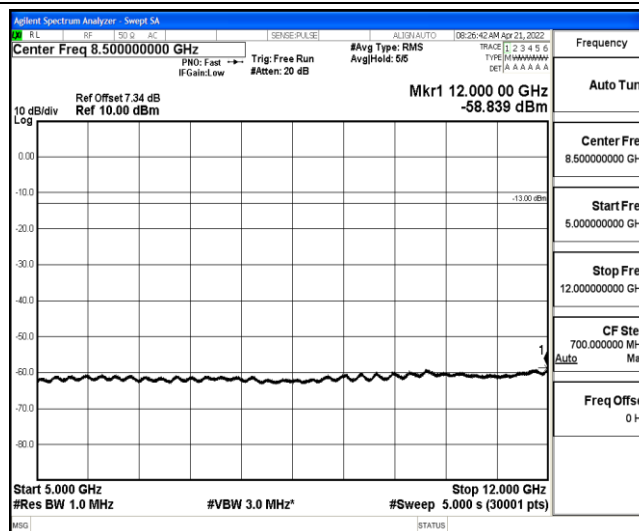
Band26-10MHz-16QAM-26915-1-0-Low-5000-12000--58.84-PASS
