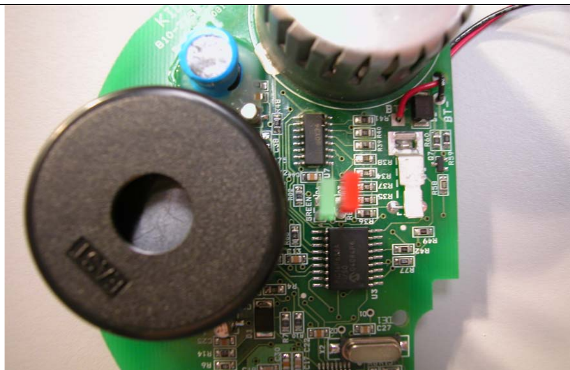
PCB 2 Front Component
