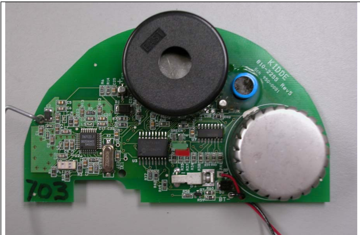
Whole Top PCB
