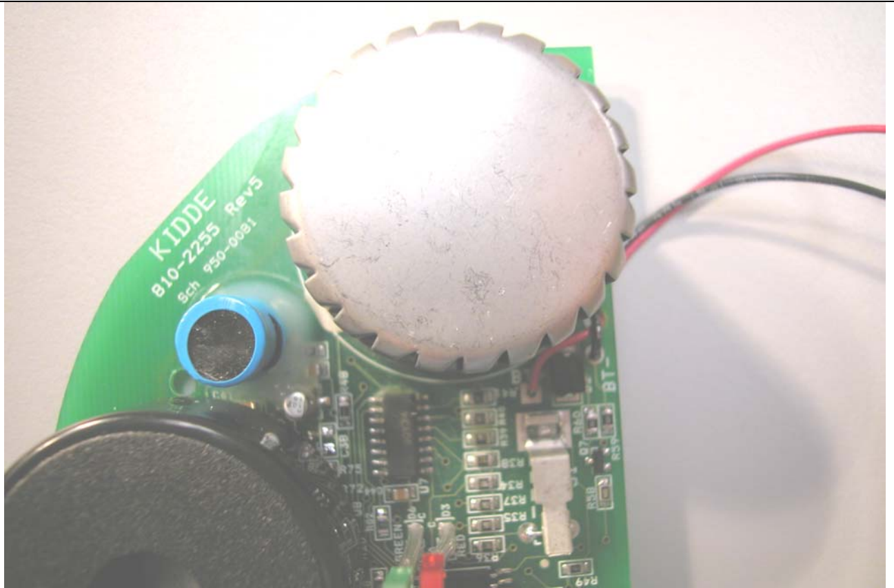
PCB 3 Front Component
