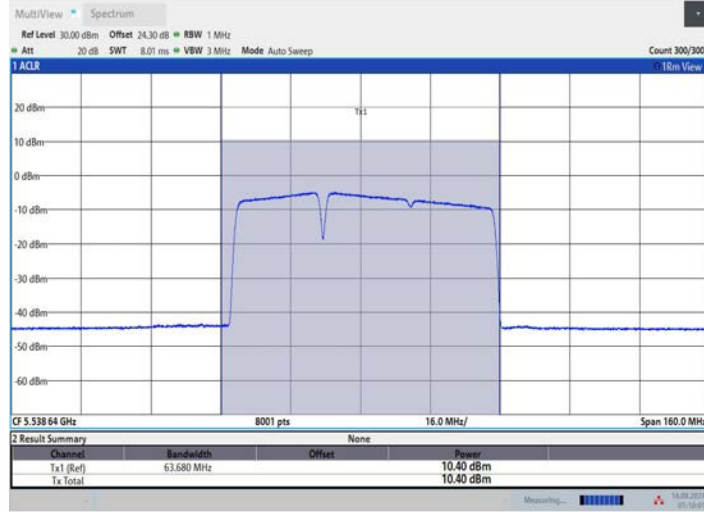
11BE80MIMO_Ant3_5530_484+242_OFDMA_1
