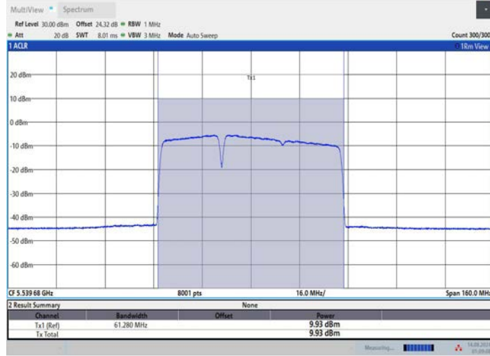
11BE80MIMO_Ant1_5530_484+242_OFDMA_1
