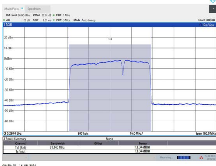
11BE80MIMO_Ant3_5290_484+242_OFDMA_1
