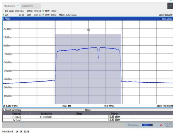
11BE80MIMO_Ant2_5290_484+242_OFDMA_1
