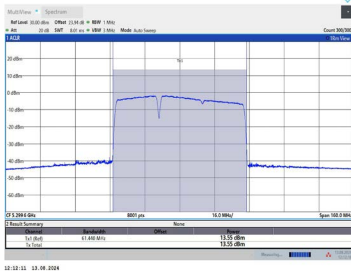
11BE80MIMO_Ant1_5290_484+242_OFDMA_2
