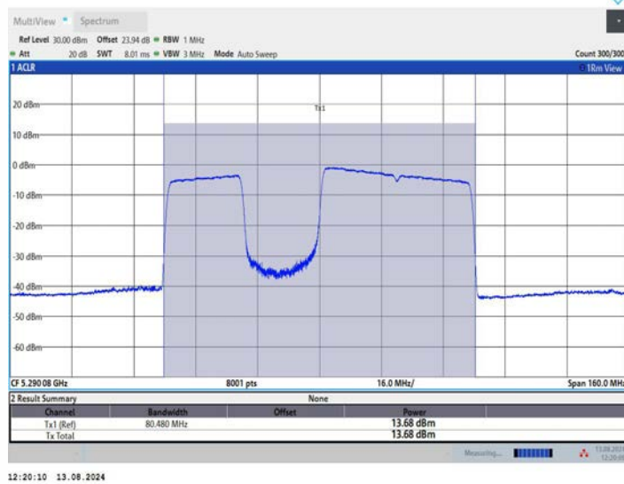
11BE80MIMO_Ant1_5290_484+242_OFDMA_3
