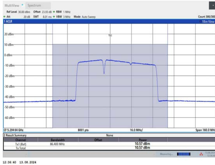
11BE80MIMO_Ant3_5290_484+242_OFDMA_1
