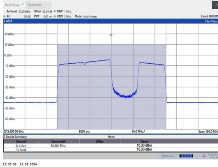
11BE80MIMO_Ant1_5290_484+242_OFDMA_3
