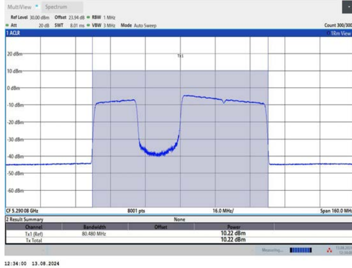
11BE80MIMO_Ant1_5290_484+242_OFDMA_2
