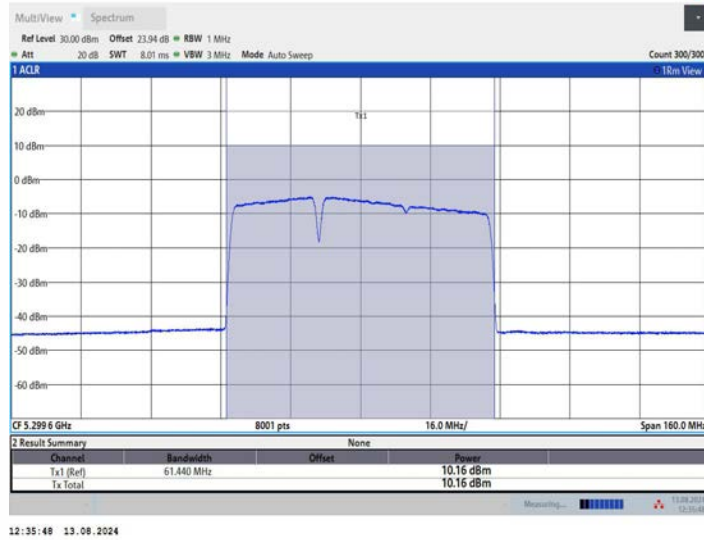
11BE80MIMO_Ant1_5290_484+242_OFDMA_1
