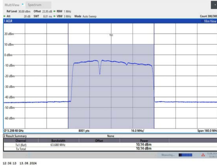
11BE80MIMO_Ant2_5290_484+242_OFDMA_1
