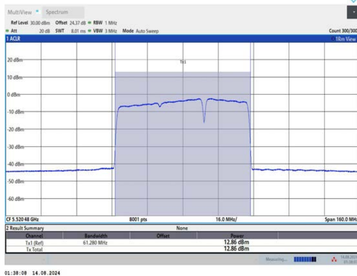
11BE80MIMO_Ant3_5530_484+242_OFDMA_1
