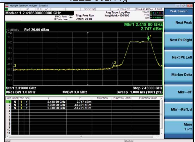
Channel 1 / 2412 MHz – Peak
