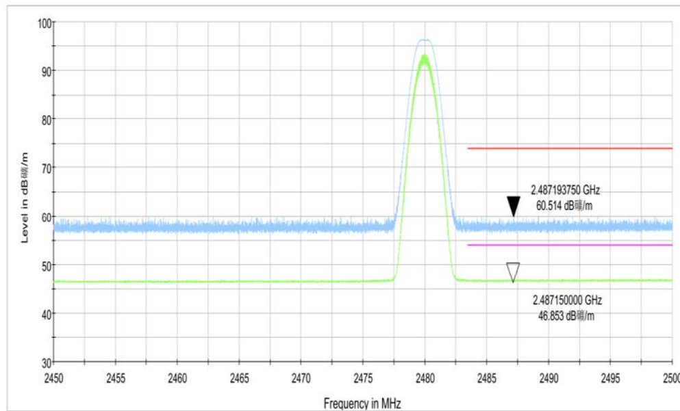
Fig.4. Frequency Band Edges: GFSK, 2480 MHz, 2.45 GHz - 2.50GHz
