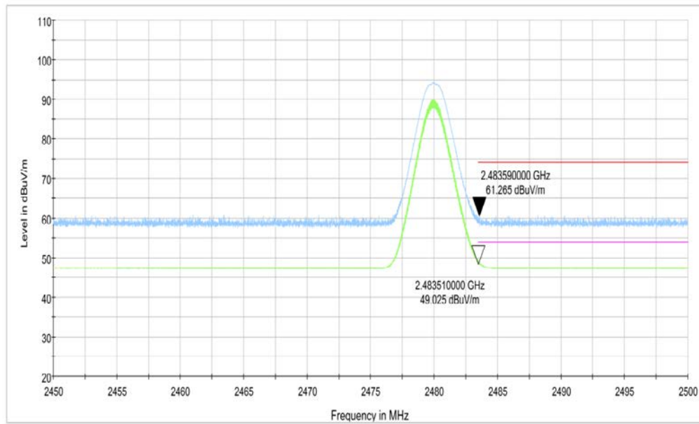
Fig.2. Frequency Band Edges: GFSK, 2480 MHz, 2.45 GHz - 2.50GHz
