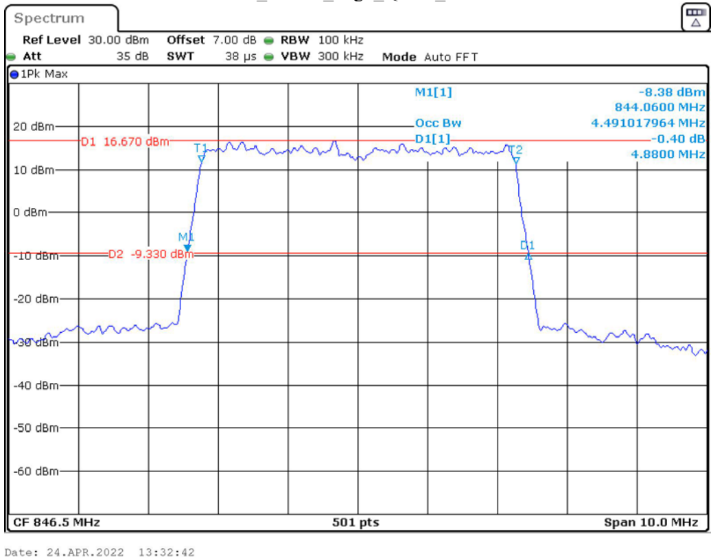
Band 5_5 MHz_High_QPSK_RB25#0
