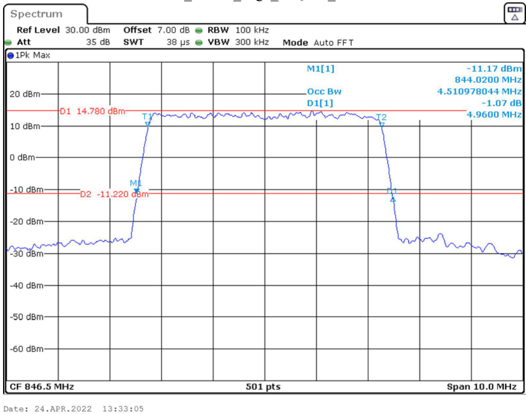
Band 5_5 MHz_High_16QAM_RB25#0
