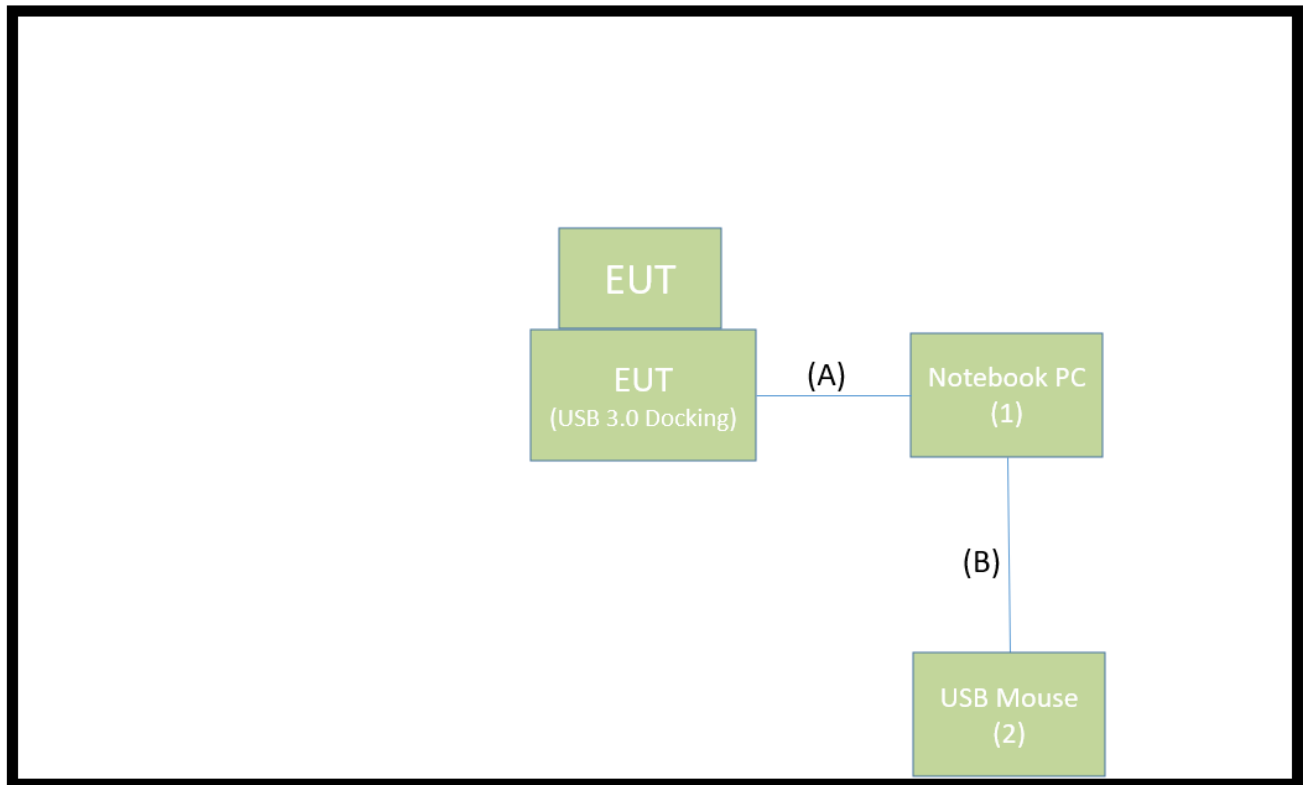
Connection Diagram
