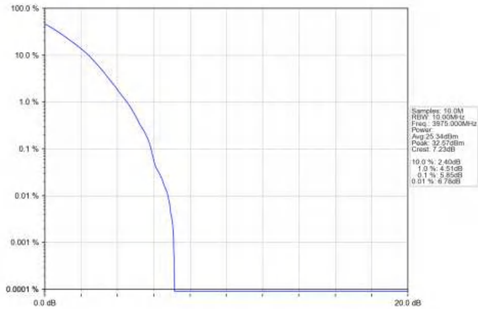
n77a_15kHz_SISO_NTNV_10MHz_DFT-s-OFDM_QPSK_3975MHz_Outer_Full_Ant1
