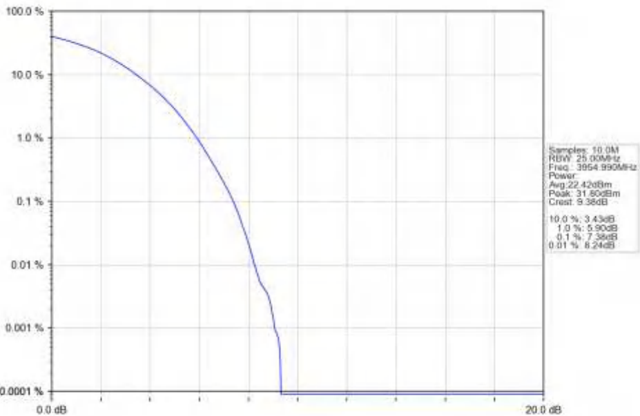
n77a_15kHz_SISO_NTNV_50MHz_DFT-s-OFDM_16_QAM_3954.99MHz_Outer_Full_Ant1
