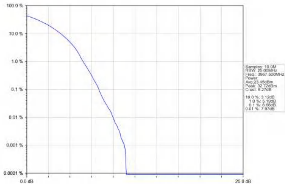
n77a_30kHz_SISO_NTNV_25MHz_DFT-s-OFDM_256_QAM_3967.5MHz_Outer_Full_Ant1
