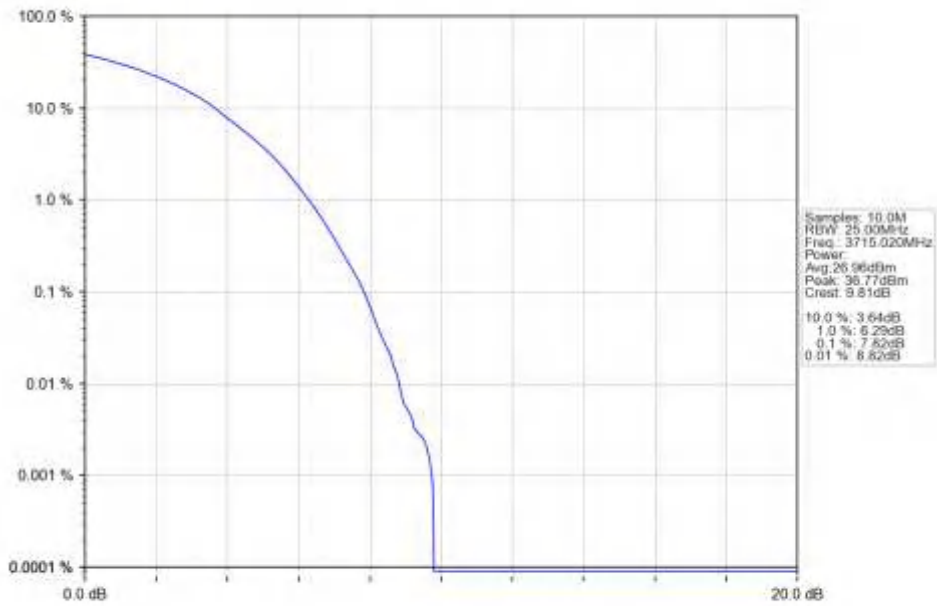
n77a_30kHz_SISO_NTNV_30MHz_CP-OFDM_QPSK_3715.02MHz_Outer_Full_Ant1
