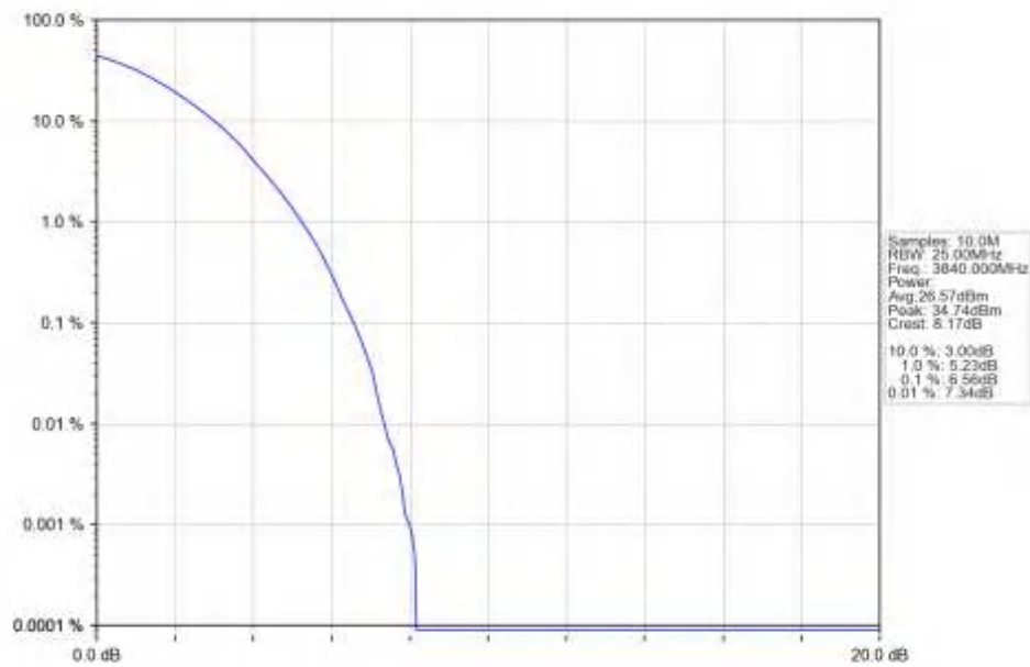
n77a_30kHz_SISO_NTNV_30MHz_DFT-s-OFDM_64_QAM_3840MHz_Outer_Full_Ant1
