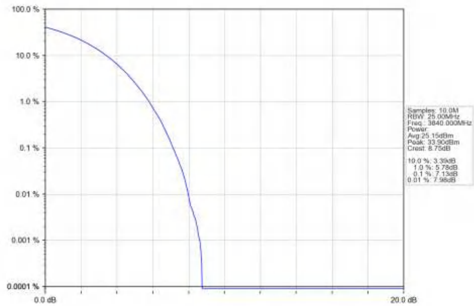
n77a_30kHz_SISO_NTNV_40MHz_DFT-s-OFDM_16_QAM_3840MHz_Outer_Full_Ant1
