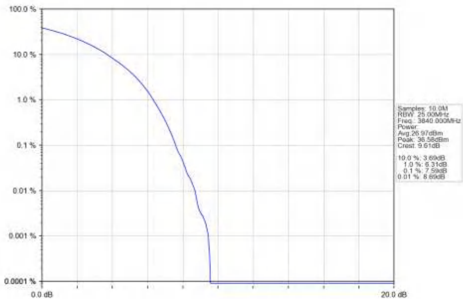
n77a_30kHz_SISO_NTNV_25MHz_CP-OFDM_16_QAM_3840MHz_Outer_Full_Ant1
