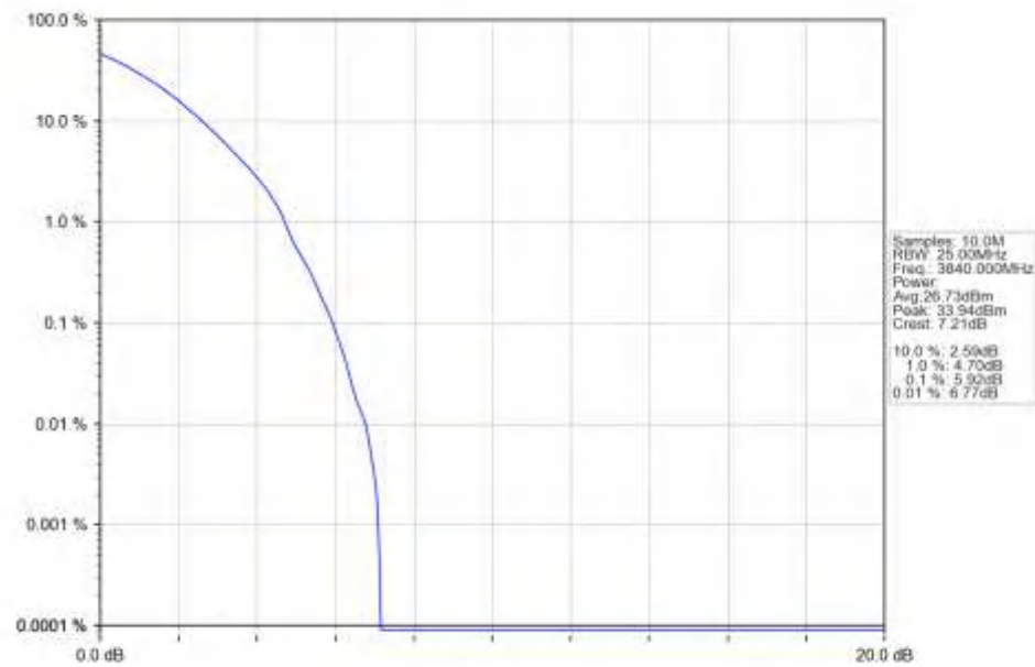
n77a_30kHz_SISO_NTNV_15MHz_DFT-s-OFDM_QPSK_3840MHz_Outer_Full_Ant1
