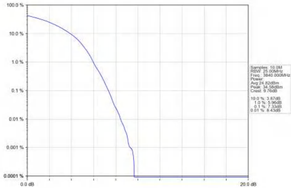
n77a_30kHz_SISO_NTNV_25MHz_DFT-s-OFDM_256_QAM_3840MHz_Outer_Full_Ant1
