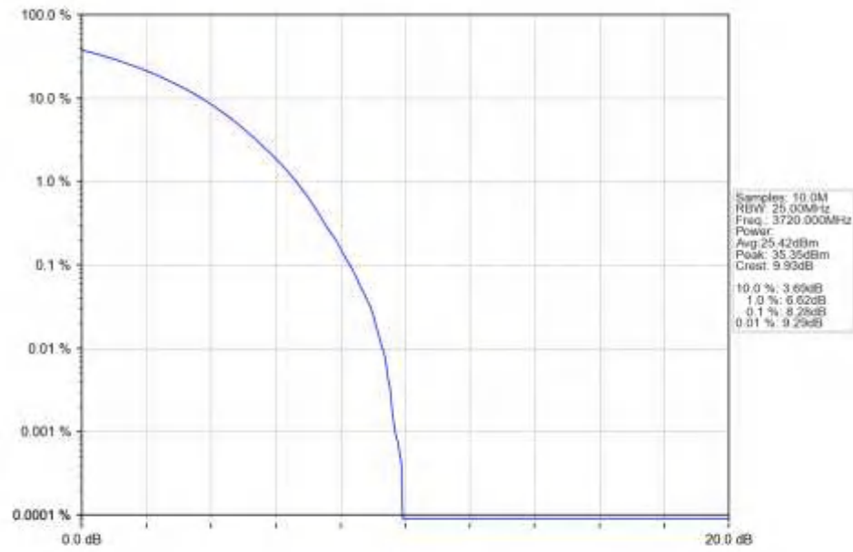
n77a 30kHz SISO_NTNV_40MHz CP-OFDM QPSK_3720MHz_Outer_Full_Ant1
