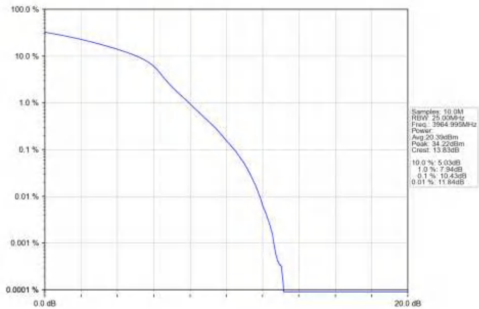
n77a_15kHz_SISO_NTNV_30MHz_CP-OFDM_256_QAM_3964.995MHz_Outer_Full_Ant1
