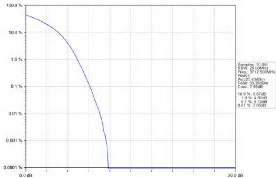
n77a_15kHz_SISO_NTNV_25MHz_DFT-s-OFDM_16_QAM_3712.5MHz_Outer_Full_Ant1
