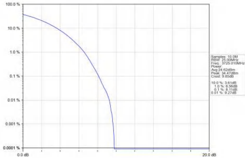
n77a_15kHz_SISO_NTNV_50MHz_CP-OFDM_QPSK_3725.01MHz_Outer_Full_Ant1
