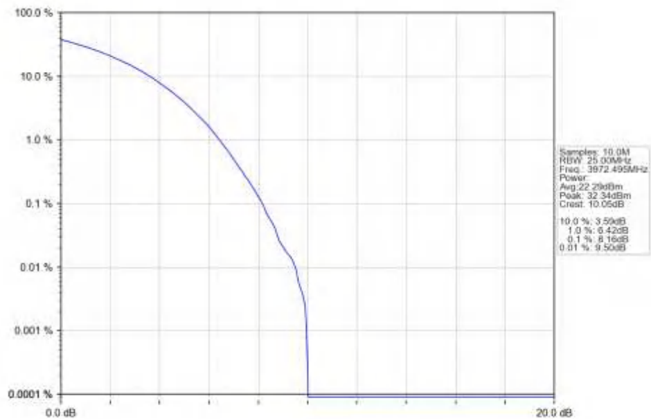
n77a_15kHz_SISO_NTNV_15MHz_CP-OFDM_256_QAM_3972.495MHz_Outer_Full_Ant1
