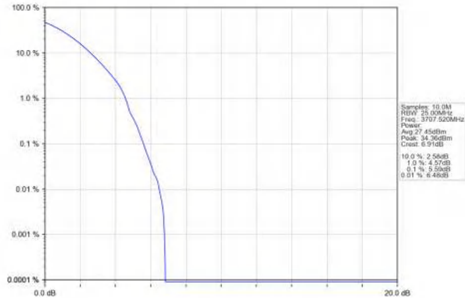
n77a_30kHz_SISO_NTNV_15MHz_DFT-s-OFDM_QPSK_3707.52MHz_Outer_Full_Ant1
