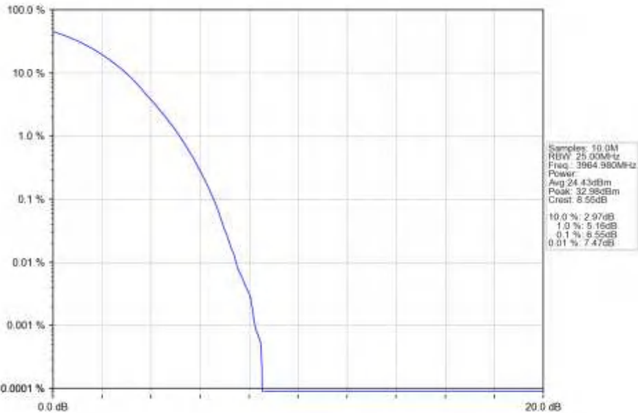
n77a_30kHz_SISO_NTNV_30MHz_DFT-s-OFDM_16_QAM_3964.98MHz_Outer_Full_Ant1
