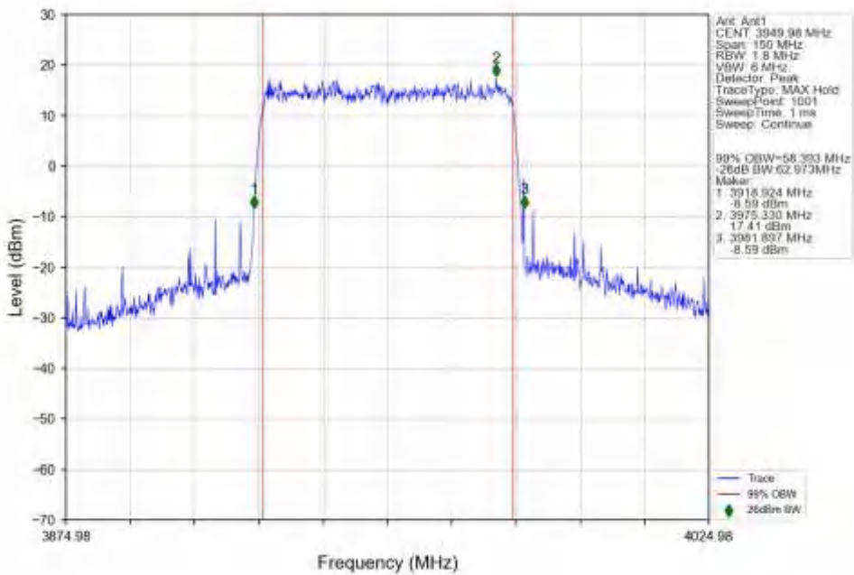
n77a_30kHz_SISO_NTNV_60MHz_CP-OFDM_256_QAM_3949.98MHz_Outer_Full_Ant1
