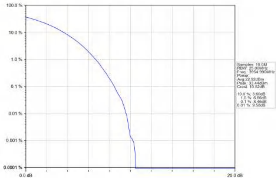
n77a_15kHz_SISO_NTNV_50MHz_CP-OFDM_16_QAM_3954.99MHz_Outer_Full_Ant1
