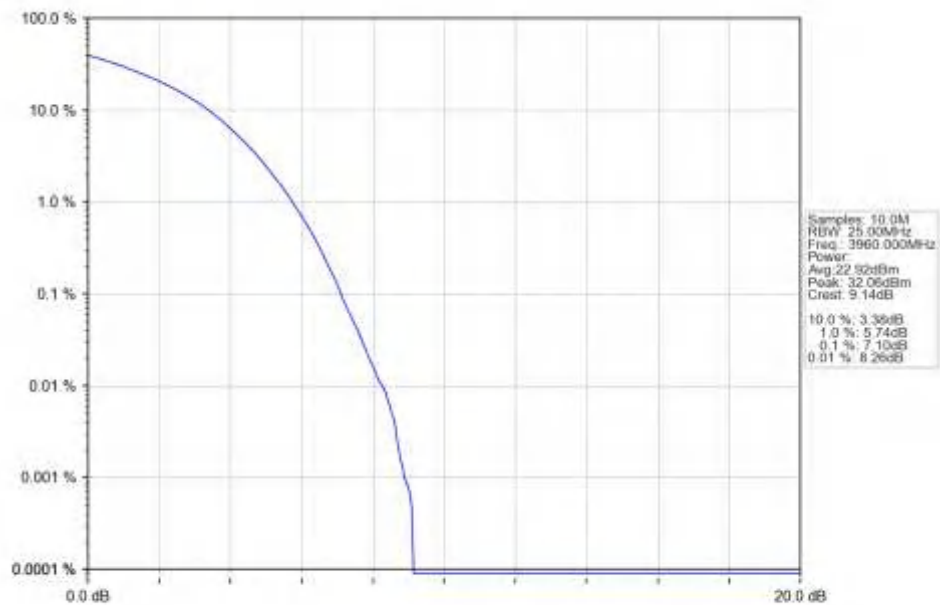
n77a_15kHz_SISO_NTNV_40MHz_DFT-s-OFDM_16_QAM_3960MHz_Outer_Full_Ant1
