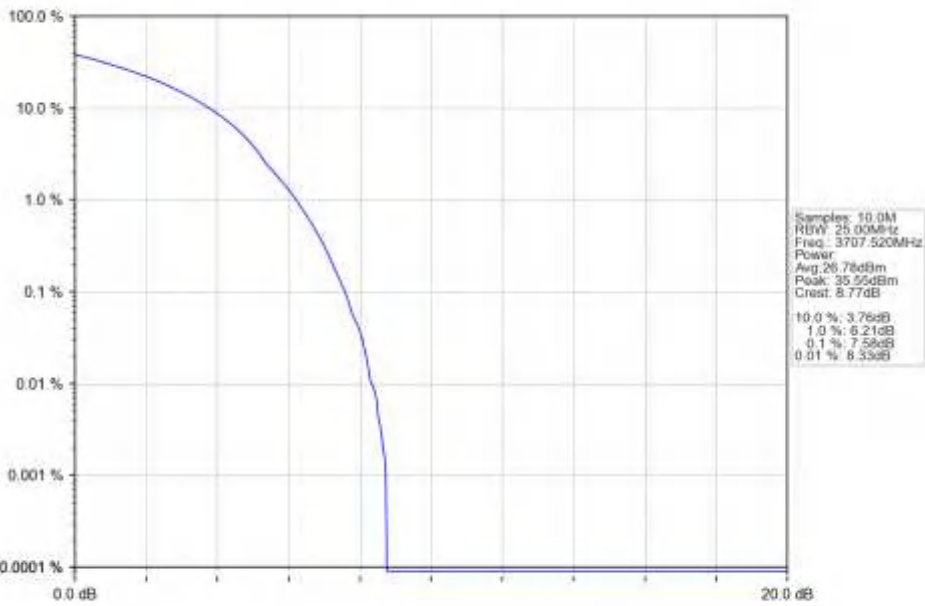
n77a_30kHz_SISO_NTNV_15MHz_CP-OFDM_64_QAM_3707.52MHz_Outer_Full_Ant1
