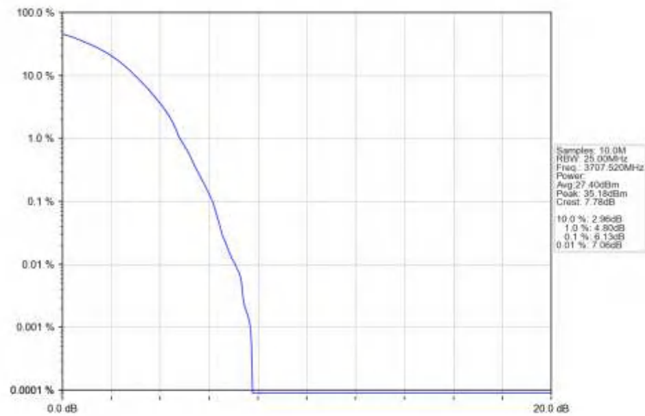
n77a_30kHz_SISO_NTNV_15MHz_DFT-s-OFDM_16_QAM_3707.52MHz_Outer_Full_Ant1
