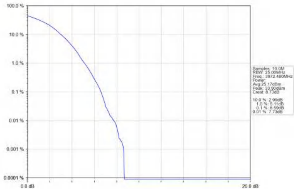
n77a 30kHz SISO NTN 15MHz DFT-s-OFDM 16 QAM 3972.48MHz Outer Full Ant1
