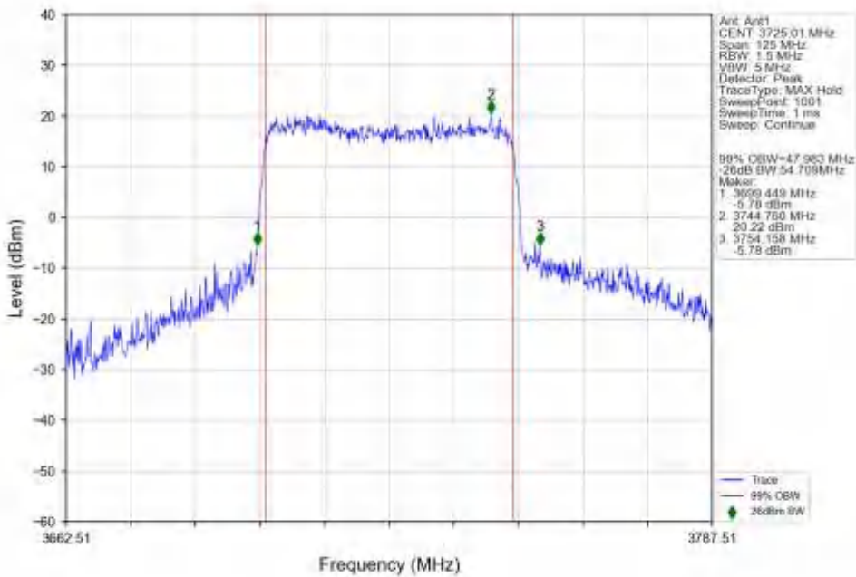
n77a_30kHz_SISO_NTNV_50MHz_CP-OFDM_16_QAM_3725.01MHz_Outer_Full_Ant1
