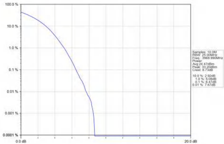
n77a_15kHz_SISO_NTNV_20MHz_DFT-s-OFDM_256_QAM_3969.99MHz_Outer_Full_Ant1
