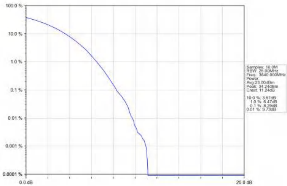
n77a_15kHz_SISO_NTNV_25MHz_CP-OFDM_256_QAM_3840MHz_Outer_Full_Ant1
