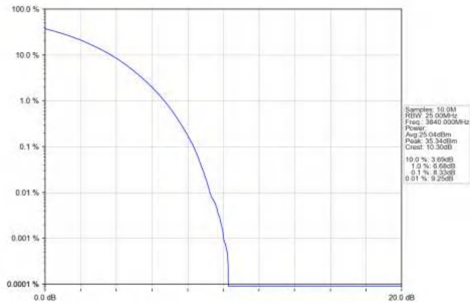
n77a 30kHz SISO_NTNV_40MHz CP-OFDM QPSK_3840MHz_Outer_Full_Ant1
