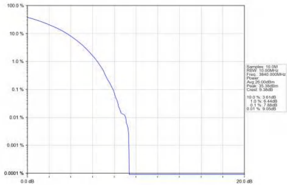
n77a_15kHz_SISO_NTNV_10MHz_CP-OFDM_16_QAM_3840MHz_Outer_Full_Ant1
