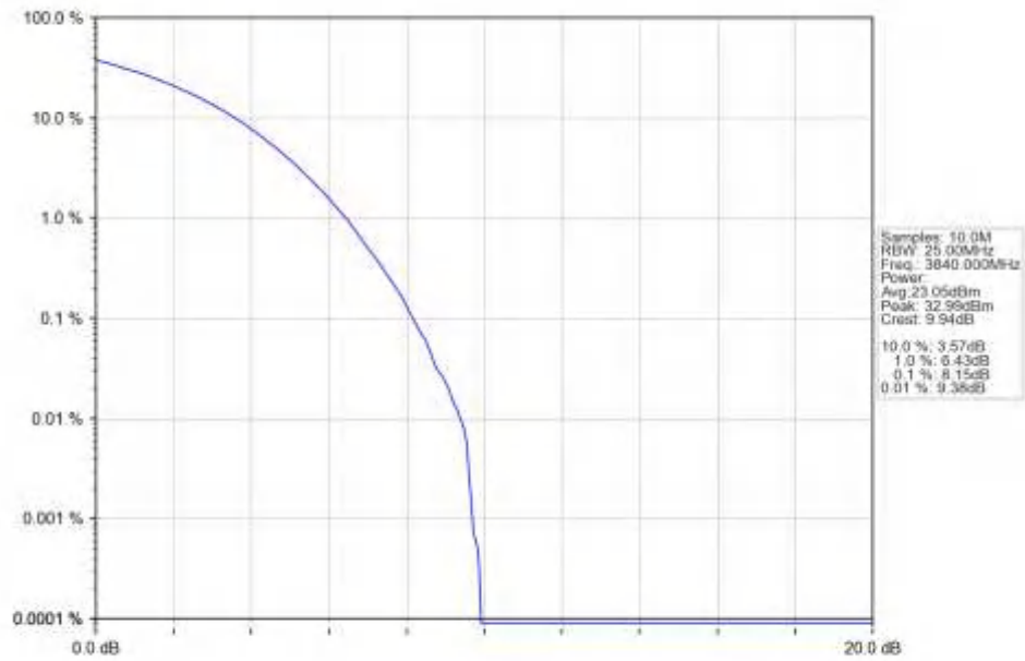
n77a_15kHz_SISO_NTNV_15MHz_CP-OFDM_256_QAM_3840MHz_Outer_Full_Ant1
