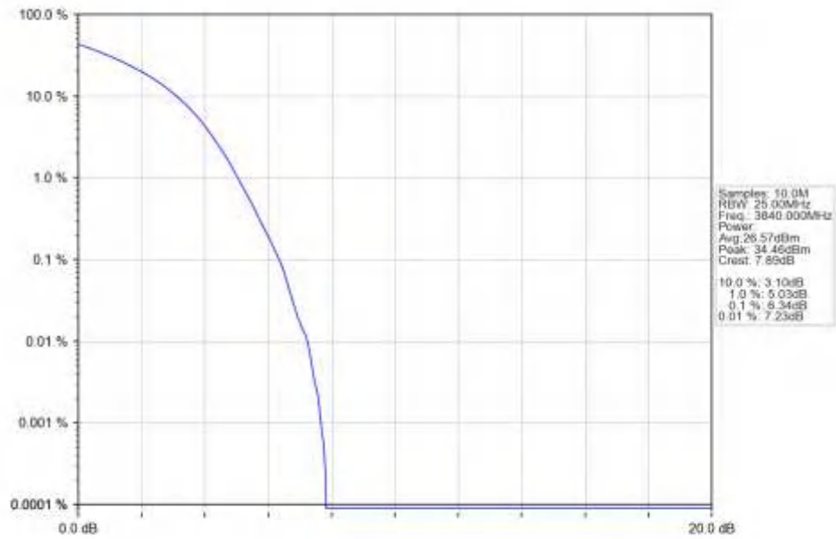
n77a_15kHz_SISO_NTNV_25MHz_DFT-s-OFDM_16_QAM_3840MHz_Outer_Full_Ant1
