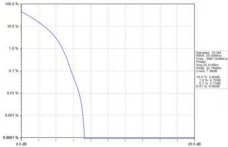
n77a_15kHz_SISO_NTNV_25MHz_DFT-s-OFDM_QPSK_3967.5MHz_Outer_Full_Ant1
