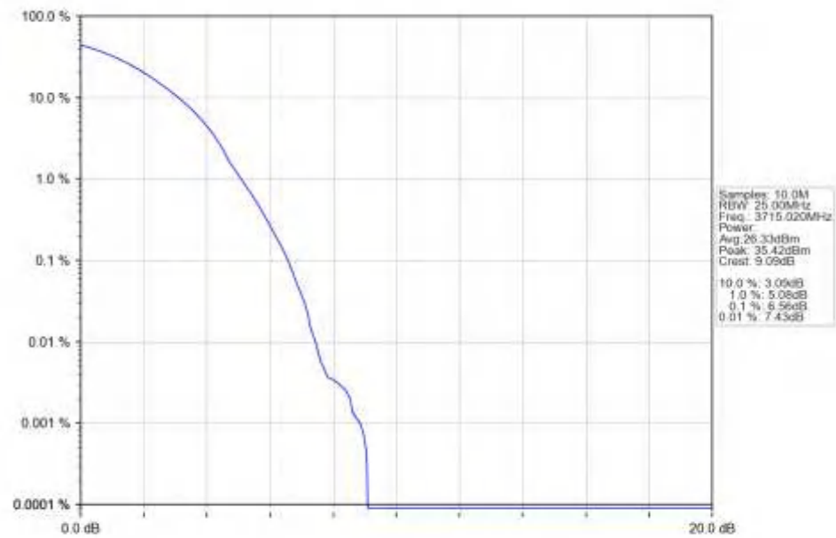
n77a_30kHz_SISO_NTNV_30MHz_DFT-s-OFDM_256_QAM_3715.02MHz_Outer_Full_Ant1
