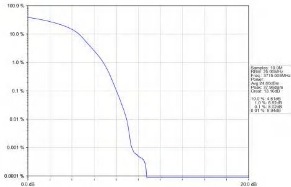
n77a_15kHz_SISO_NTNV_30MHz_DFT-s-OFDM_256_QAM_3715.005MHz_Outer_Full_Ant1
