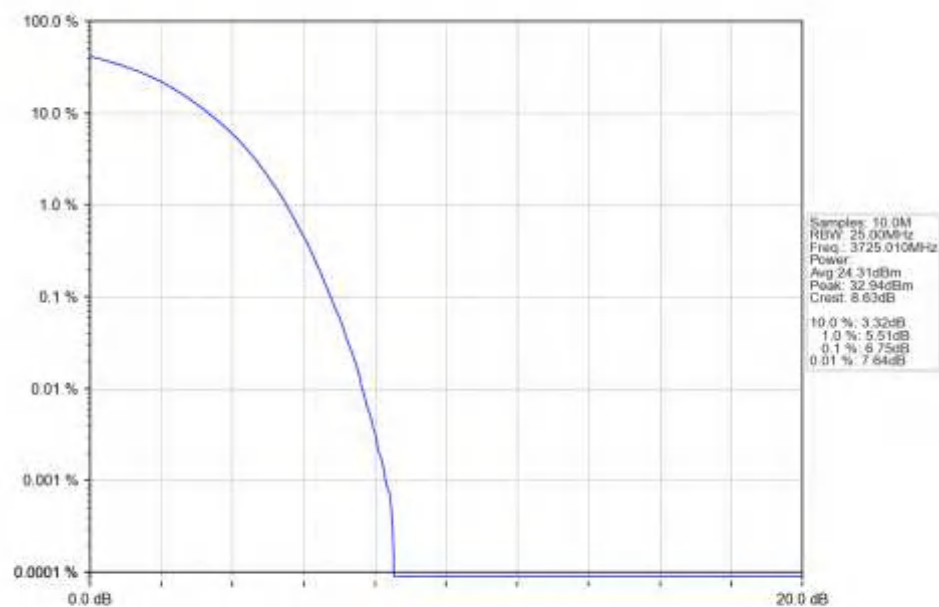
n77a_15kHz_SISO_NTNV_50MHz_DFT-s-OFDM QPSK_3725.01MHz_Outer_Full_Ant1
