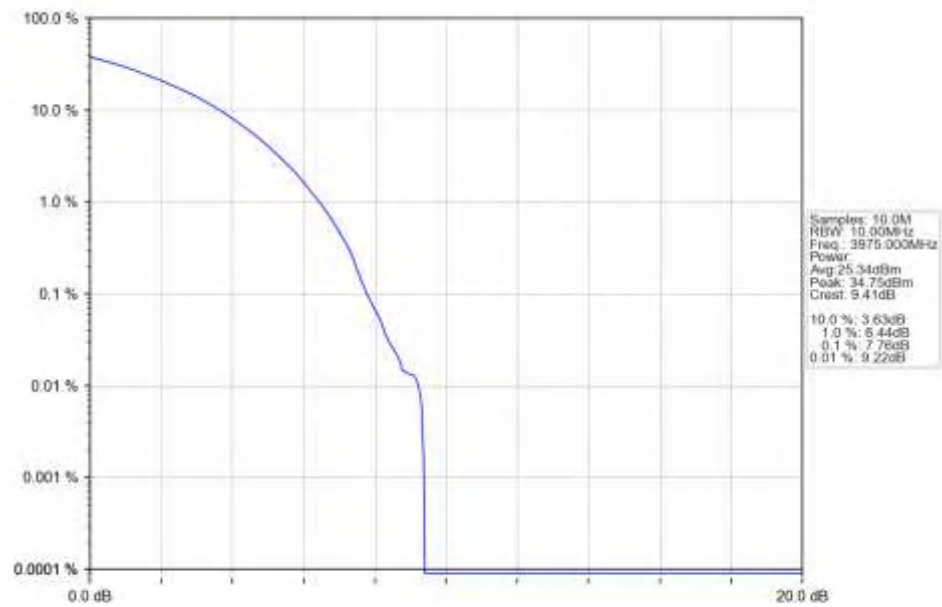
n77a_15kHz_SISO_NTNV_10MHz_CP-OFDM_16_QAM_3975MHz_Outer_Full_Ant1
