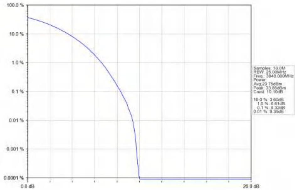
n77a_15kHz_SISO_NTNV_50MHz_CP-OFDM_16_QAM_3840MHz_Outer_Full_Ant1
