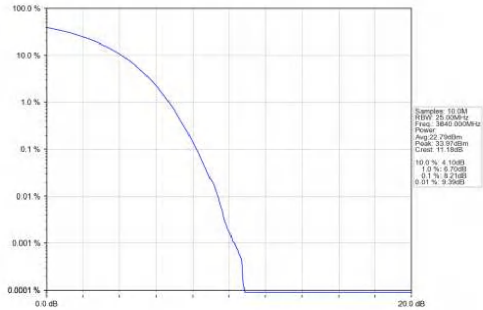
n77a_30kHz_SISO_NTNV_40MHz_DFT-s-OFDM_256_QAM_3840MHz_Outer_Full_Ant1
