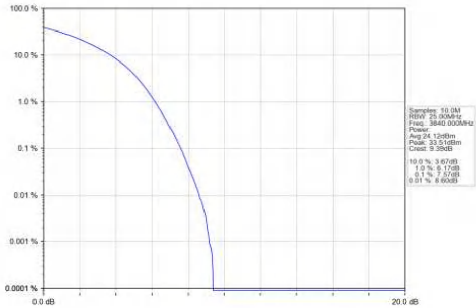
n77a_30kHz_SISO_NTNV_50MHz_DFT-s-OFDM_16_QAM_3840MHz_Outer_Full_Ant1
