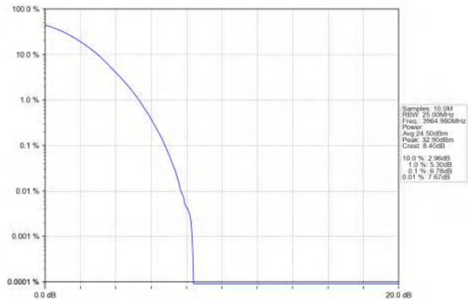
n77a_30kHz_SISO_NTNV_30MHz_DFT-s-OFDM_64_QAM_3964.98MHz_Outer_Full_Ant1
