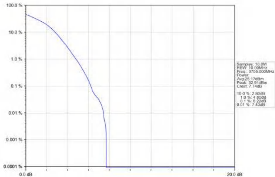
n77a_15kHz_SISO_NTNV_10MHz_DFT-s-OFDM_16_QAM_3705MHz_Outer_Full_Ant1
