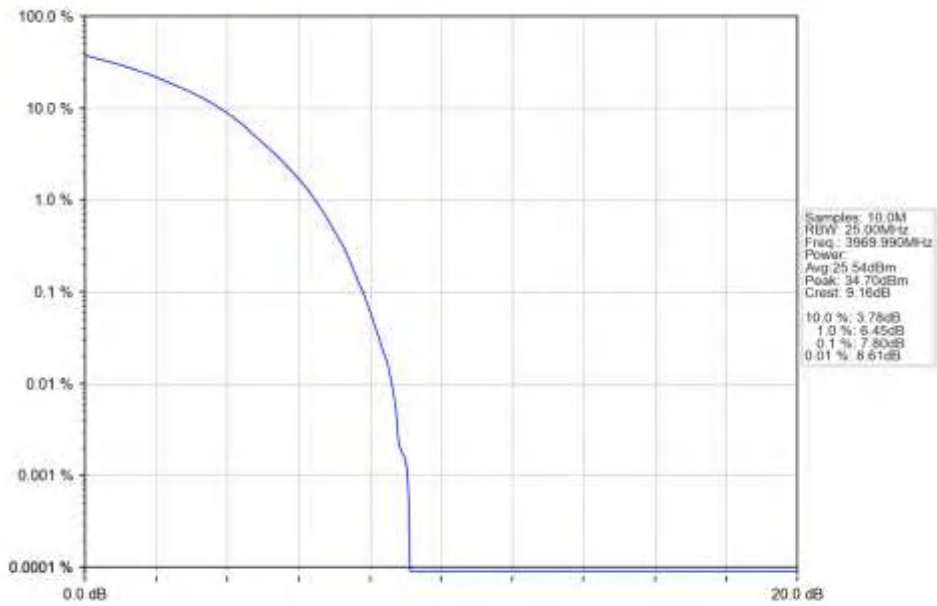
n77a_30kHz_SISO_NTNV_20MHz_CP-OFDM_QPSK_3969.99MHz_Outer_Full_Ant1
