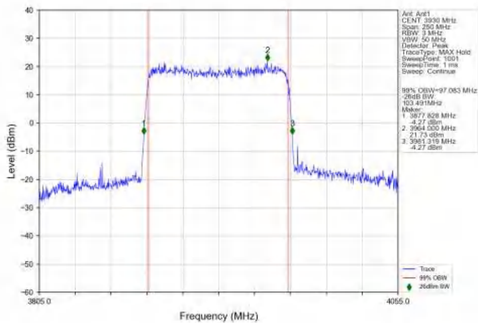
n77a_30kHz_SISO_NTNV_100MHz_DFT-s-OFDM_16_QAM_3930MHz_Outer_Full_Ant1
