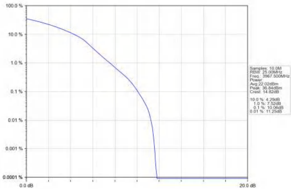
n77a_15kHz_SISO_NTNV_25MHz_CP-OFDM_256_QAM_3967.5MHz_Outer_Full_Ant1
