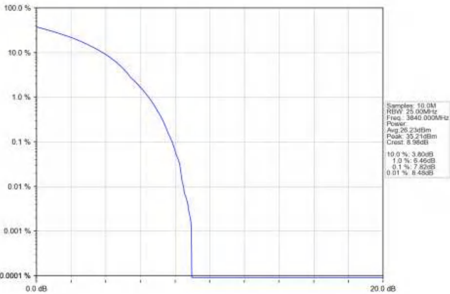
n77a_30kHz_SISO_NTNV_15MHz_CP-OFDM_64_QAM_3840MHz_Outer_Full_Ant1
