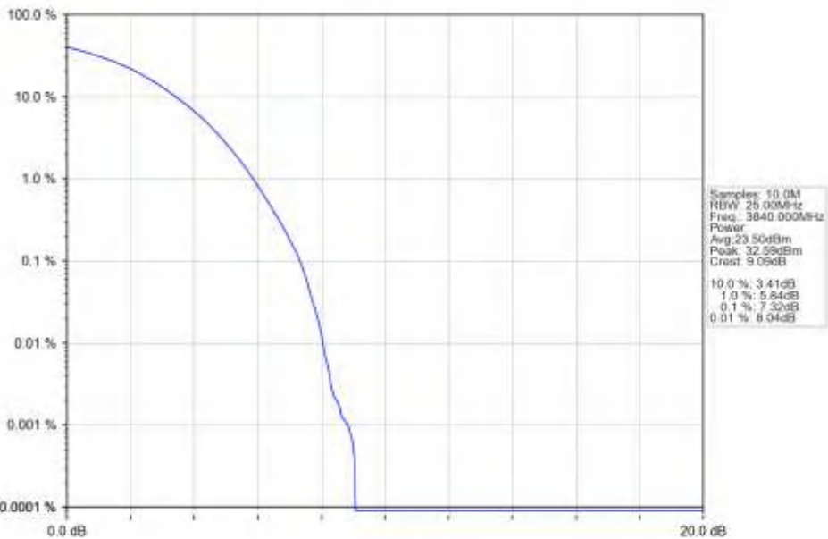
n77a_15kHz_SISO_NTNV_50MHz_DFT-s-OFDM_16_QAM_3840MHz_Outer_Full_Ant1
