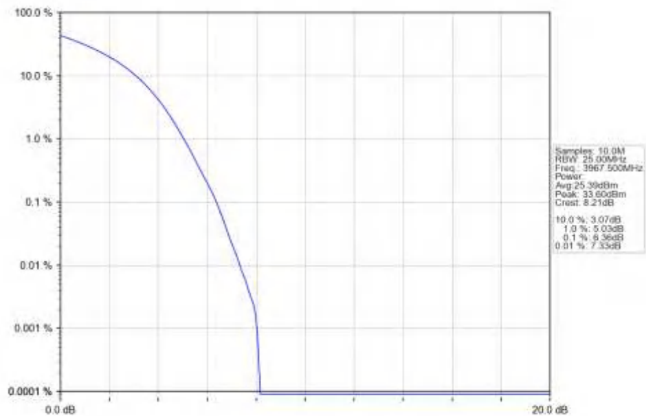
n77a_15kHz_SISO_NTNV_25MHz_DFT-s-OFDM_16_QAM_3967.5MHz_Outer_Full_Ant1
