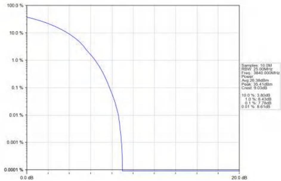
n77a_30kHz_SISO_NTNV_20MHz_CP-OFDM_64_QAM_3840MHz_Outer_Full_Ant1
