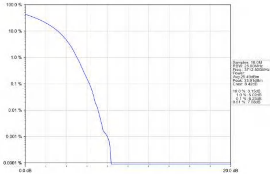
n77a_15kHz_SISO_NTNV_25MHz_DFT-s-OFDM_64_QAM_3712.5MHz_Outer_Full_Ant1
