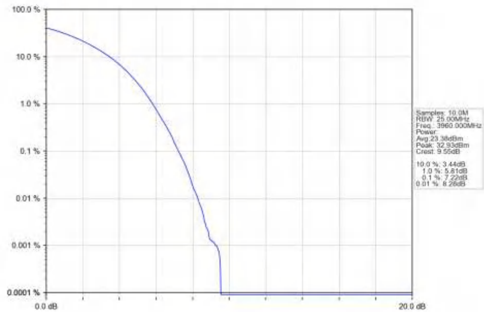
n77a_30kHz_SISO_NTNV_40MHz_DFT-s-OFDM_16_QAM_3960MHz_Outer_Full_Ant1
