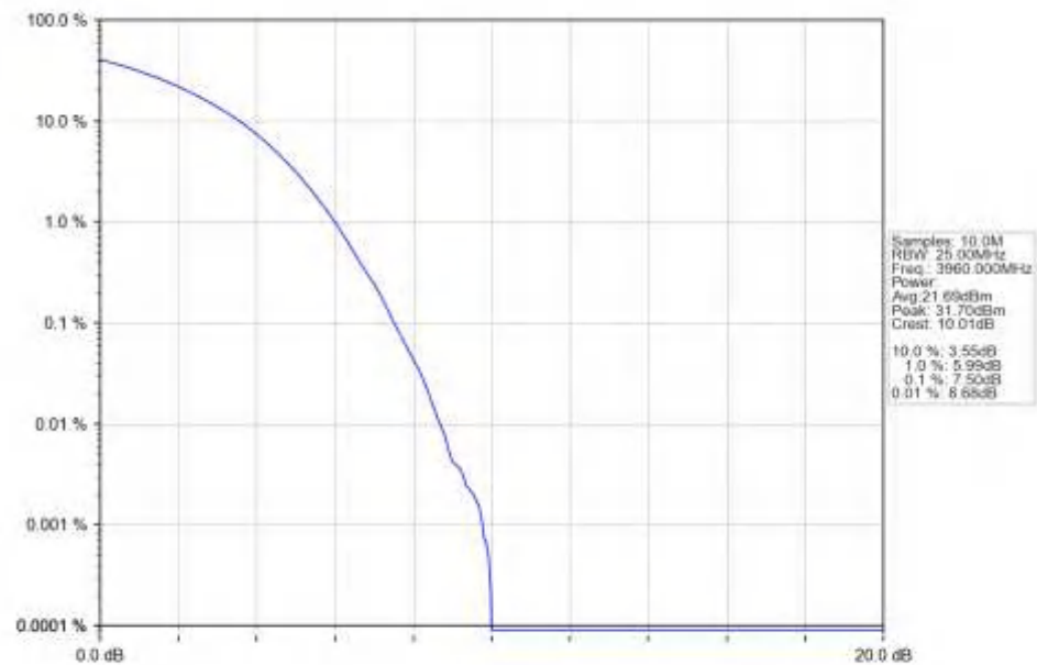
n77a_30kHz_SISO_NTNV_40MHz_DFT-s-OFDM_256_QAM_3960MHz_Outer_Full_Ant1
