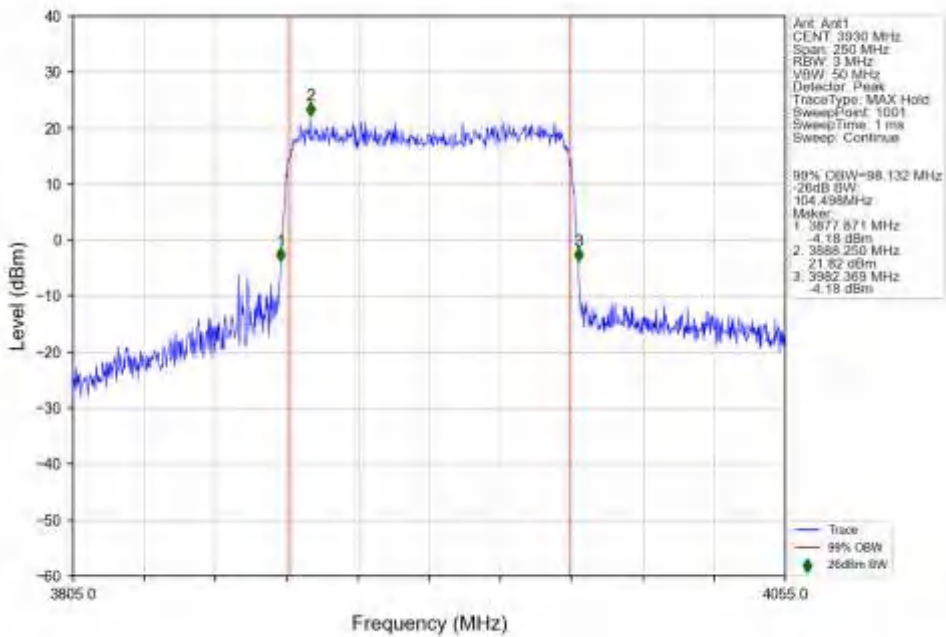
n77a_30kHz_SISO_NTNV_100MHz_CP-OFDM_16_QAM_3930MHz_Outer_Full_Ant1
