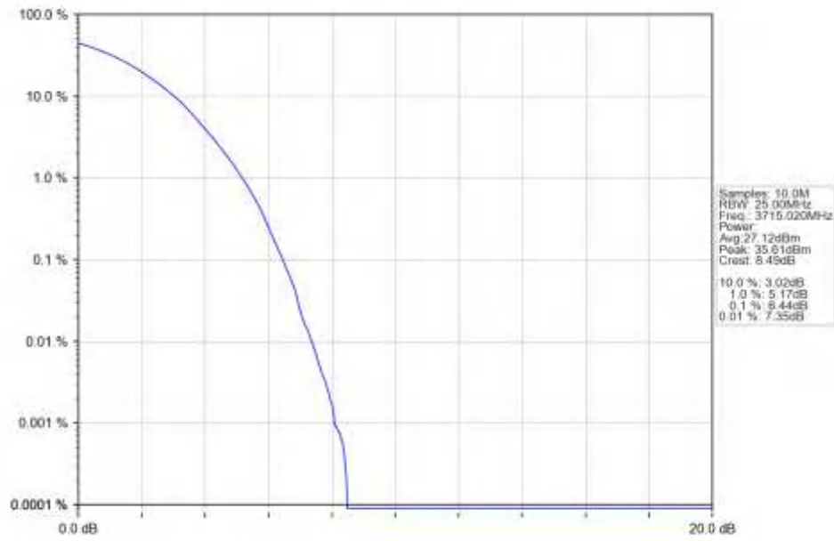
n77a_30kHz_SISO_NTNV_30MHz_DFT-s-OFDM_64_QAM_3715.02MHz_Outer_Full_Ant1
