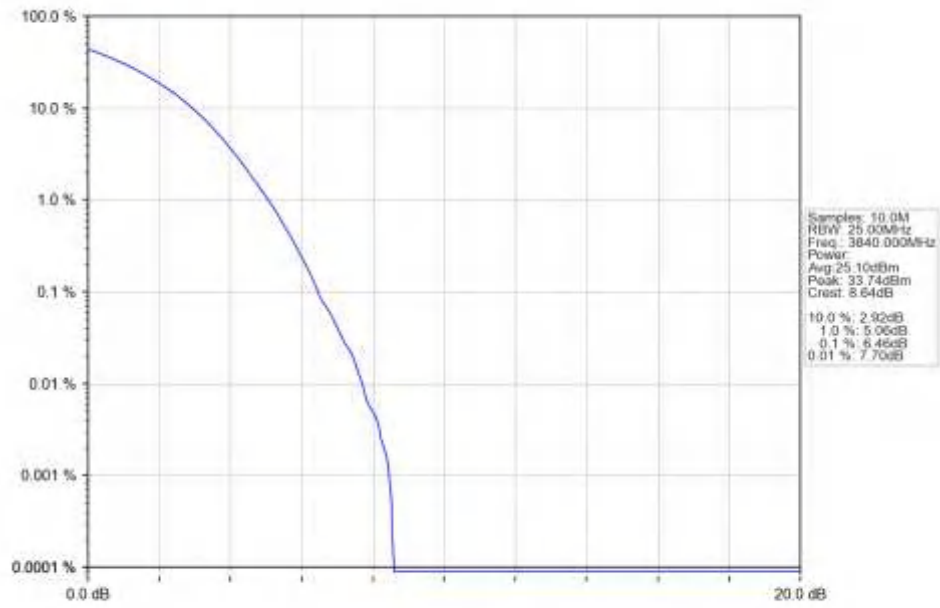
n77a_15kHz_SISO_NTNV_20MHz_DFT-s-OFDM_256_QAM_3840MHz_Outer_Full_Ant1
