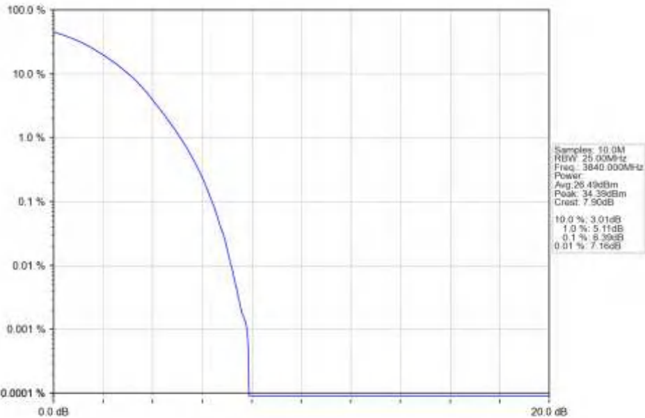
n77a_30kHz_SISO_NTNV_30MHz_DFT-s-OFDM_16_QAM_3840MHz_Outer_Full_Ant1
