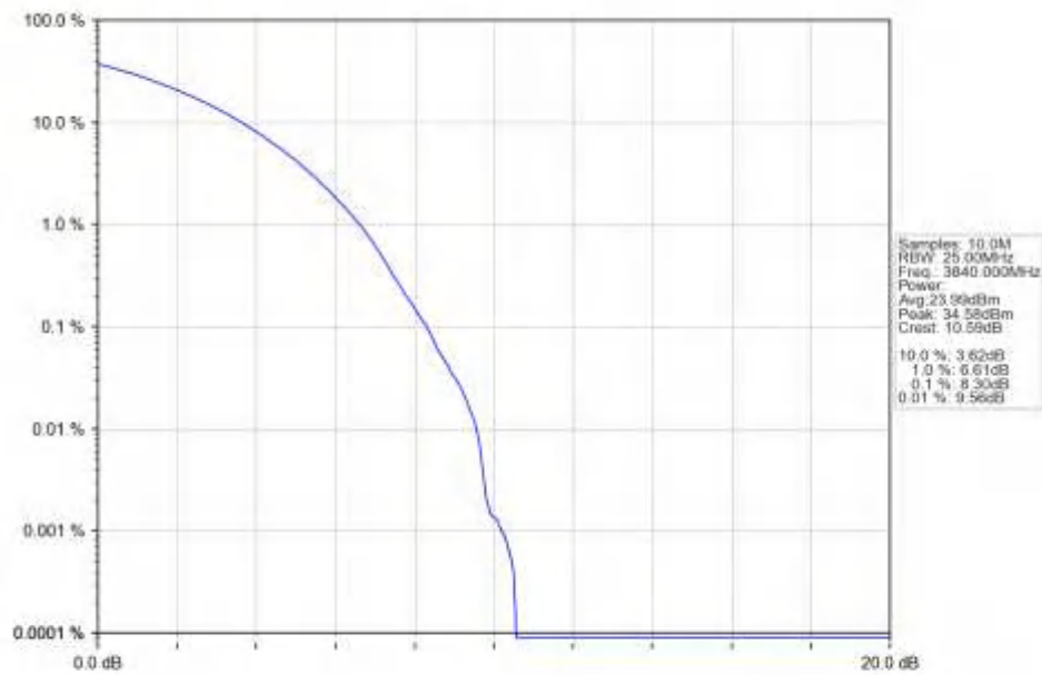
n77a_15kHz_SISO_NTNV_50MHz_CP-OFDM_QPSK_3840MHz_Outer_Full_Ant1
