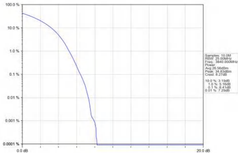
n77a_15kHz_SISO_NTNV_25MHz_DFT-s-OFDM_64_QAM_3840MHz_Outer_Full_Ant1
