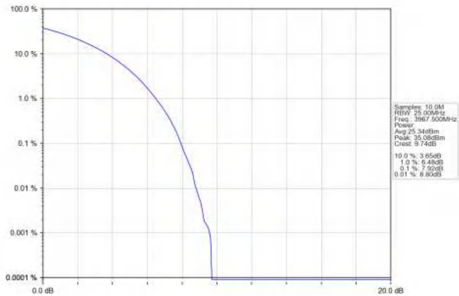
n77a_15kHz_SISO_NTNV_25MHz_CP-OFDM_16_QAM_3967.5MHz_Outer_Full_Ant1
