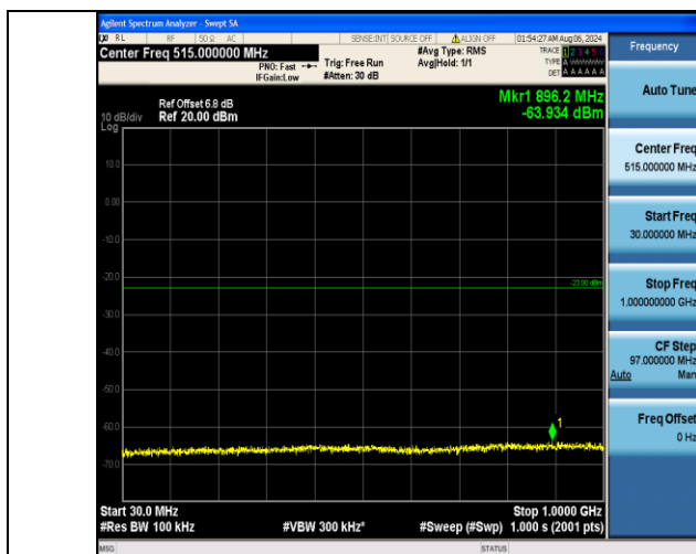
Band2 1.4MHz QPSK 18607 6RB#0 30~1000 30~1000
