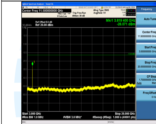
Band2_1.4MHz_16QAM_19193_1RB#5_3000~20000_3000~20000
