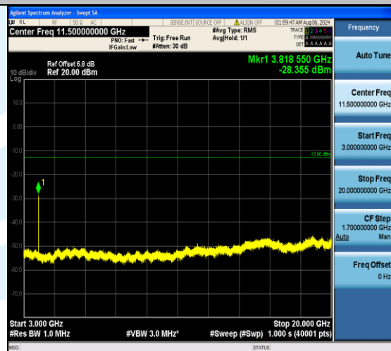
Band2_1.4MHz_16QAM_19193_6RB#0_3000~20000_3000~20000
