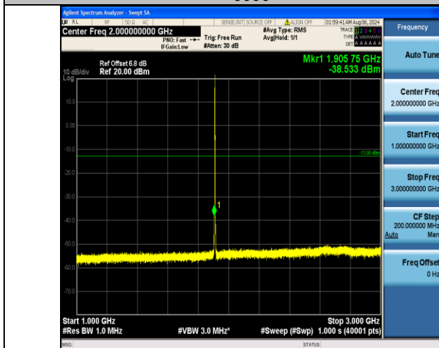
Band2_1.4MHz_16QAM_19193_6RB#0_1000~3000_1000~3000
