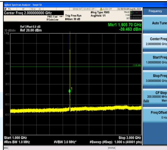
Band2_1.4MHz_16QAM_19193_1RB#5_1000~3000_1000~3000
