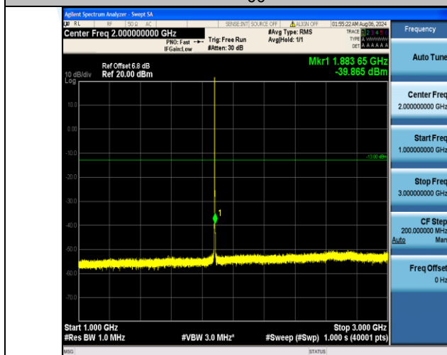
Band2_1.4MHz_QPSK_18900_1RB#0_1000~3000_1000~3000
