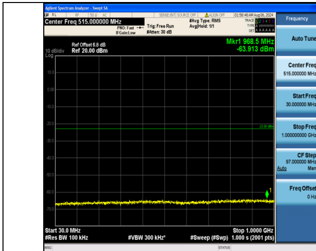
Band2_1.4MHz_16QAM_19193_1RB#5_30~1000_30~1000
