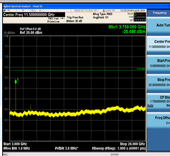
Band2_1.4MHz_QPSK_18900_1RB#0_3000~20000_3000~20000
