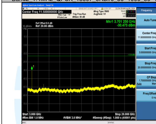
Band2_1.4MHz_QPSK_18607_6RB#0_3000~20000_3000~20000
