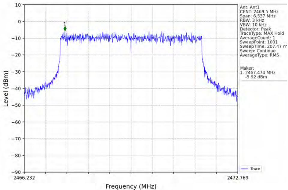
5M_HCH_2469.5MHz_Ant1_NTNV
