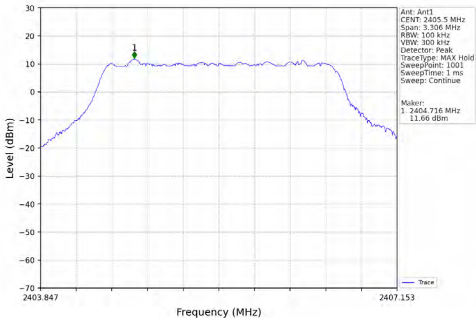
3M_LCH_2405.5MHz_Ant1_NTNV
