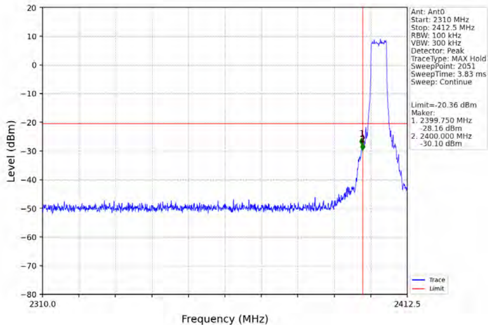
5M_LCH_2404.5MHz_Ant0_NTNV
