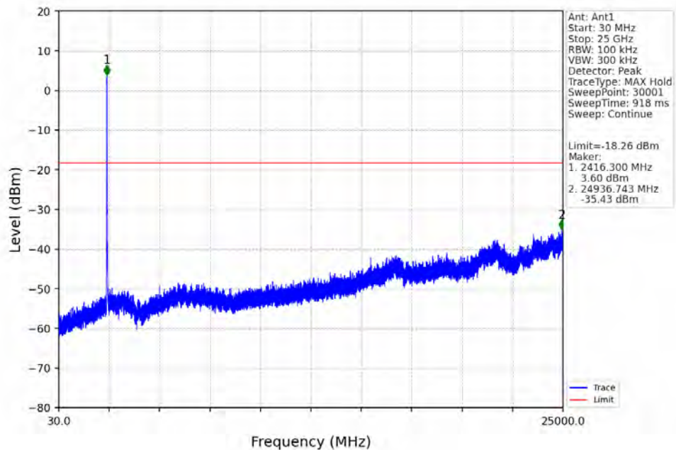
20M_LCH_2412.5MHz_Ant1_NTNV
