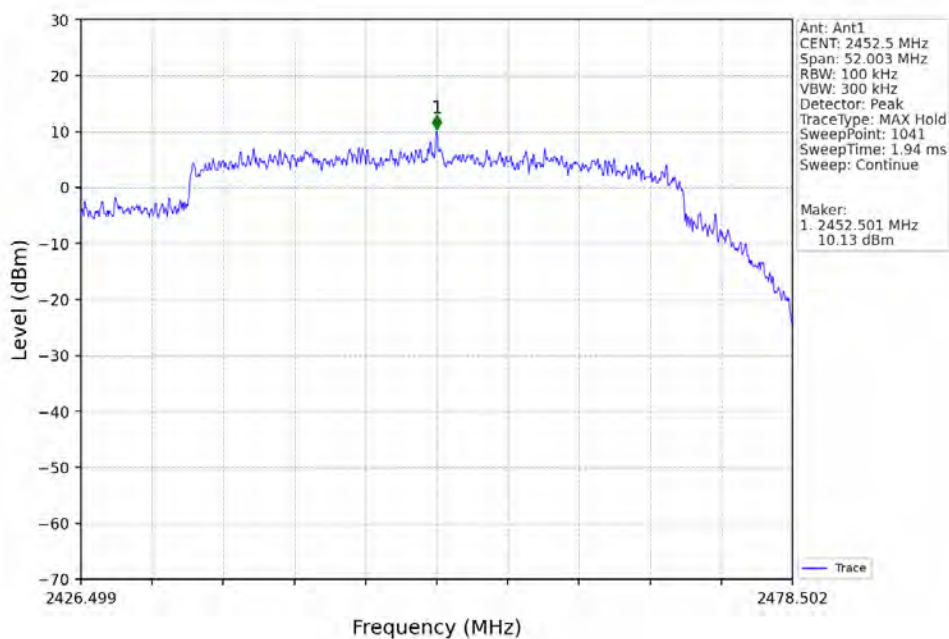
40M_HCH_2452.5MHz_Ant1_NTNV
