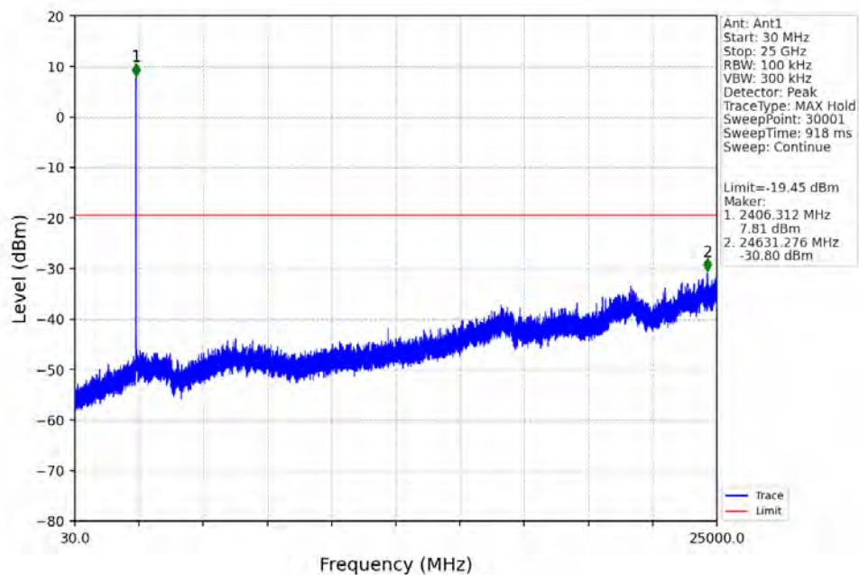
5M_LCH_2404.5MHz_Ant1_NTNV
