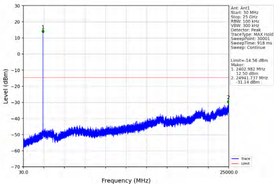
1.4M_LCH_2403.5MHz_Ant1_NTNV
