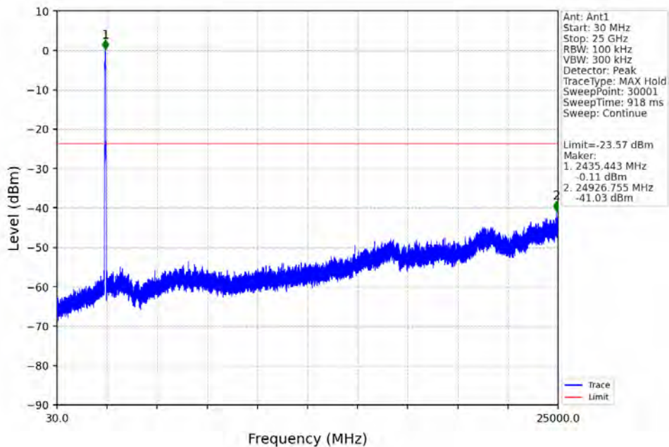
60M_LCH_2432.5MHz_Ant1_NTNV
