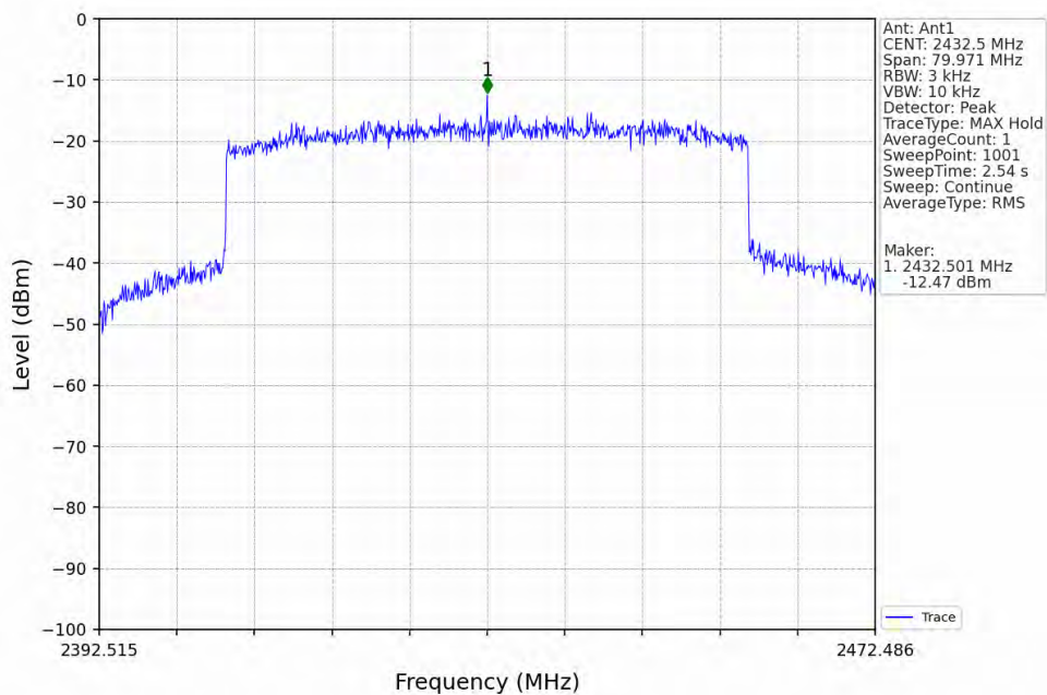
60M_LCH_2432.5MHz_Ant1_NTNV
