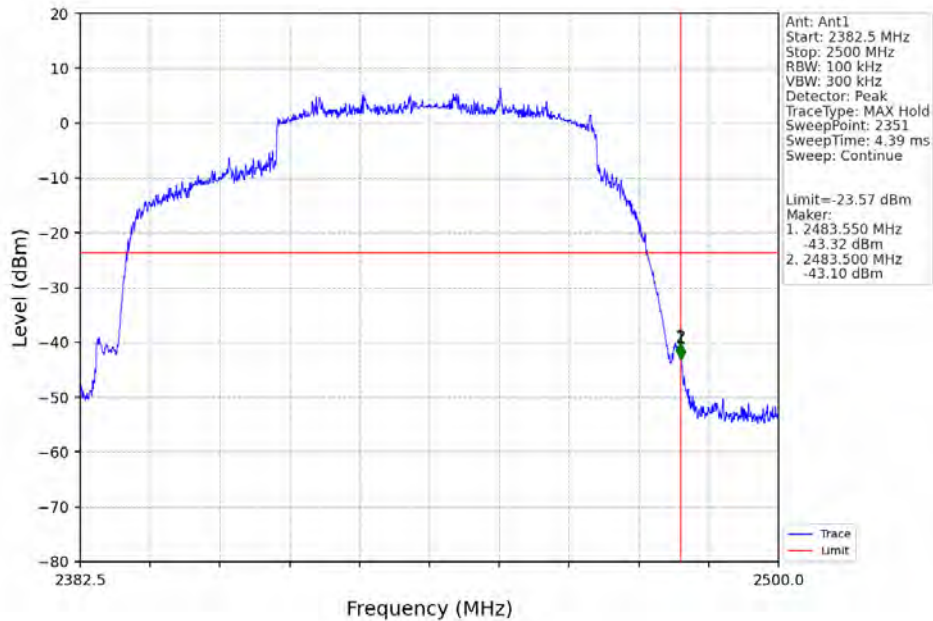
60M_HCH_2442.5MHz_Ant1_NTNV
