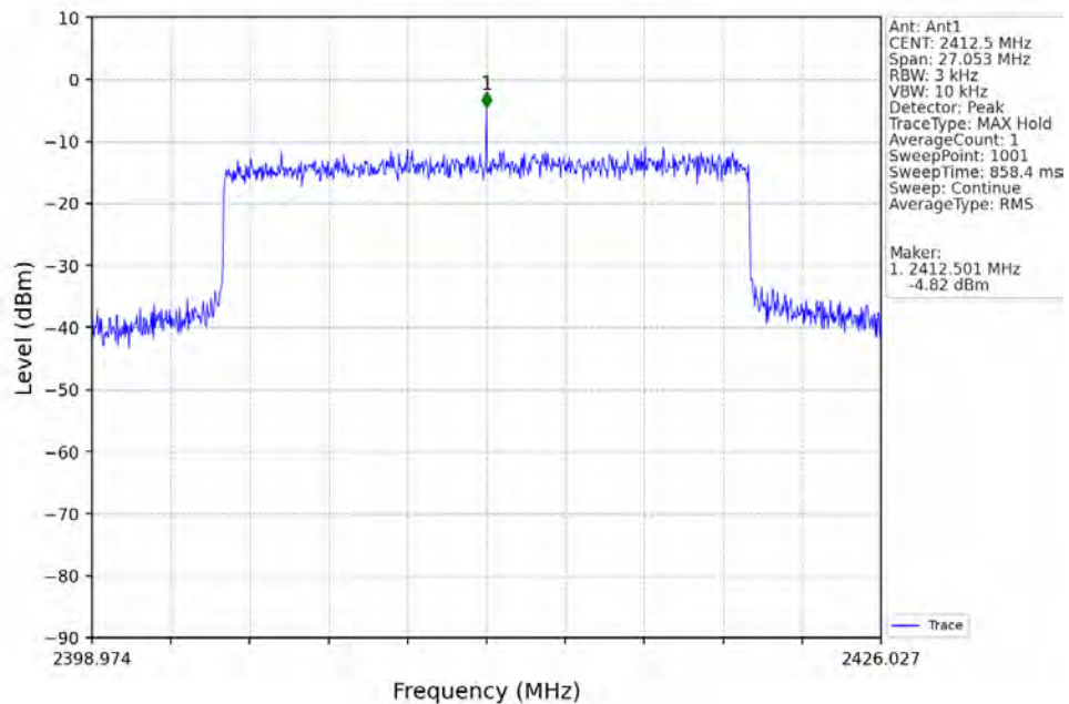
20M_LCH_2412.5MHz_Ant1_NTNV
