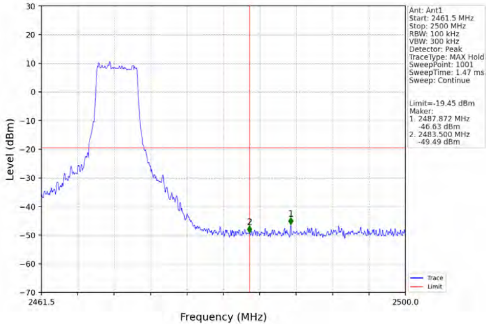
5M_HCH_2469.5MHz_Ant1_NTNV
