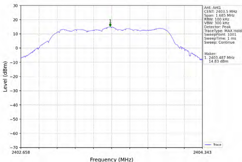
1.4M_LCH_2403.5MHz_Ant1_NTNV
