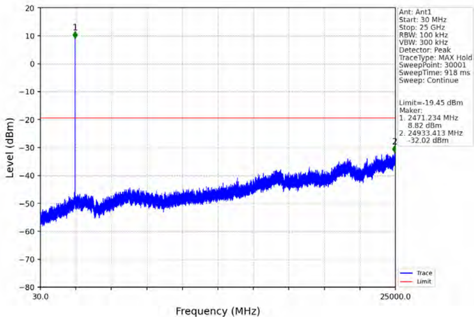
5M_HCH_2469.5MHz_Ant1_NTNV
