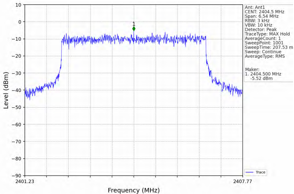
5M_LCH_2404.5MHz_Ant1_NTNV
