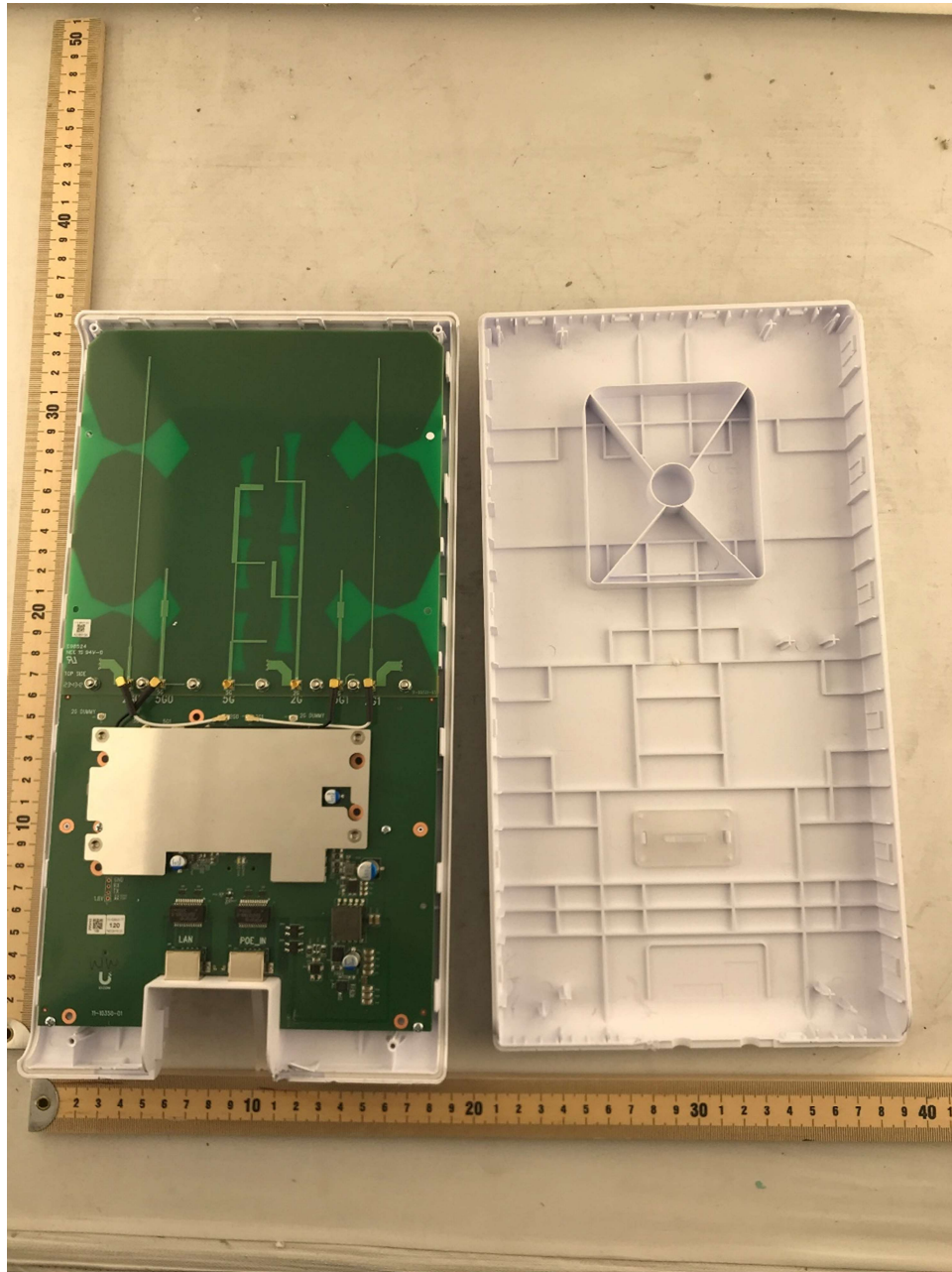
Photograph 1: Internal View With Front Cover Off
