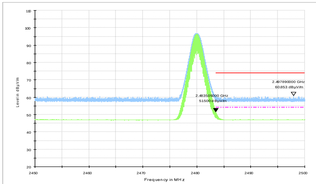
Fig.14. Frequency Band Edges: GFSK, Channel 78, ch11, 2.45 GHz - 2.50GHz
