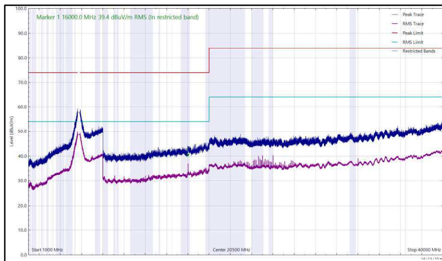
Figure 534 - U-NII-3 - 5745 MHz (CH149), HE20, RU26-0, CDD, Core 0 + Core 1, 1 GHz to 40 GHz, Horizontal
