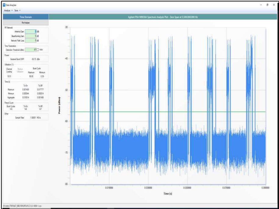
Figure 538 - Channel Loading
