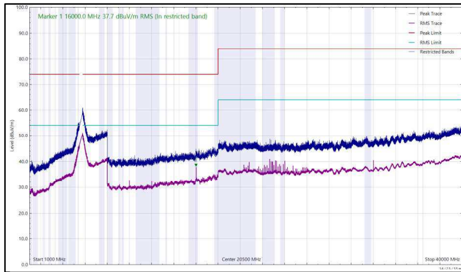
Figure 532 - U-NII-2C - 5700 MHz (CH140), HE20, RU52-37, CDD, Core 0 + Core 1, 1 GHz to 40 GHz, Horizontal
