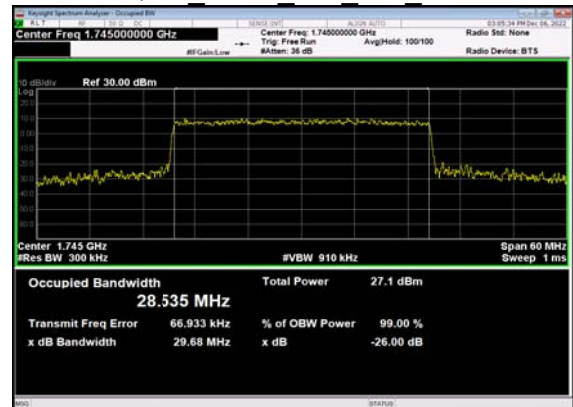
N66(30M)_CP-OFDM_64 QAM Outer Full Mid CH
