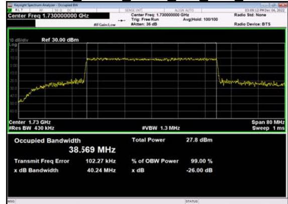
N66(40M)_CP- OFDM QPSK Outer Full Low CH
