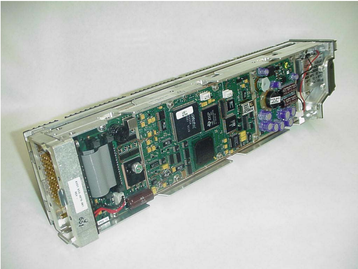
Photo 6: Assembled VHF-4000E, with cover removed. View of DSP/Power Supply Circuit Card side
