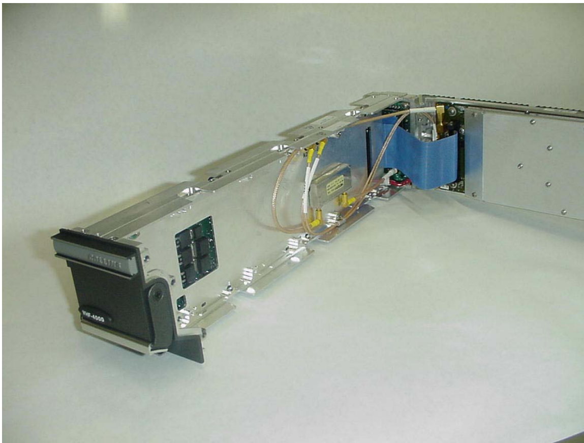
Photo 7: Open Chassis view of VHF-4000E showing RF card assembly on the right, interconnections, and chassis web under DSP/Power Supply. The Connectorized component at middle right is a lowpass filter in both receive and transmit paths. See circuit description, exhibit L.
