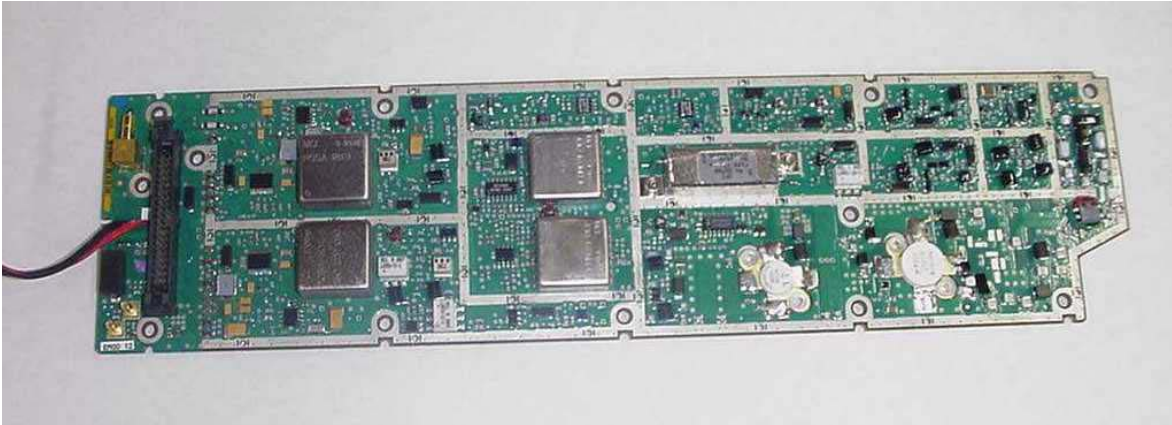
Photo 3: RF Circuit Card, Top View
