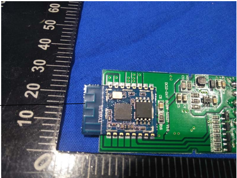
Wifi antenna
