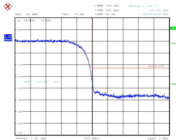
Figure 2-53a: Band II, HSPA High Channel Mask
