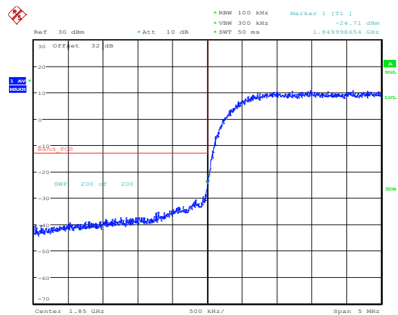
Figure 2-52a: Band II, HSPA Low Channel Mask
