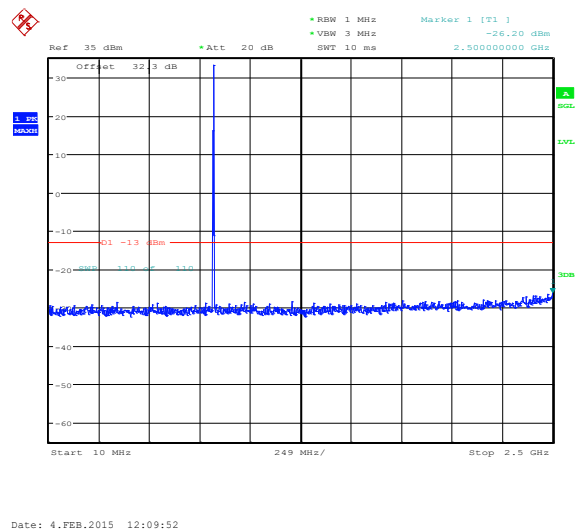
Figure 1-39a: GSM850 band, Spurious Conducted Emissions, Low channel in Edge Mode
