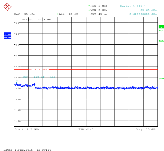
Figure 1-42a: GSM850 band, Spurious Conducted Emissions, Middle channel in Edge Mode
