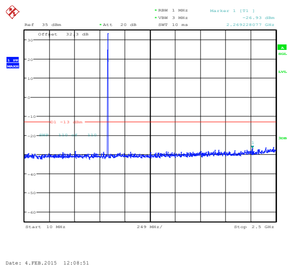
Figure 1-41a: GSM850 band, Spurious Conducted Emissions, Middle channel in Edge Mode
