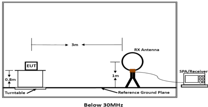
Below 30MHz
