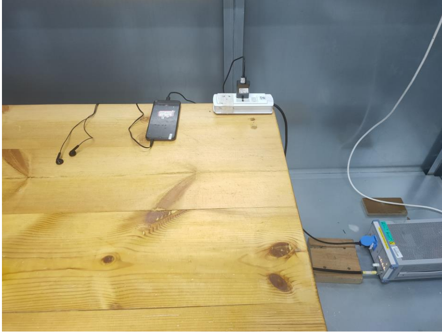
13. Conducted Emission (Part 15C, Bluetooth/Wi-Fi)
