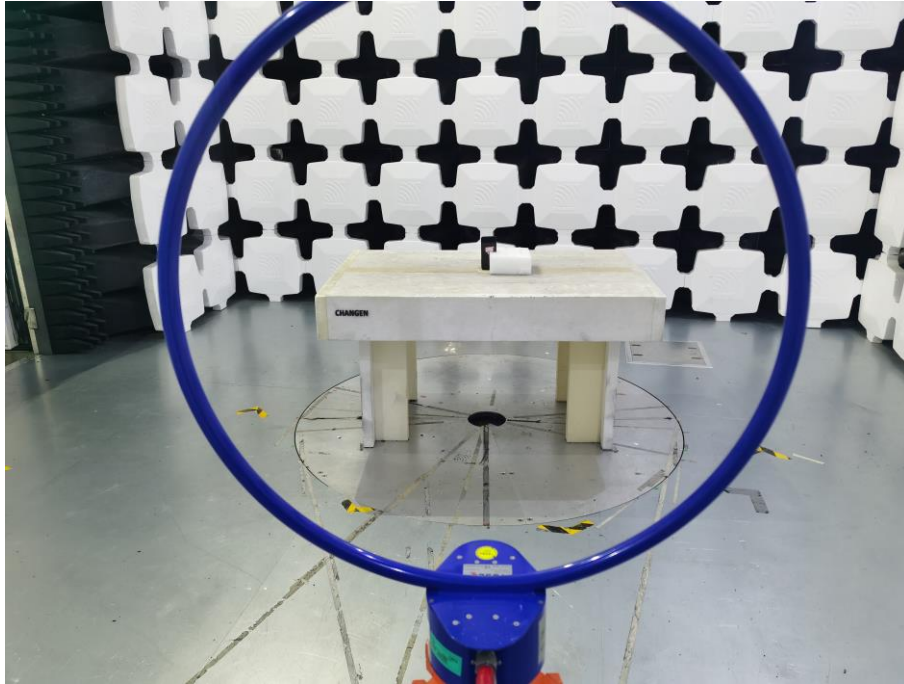
5. Radiated Emissions (Part 15C, 9kHz-30MHz)
