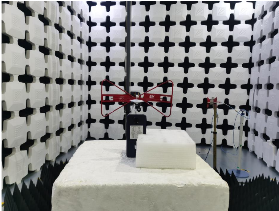
9. Radiated Emissions (Part 22/24/27,30MHz-18GHz)
