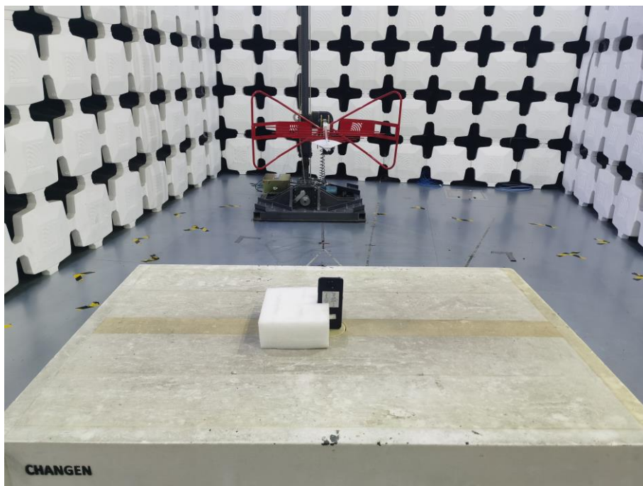
6. Radiated Emissions (Part 15C, 30MHz-1GHz)
