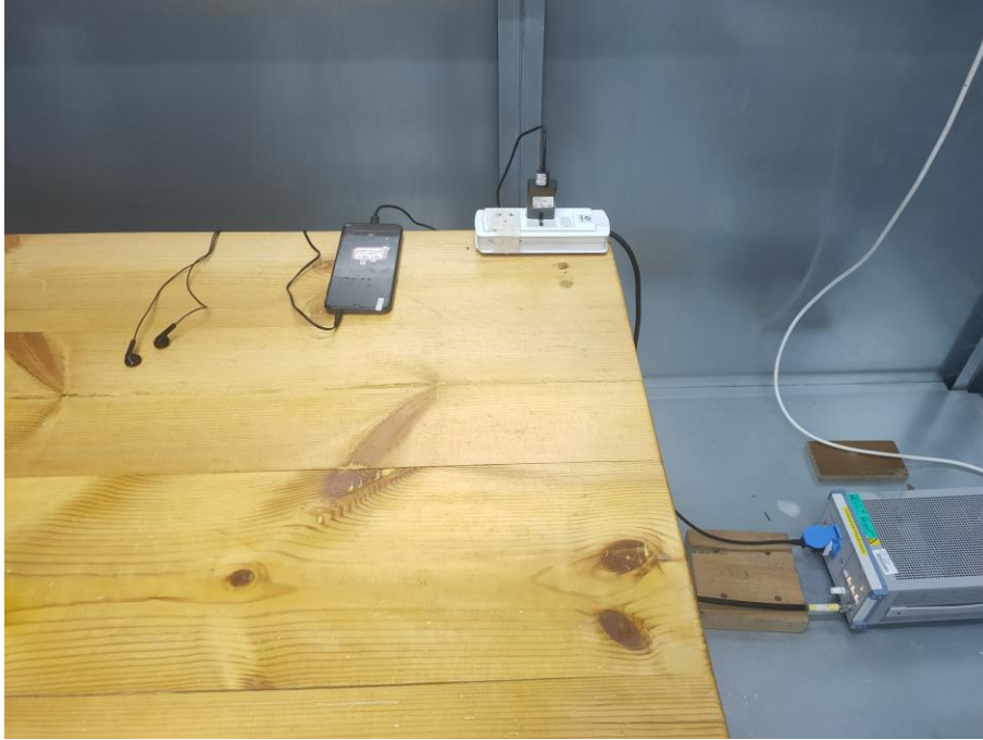
11. Conducted Emission (Part 15B, Camera/Video Player/GNSS/ FM receiver)
