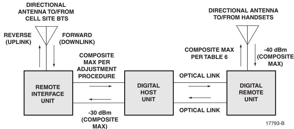
Figure 9. Remote BTS Interface Block Diagram
