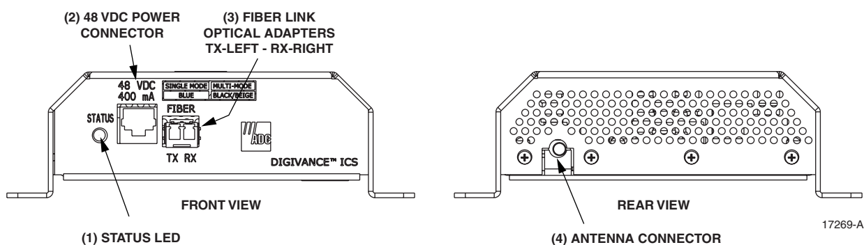
Figure 5. Digital Remote Unit User Interface
