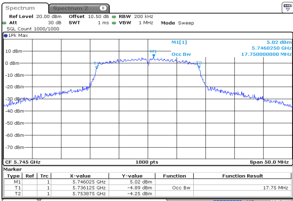
n20_5745MHz_Chain 0
