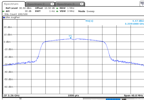
n20_5260MHz_Chain 0
