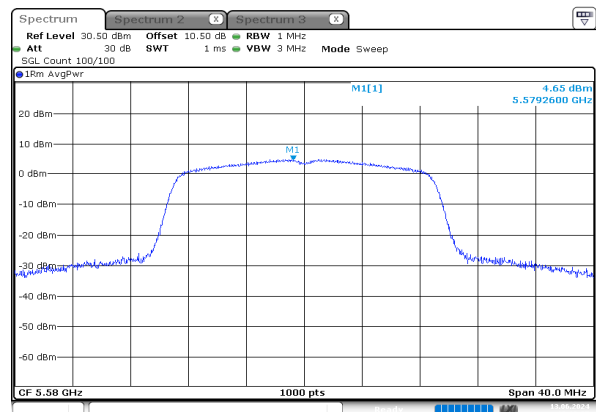
n20_5580MHz_Chain 0
