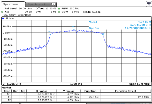
n20_5785MHz_Chain 0
