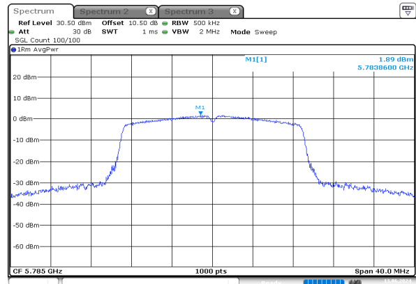
n20_5785MHz_Chain 0
