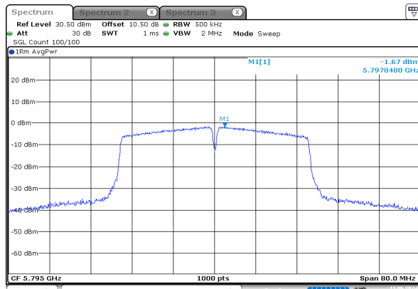
n40_5795MHz_Chain 0
