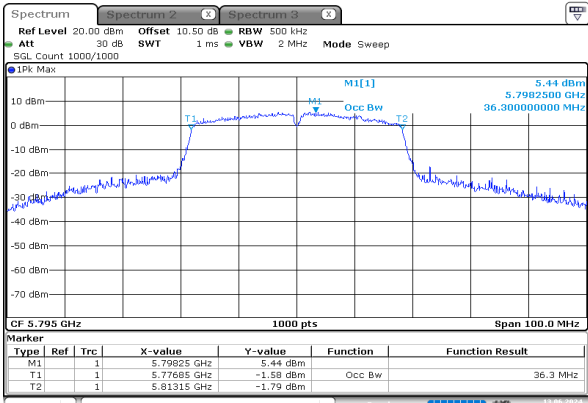
n40_5795MHz_Chain 0
