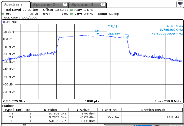
ac80_5775MHz_Chain 0
