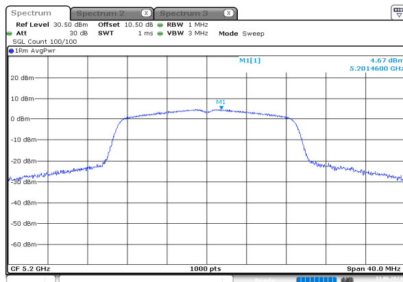
n20_5200MHz_Chain 0
