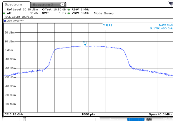
a_5180MHz_Chain 0
