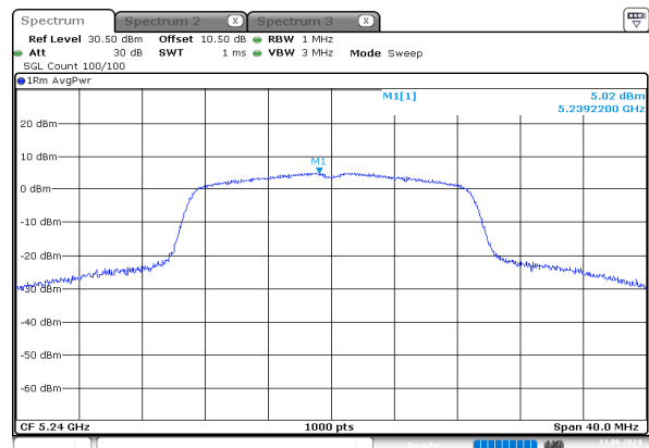
n20_5240MHz_Chain 0
