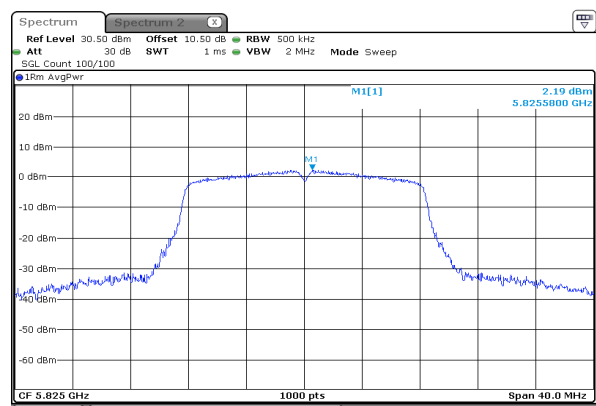
a_5825MHz_Chain 0
