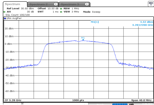
n20_5280MHz_Chain 0
