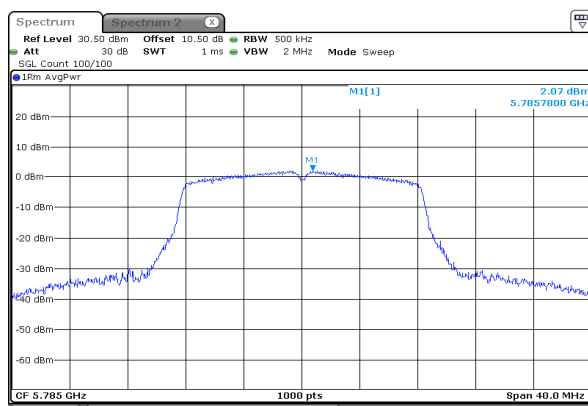
a_5785MHz_Chain 0
