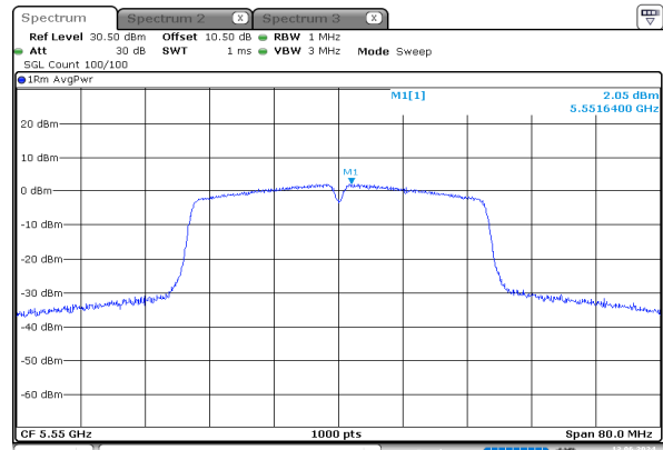
n40_5550MHz_Chain 0
