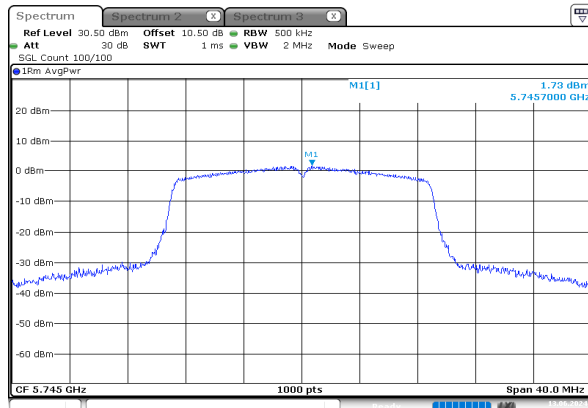
n20_5745MHz_Chain 0
