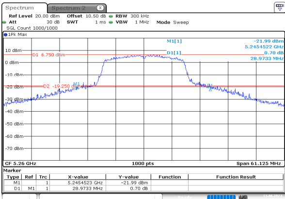
n20_5260MHz_Chain 0
