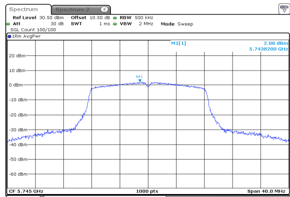
a_5745MHz_Chain 0
