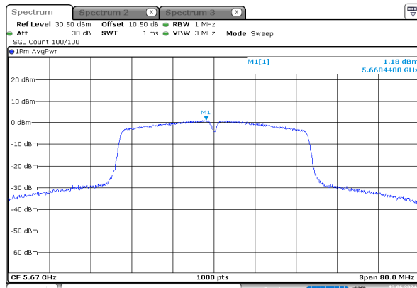
n40_5670MHz_Chain 0
