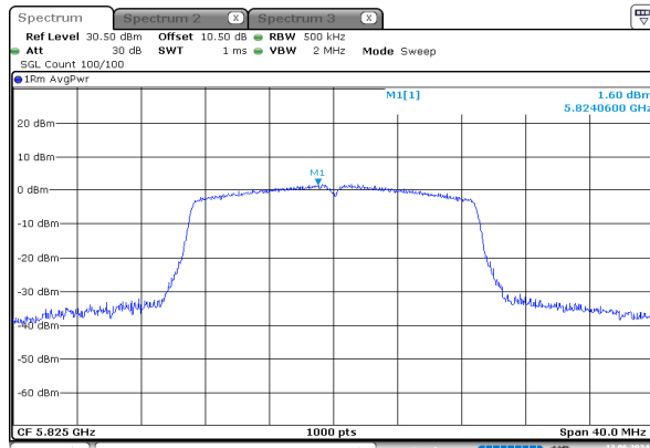
n20_5825MHz_Chain 0
