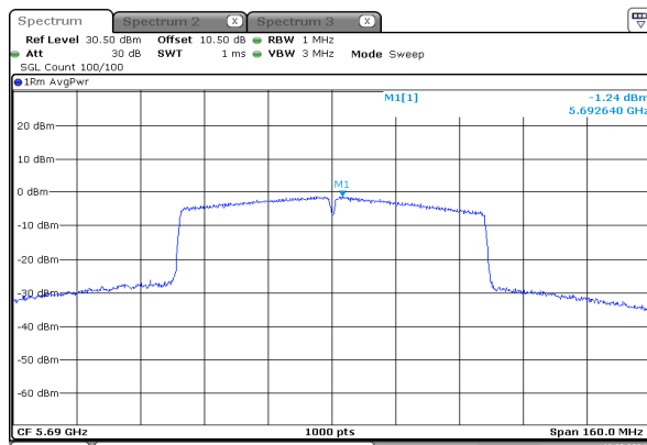
ac80_5690MHz_Chain 0
