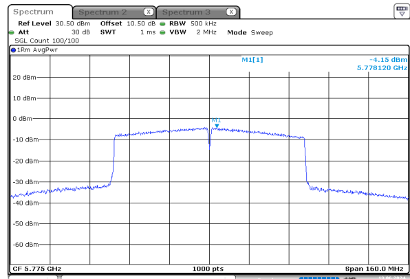
ac80_5775MHz_Chain 0
