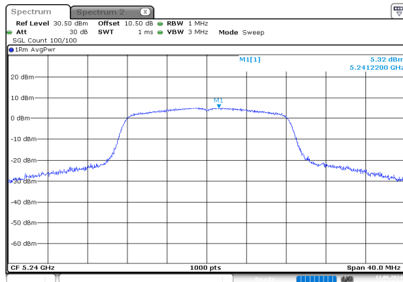
a_5240MHz_Chain 0
