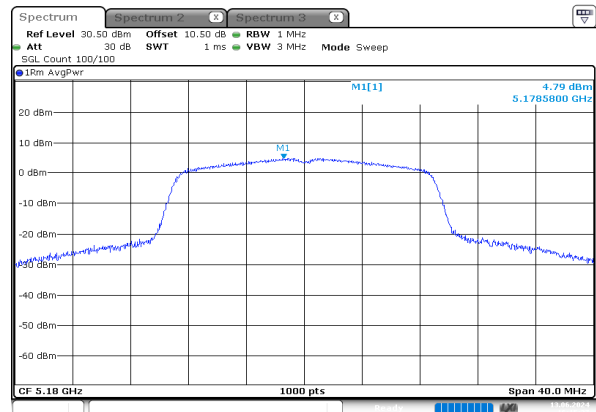
n20_5180MHz_Chain 0
