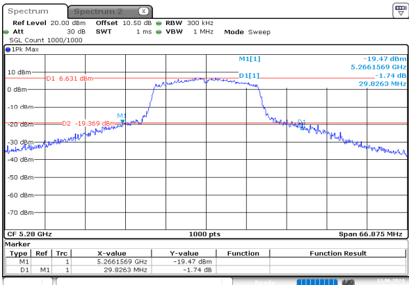
n20_5280MHz_Chain 0
