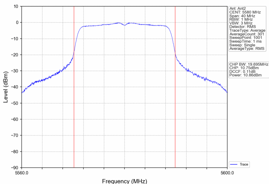
802.11n(HT20)_MCH_5580MHz_Ant2_NTNV
