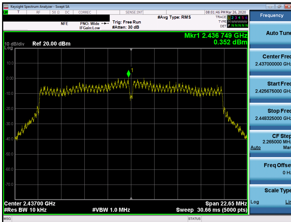
Plot 7-26. Power Spectral Density Plot SISO ANT1 (802.11n (2.4GHz) – Ch. 6)
