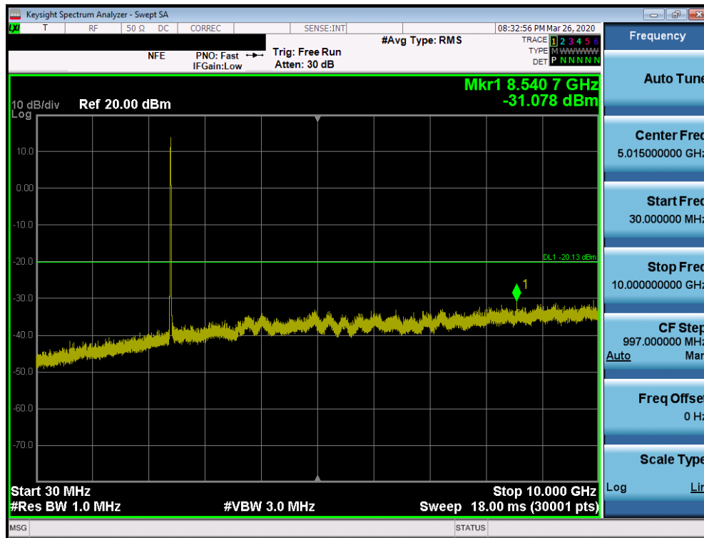
Plot 7-49. Conducted Spurious Plot SISO ANT1 (802.11b – Ch. 1)
