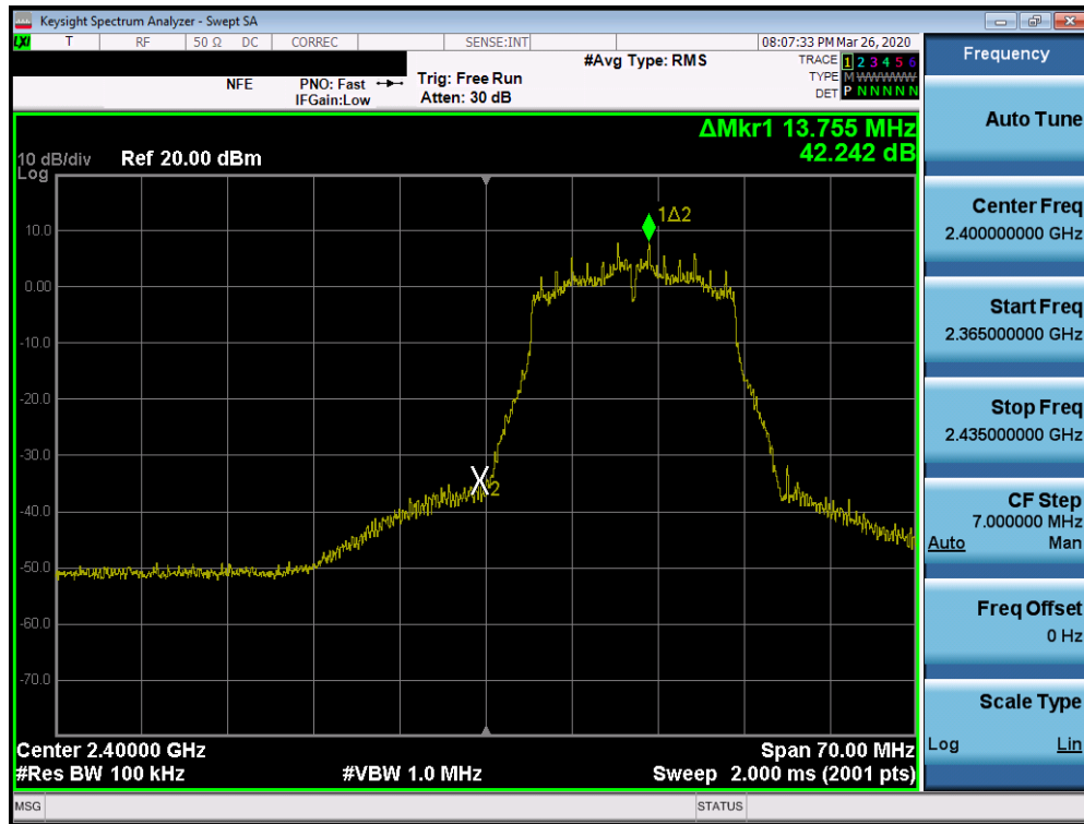
Plot 7-39. Band Edge Plot SISO ANT1 (802.11g- Ch. 1)
