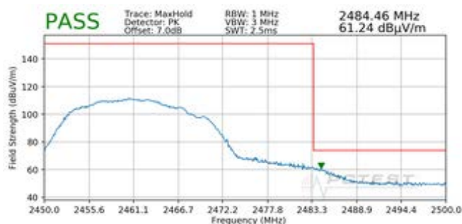
Plot 7-84. Radiated Restricted Upper Band Edge Measurement MIMO (Peak)
