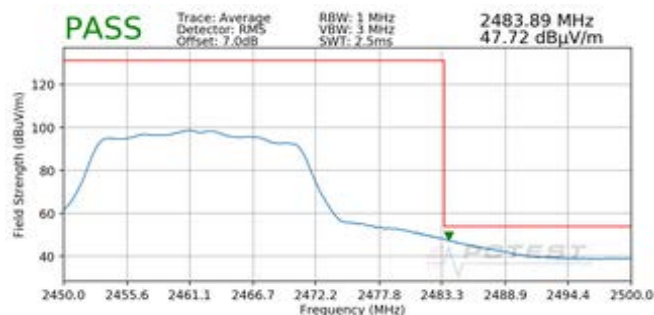
Plot 7-75. Radiated Restricted Upper Band Edge Measurement SISO ANT1 (Average)
