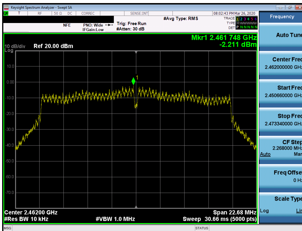
Plot 7-27. Power Spectral Density Plot SISO ANT1 (802.11n (2.4GHz) – Ch. 11)
