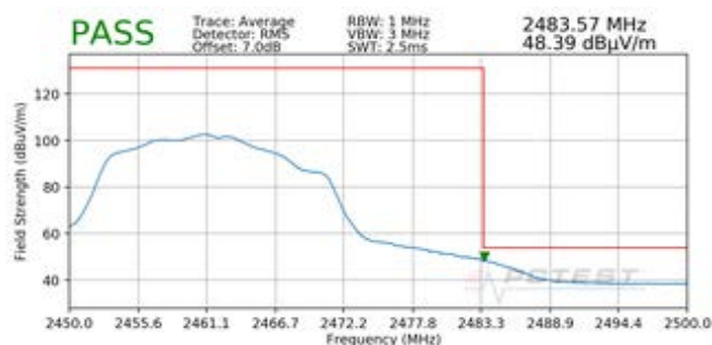
Plot 7-83. Radiated Restricted Upper Band Edge Measurement MIMO (Average)
