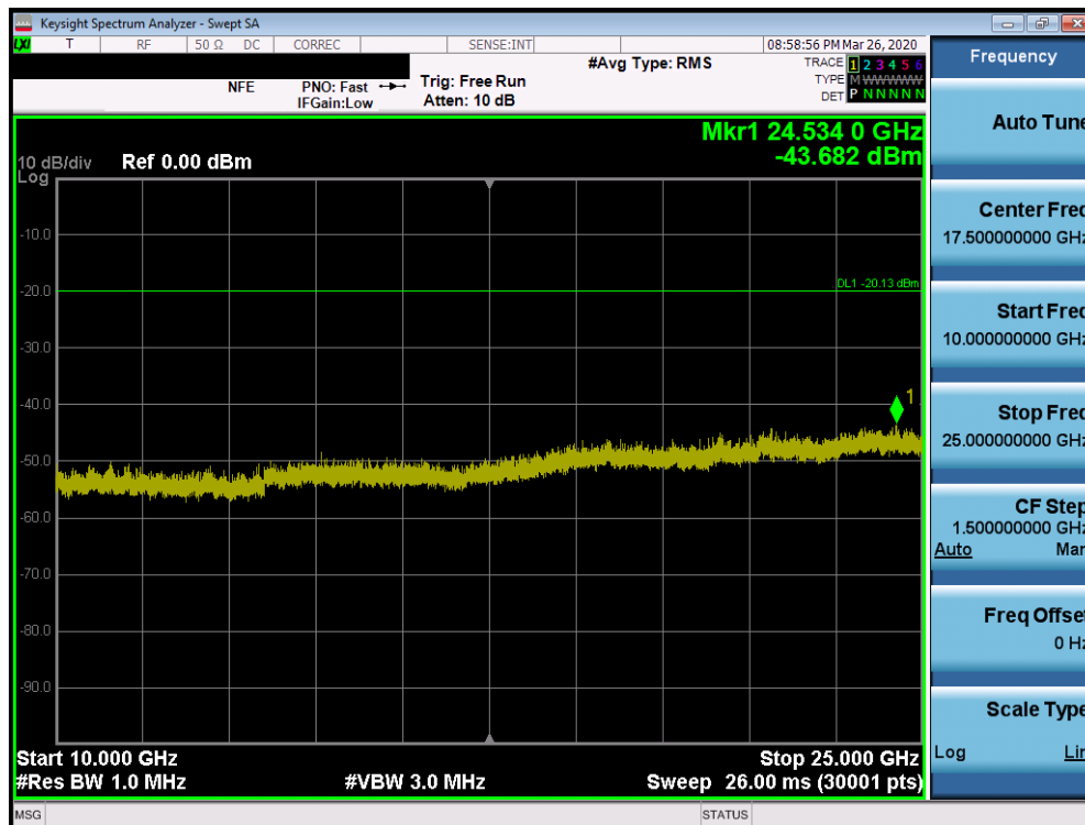
Plot 7-50. Conducted Spurious Plot SISO ANT1 (802.11b – Ch. 1)
