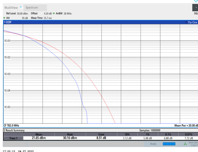
Band13-10MHz-16QAM-23230-27RB#0
