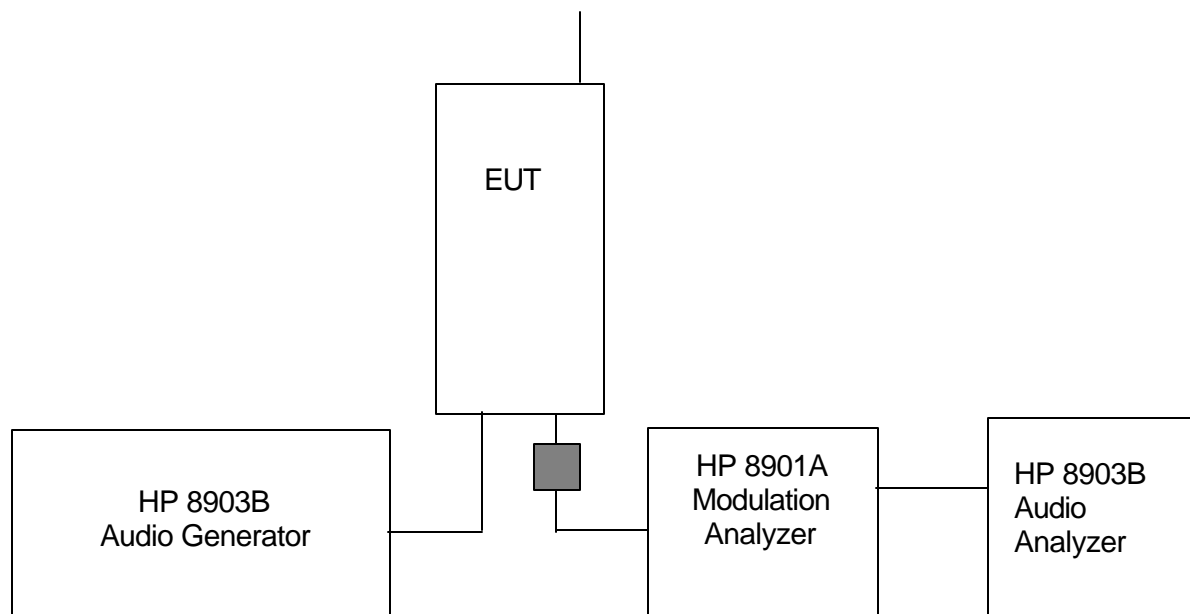
Fig. 3. Transmitter Audio Frequency & Tone Modulation Test Setup.
