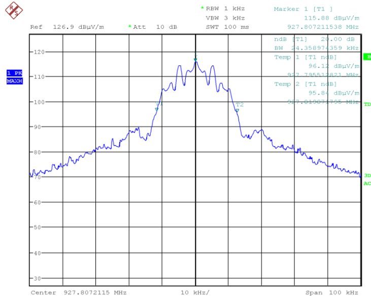
Graph 4: Highest Channel Bandwidth
