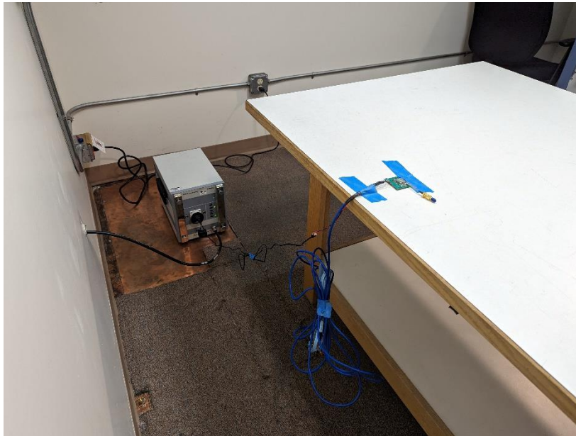
Photograph 14: Back View Conducted Emissions Worst-Case Configuration
