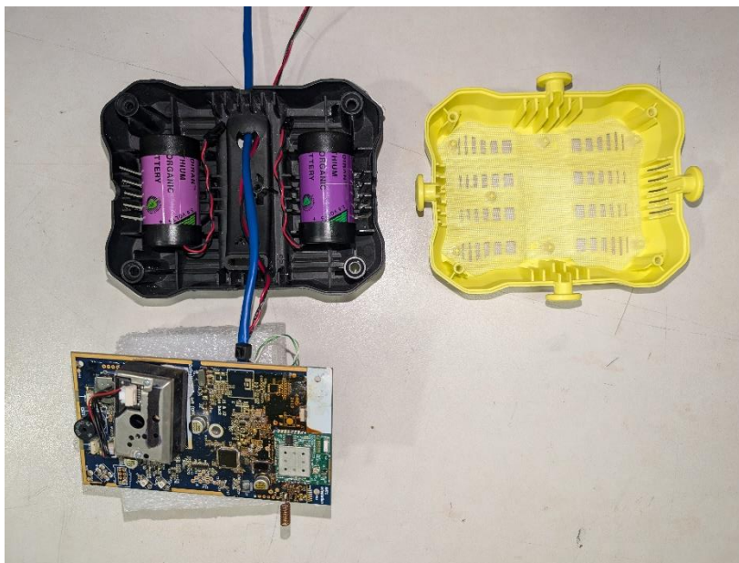
Photograph 24: View of the Host PCB Removed from the Enclosure
