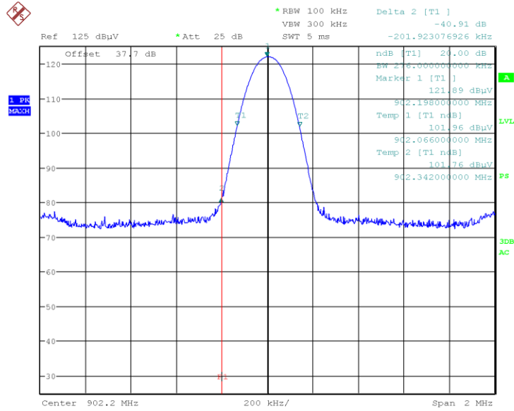
Graph 19: Radiated Lower Band Edge Plot (L-Com HG908P-RTP)
