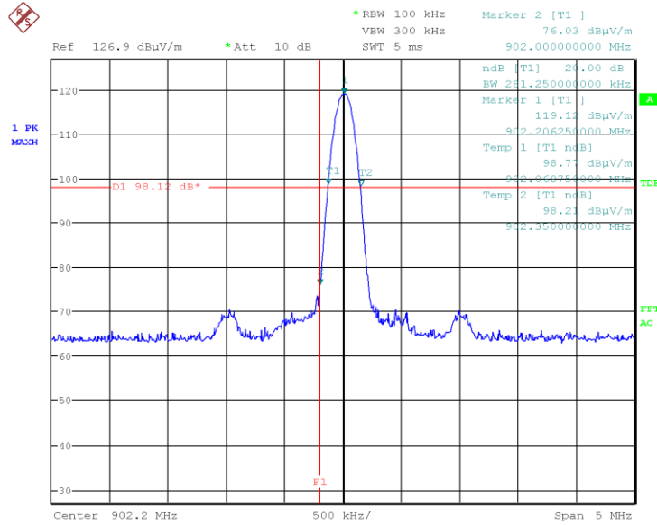
Graph 15: Radiated Lower Band Edge Plot (G-NiceRF SW915-TH12)
