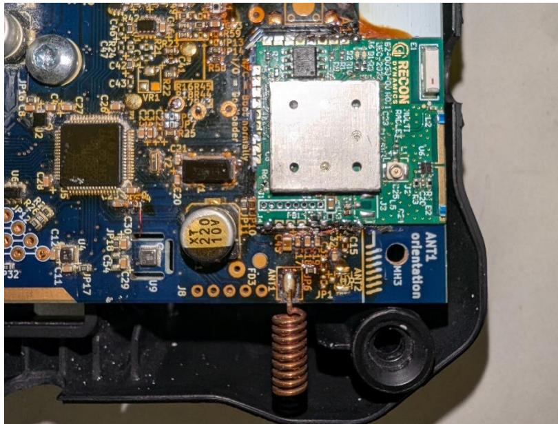
Photograph 31: View of Front of Module in the Host PCB and the RF Circuitry of the Wire-Wound Internal 900MHz Antenna
