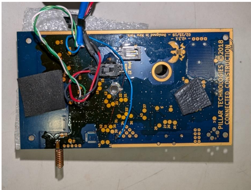
Photograph 26: Back View of Module in the Host PCB and the RF Circuitry of the Wire-Wound Internal 900MHz Antenna
