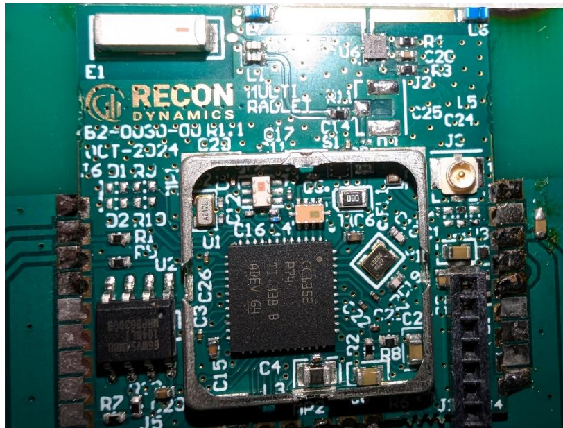
Photograph 33: Close-up View of Front of Module with RF Shield Removed (EUT for All Testing Except Internal 900Mhz Antenna)
