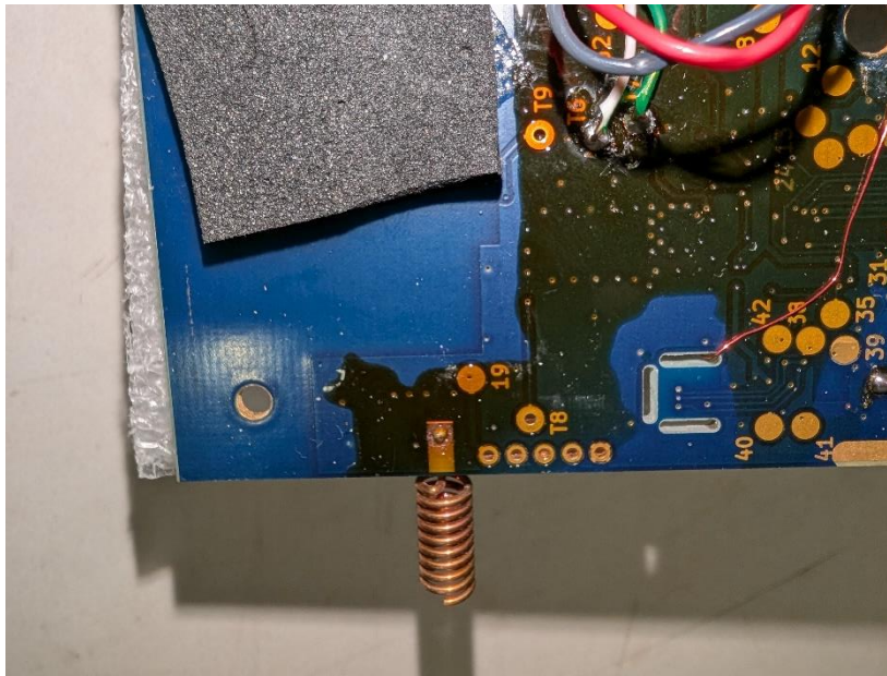
Photograph 25: Closeup View of Front of the RF Circuitry of the Wire-Wound Internal 900MHz Antenna on the Bottom of the Host PCB
