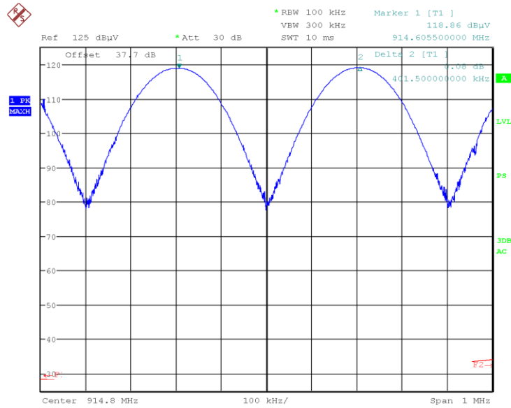
Graph 9: Hopping Mode Channel Separation is 401.5 kHz
