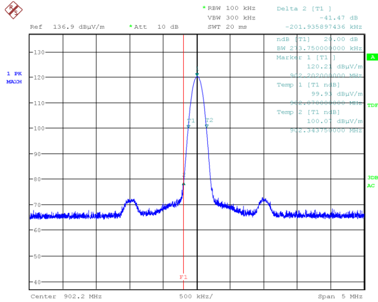
Graph 17: Radiated Lower Band Edge Plot (L-Com HG908UP)
