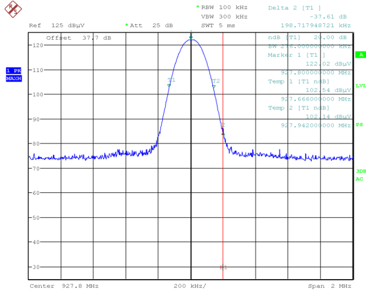
Graph 20: Radiated Upper Band Edge Plot (L-Com HG908P-RTP)
