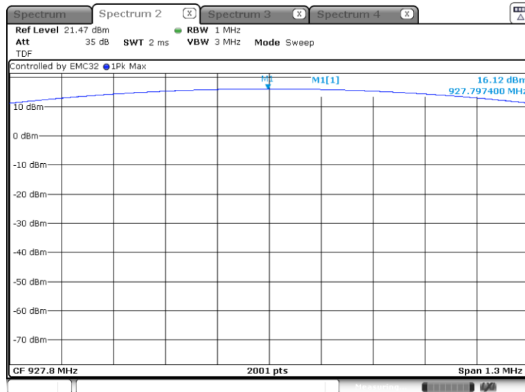
Graph 14: Highest Channel Output Power Plot
