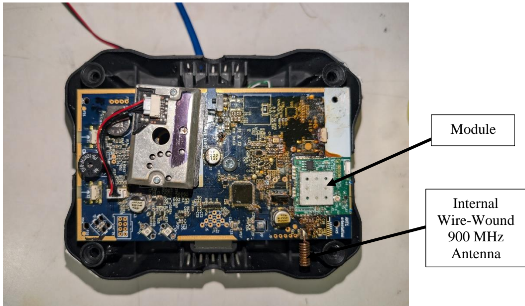
Photograph 22: View of the Module in the Host PCB with Enclosure Cover Removed
