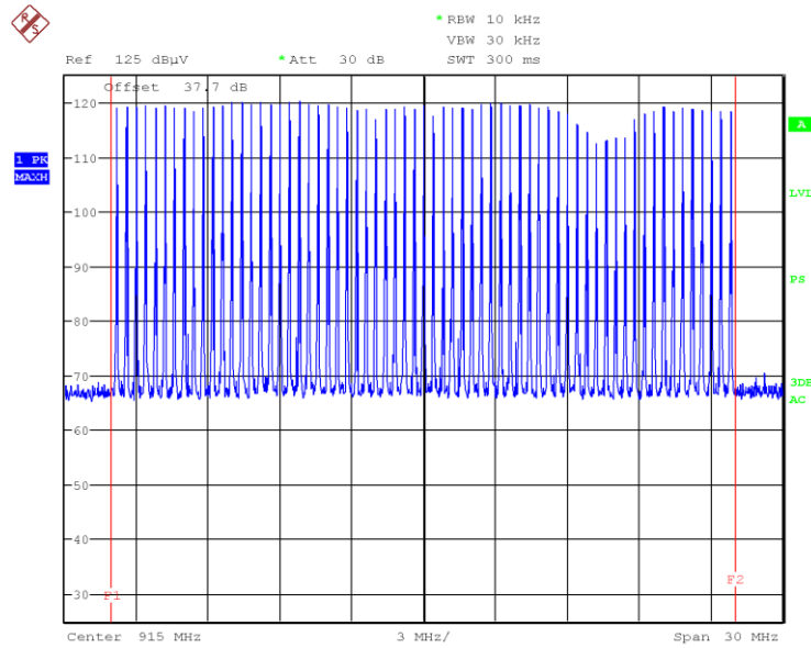
Graph 5: Full Authorized Band Channel Hopping Map
