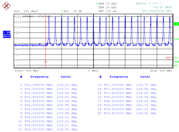
Graph 6: Hopping Mode Channels from 900MHz to 910MHz Containing 20 Channels
