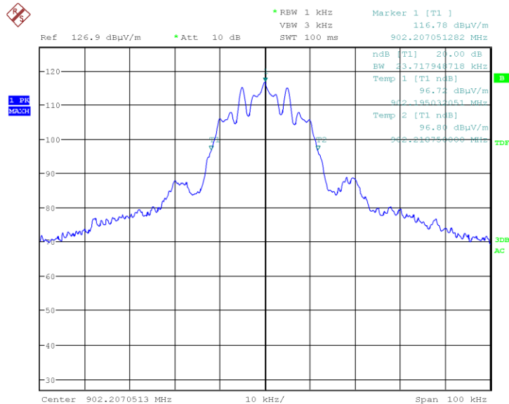
Graph 2: Lowest Channel Bandwidth
