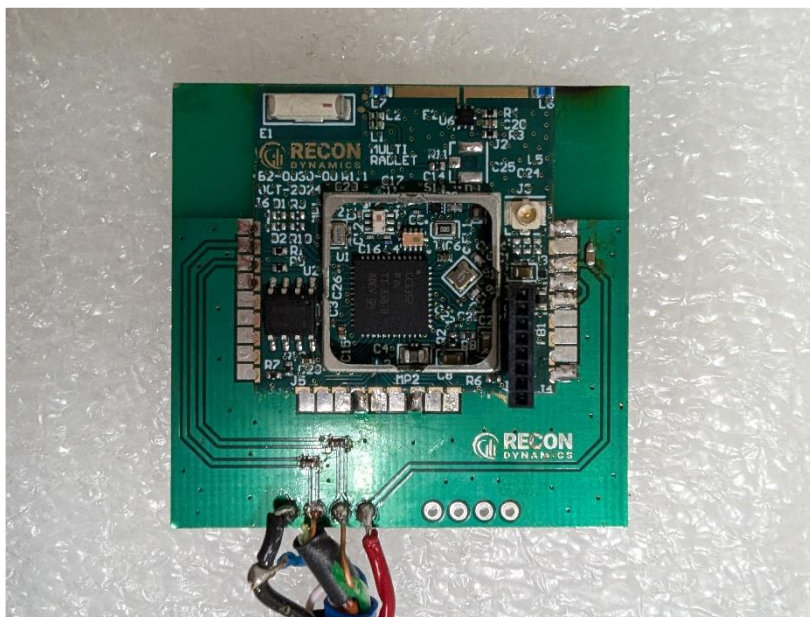
Photograph 32: View of Front of Module with RF Shield Removed (EUT for All Testing Except Internal 900Mhz Antenna)
