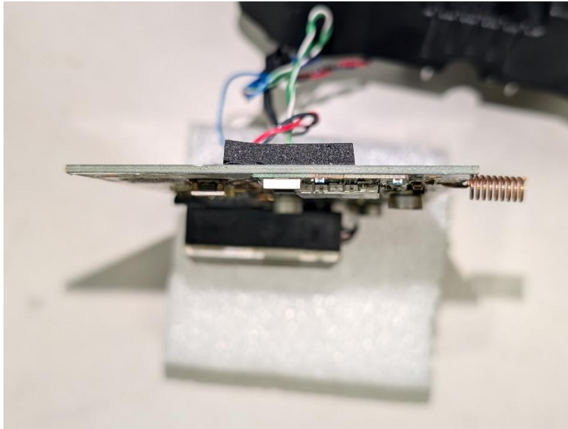
Photograph 29: Side 3 of the Host PCB
