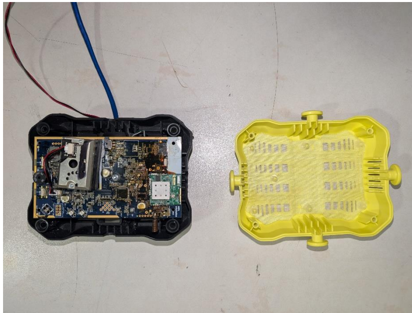
Photograph 21: View of the EUT Enclosure Cover Removed
