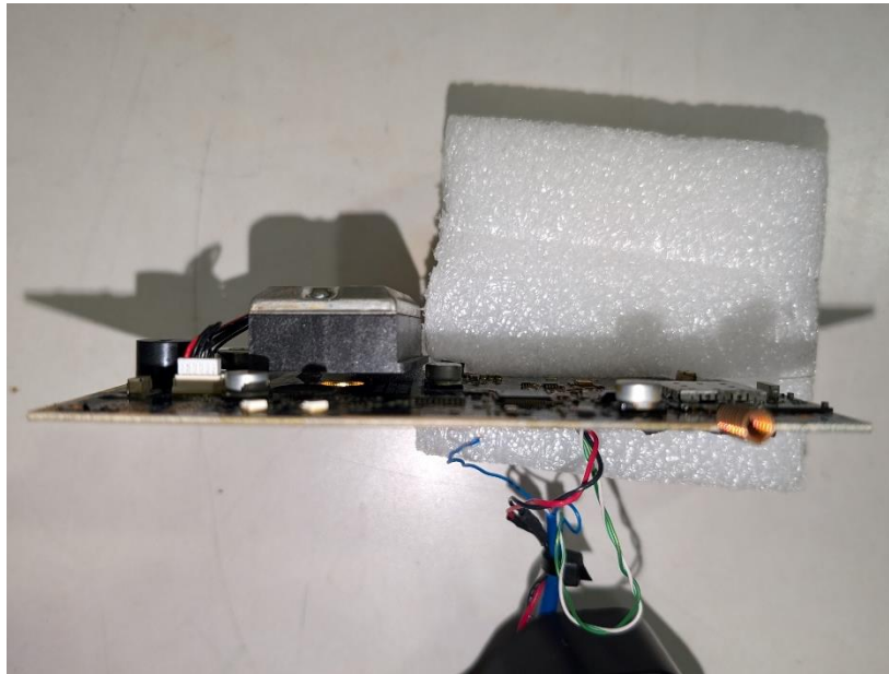
Photograph 28: Side 2 of the Host PCB
