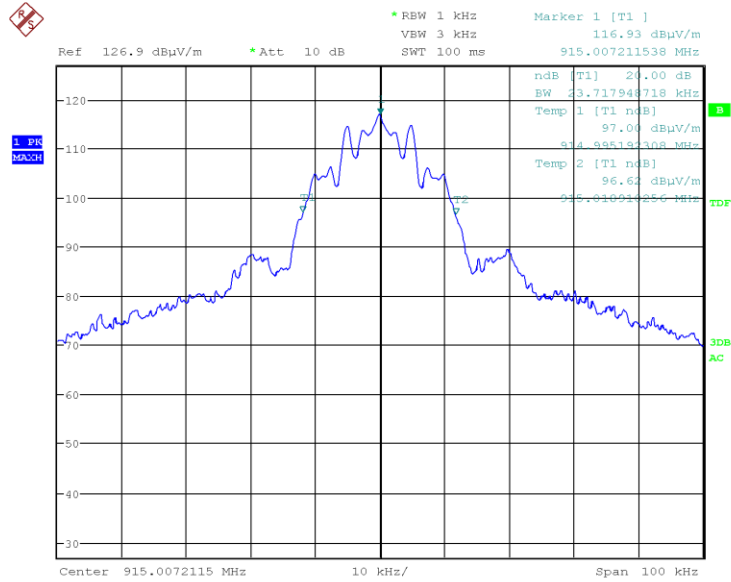
Graph 3: Middle Channel Bandwidth
