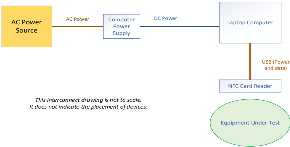
Figure 2: Block diagram of equipment arrangement A6
