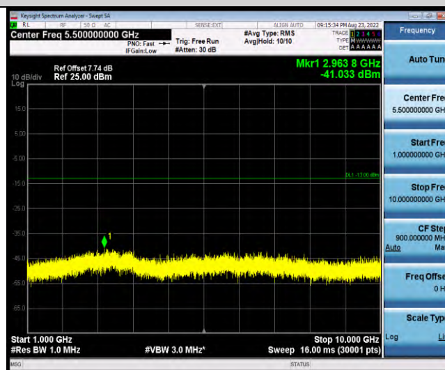
Band18-Stand-Alone-NaN-BPSK-23852-1@11-15kHz-1000-10000-1000~10000MHz@-41.03dBm--13-PASS
