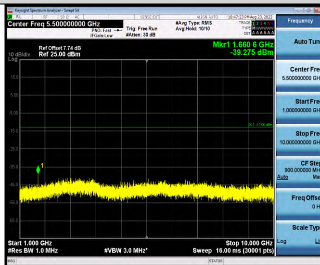
Band19-Stand-Alone-NaB-PSK-24002-1@0-15kHz-1000-10000-1000~10000MHz@-39.28dBm--13-PASS
