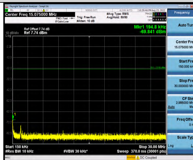
Band19-Stand-Alone-NaN-QPSK-24002-1@47-3.75kHz-0.15-30-0.15~30MHz@-69.84dBm--23-PASS
