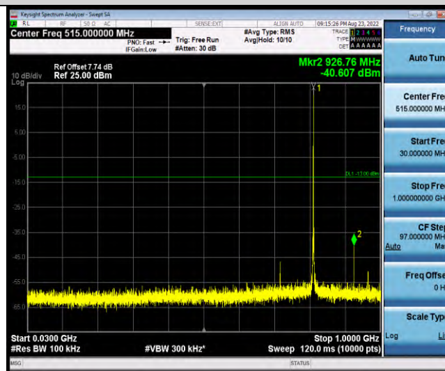
Band18-Stand-Alone-NaN-BPSK-23852-1@11-15kHz-30-1000-30~1000MHz@-40.61dBm--13-PASS
