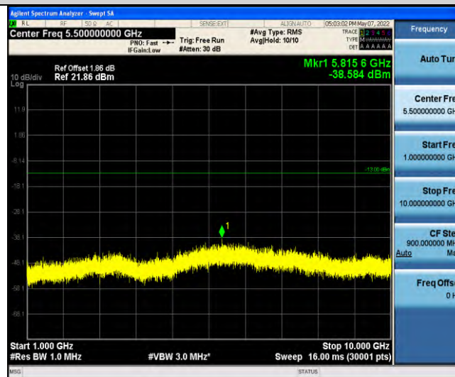
Band17-Stand-Alone-NaN-BPSK-23732-1@11-15kHz-1000-10000-1000~10000MHz@-38.58dBm--13-PASS
