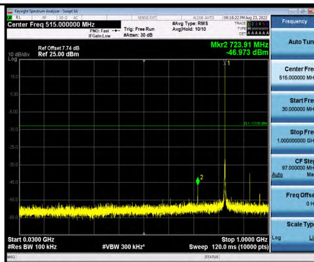
Band18-Stand-Alone-NaN-BPSK-23998-1@11-15kHz-30-1000-30~1000MHz@-46.97dBm--13-PASS
