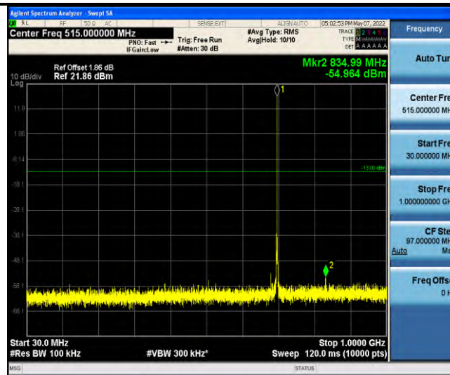
Band17-Stand-Alone-NaN-BPSK-23732-1@11-15kHz-30-1000-30~1000MHz@-54.96dBm--13-PASS
