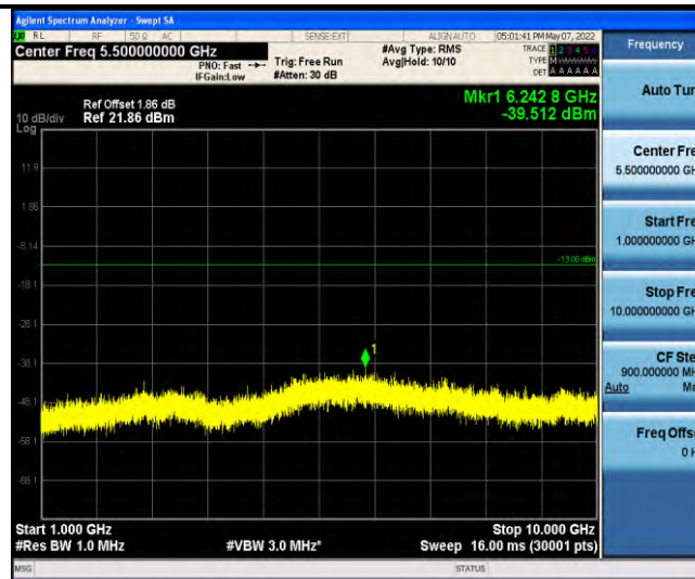
Band17-Stand-Alone-Na-N-BPSK-23732-1@0-15kHz-1000-10000-1000~10000MHz@-39.51dBm--13-PASS
