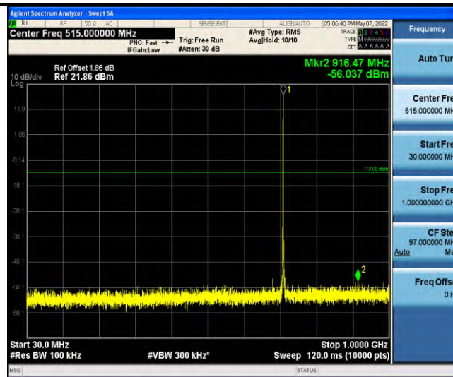
Band17-Stand-Alone-NaB-PSK-23848-1@0-15kHz-30-1000-30~1000MHz@-56.04dBm--13-PASS
