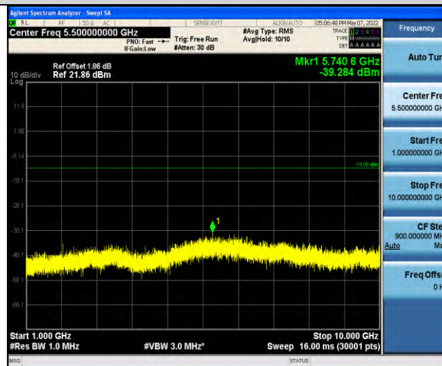
Band17-Stand-Alone-NaB-PSK-23848-1@0-15kHz-1000-10000-1000~10000MHz@-39.28dBm--13-PASS
