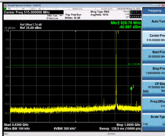
Band18-Stand-Alone-Na-N-QPSK-23852-1@0-3.75kHz-30-1000-30-1000MHz@-40.9dBm--13-PASS
