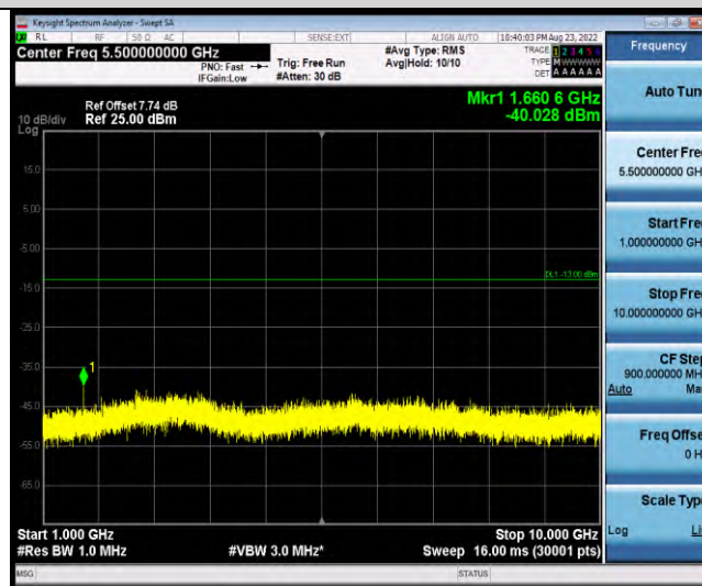
Band19-Stand-Alone-NaN-QPSK-24002-1@47-3.75kHz-1000-10000-1000~10000MHz@-40.03dBm--13-PASS
