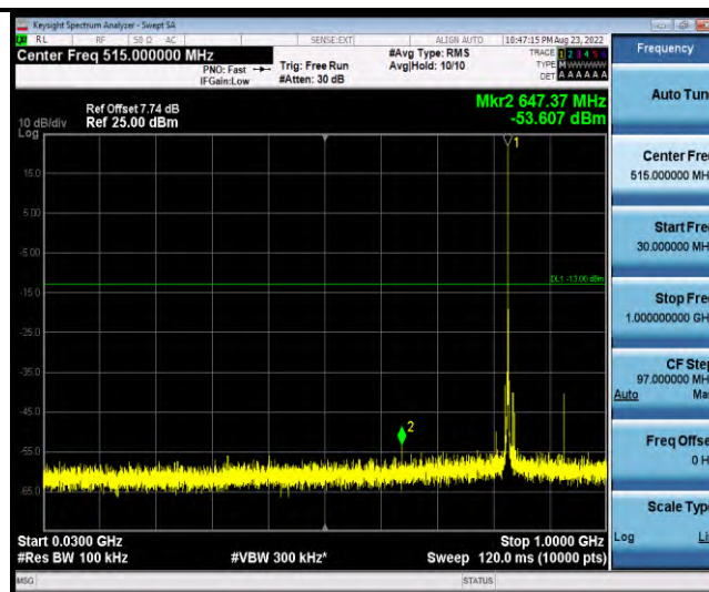
Band19-Stand-Alone-NaB-PSK-24002-1@0-15kHz-30-1000-30~1000MHz@-53.61dBm--13-PASS
