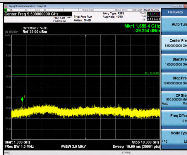
Band18-Stand-Alone-NaN-BPSK-23998-1@11-15kHz-1000-10000-1000~10000MHz@-39.25dBm--13-PASS
