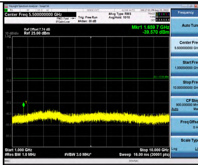
Band18-Stand-Alone-Na-N-BPSK-23998-1@0-15kHz-1000-10000-1000~10000MHz@-39.57dBm--13-PASS
