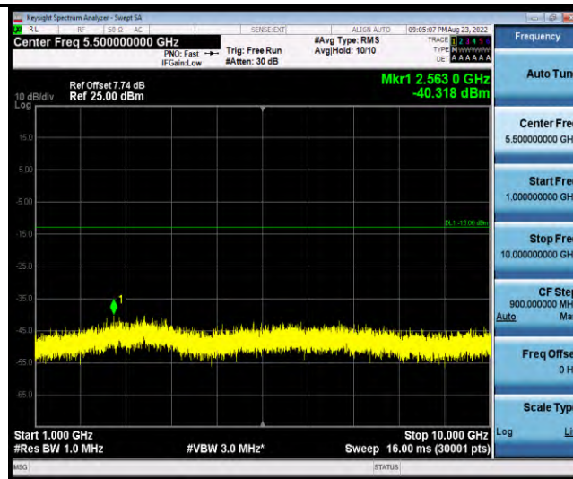
Band18-Stand-Alone-NaN-QPSK-23852-1@0-3.75kHz-1000-10000-1000~1000MHz@-40.32dBm--13-PASS
