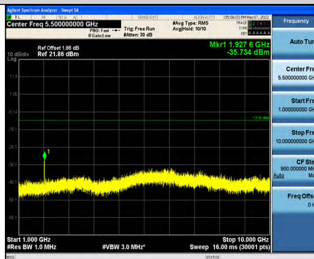
Band17-Stand-Alone-NaN-BPSK-23848-1@11-15kHz-1000-10000-1000~10000MHz@-35.73dBm--13-PASS
