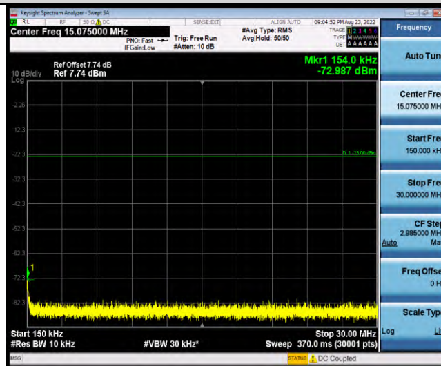
Band18-Stand-Alone-Na-N-QPSK-23852-1@0-3.75kHz-0.15-30-0.15-30MHz@-72.99dBm--23-PASS
