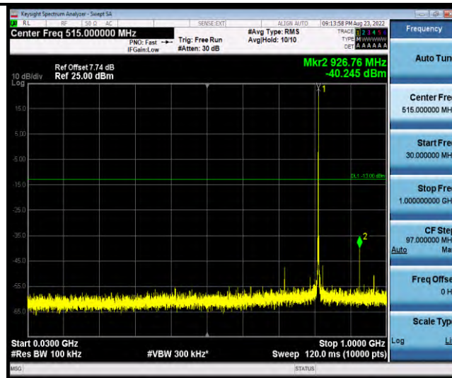
Band18-Stand-Alone-NaB-PSK-23852-1@0-15kHz-30-1000-30~1000MHz@-40.25dBm--13-PASS
