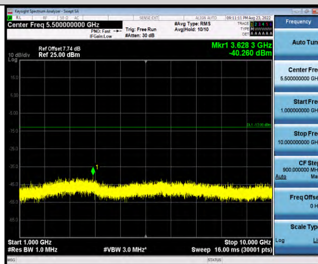
Band18-Stand-Alone-Na-N-QPSK-23852-12@0-15kHz-1000-10000-1000~10000MHz@-40.26dBm--13-PASS
