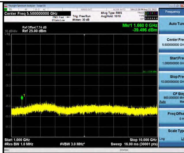
Band18-Stand-Alone-Na-N-QPSK-23998-12@0-15kHz-1000-10000-1000~10000MHz@-39.5dBm--13-PASS
