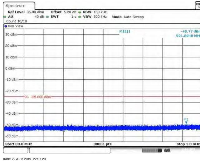
Band41_20MHz_64QAM_40640_1RB#0
