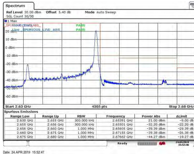
Band41_20MHz_64QAM_41140_100RB#0
