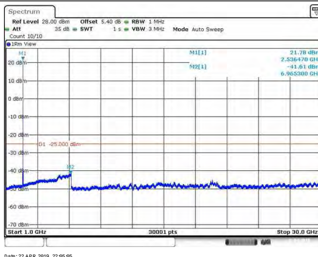
Band41_20MHz_16QAM_40640_1RB#0
