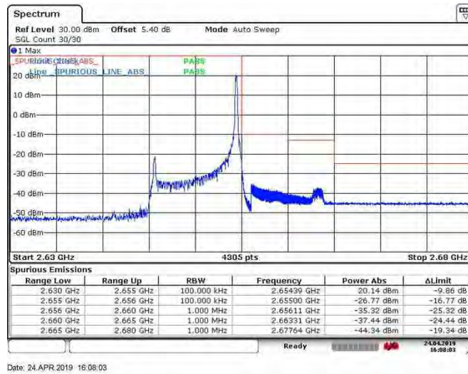
Band41_10MHz_16QAM_41190_50RB#0
