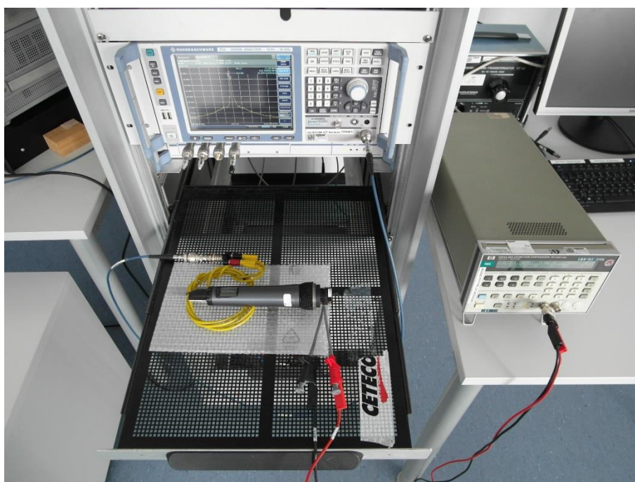
Photo 10: spectrum analyzer
