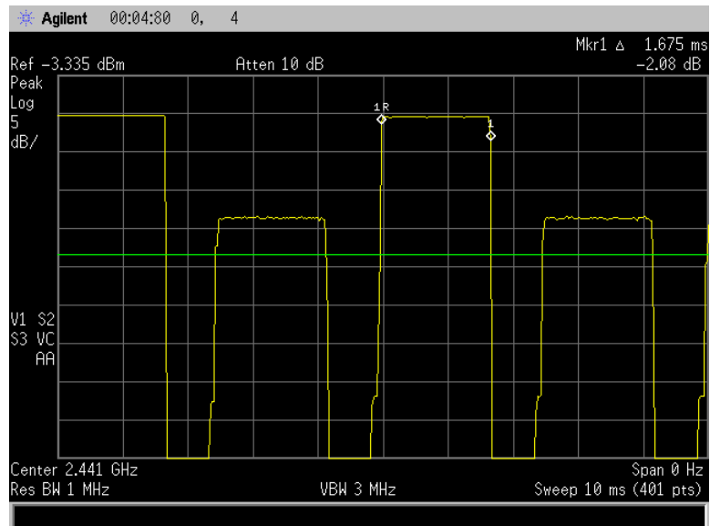
Figure 7.5.3.2-2: Channel Dwell Time – DH3
