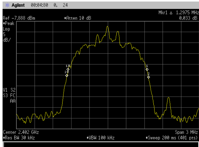
Figure 7.5.4.2-13: 20dB BW Low Channel (8DPSK)
