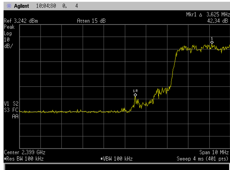
Figure 7.6.1.2-3: Lower Band-edge – Hopping Mode ( \pi/4 DQPSK)
