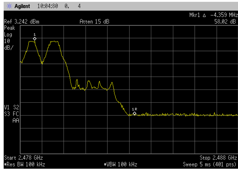
Figure 7.6.1.2-4: Upper Band-edge – Hopping Mode (GFSK)
