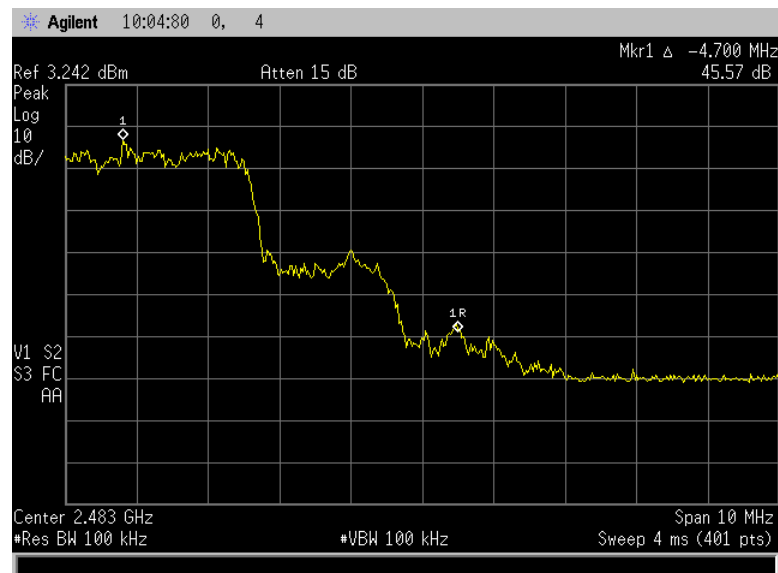
Figure 7.6.1.2-4: Upper Band-edge – Hopping Mode ( \pi/4 DQPSK)
