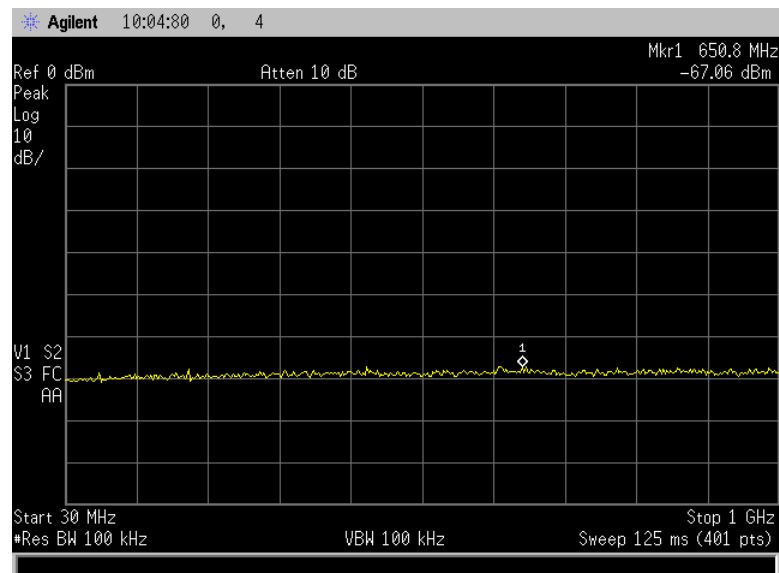
Figure 7.6.2.3-11: 30 MHz – 1 GHz – High Channel ( \pi/4 DQPSK)
