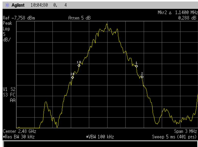
Figure 7.5.4.2-6: 99% OBW High Channel (GFSK)
