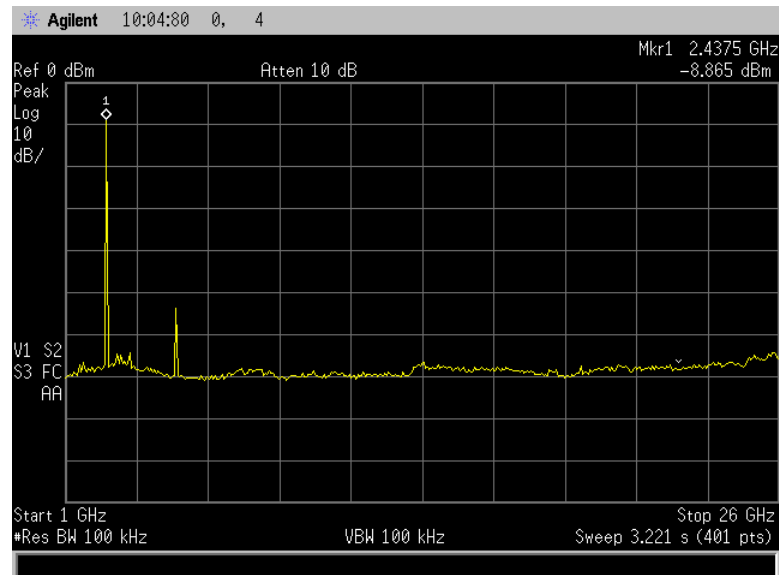
Figure 7.6.2.3-10: 1 GHz – 26.5 GHz – Mid Channel ( \pi/4 DQPSK)
