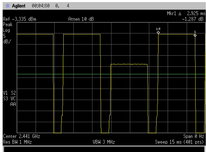
Figure 7.5.3.2-3: Channel Dwell Time – DH5
