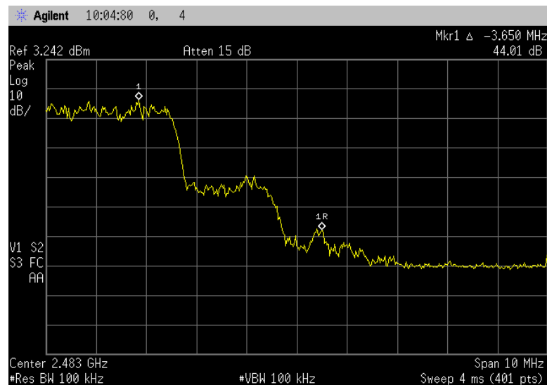
Figure 7.6.1.2-4: Upper Band-edge – Hopping Mode (8DPSK)
