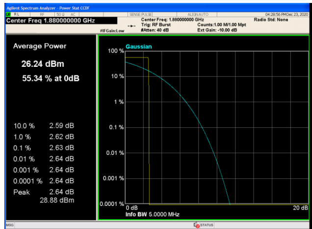
PCS 1900
