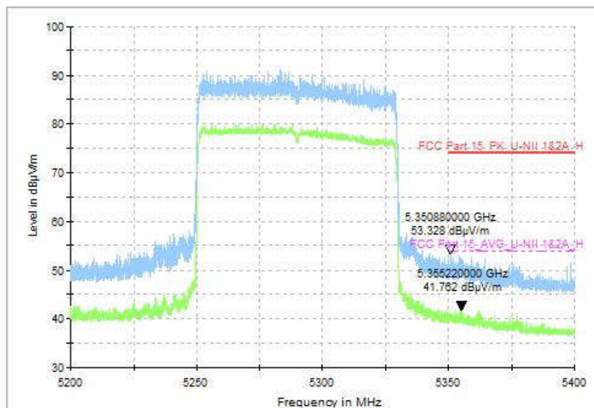
Fig. 80 Band Edges (802.11ax-HE80, CH58 5290MHz)
