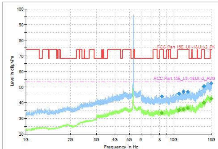
Fig. 124 Transmitter Spurious Emission (802.11ax-HE40, CH62 5310MHz, 1GHz-18GHz)
