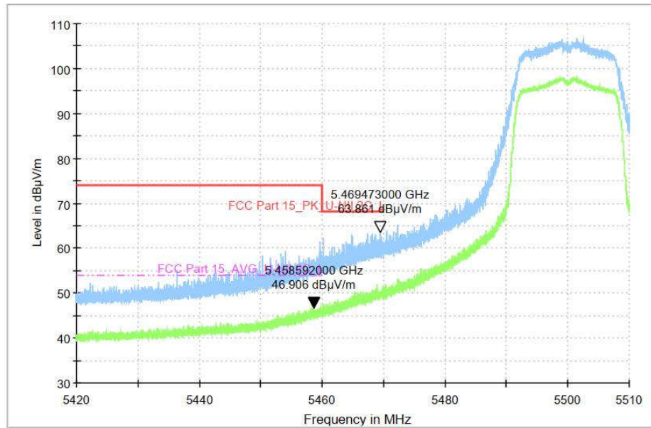
Fig. 69 Band Edges (802.11a, CH100 5500MHz)
