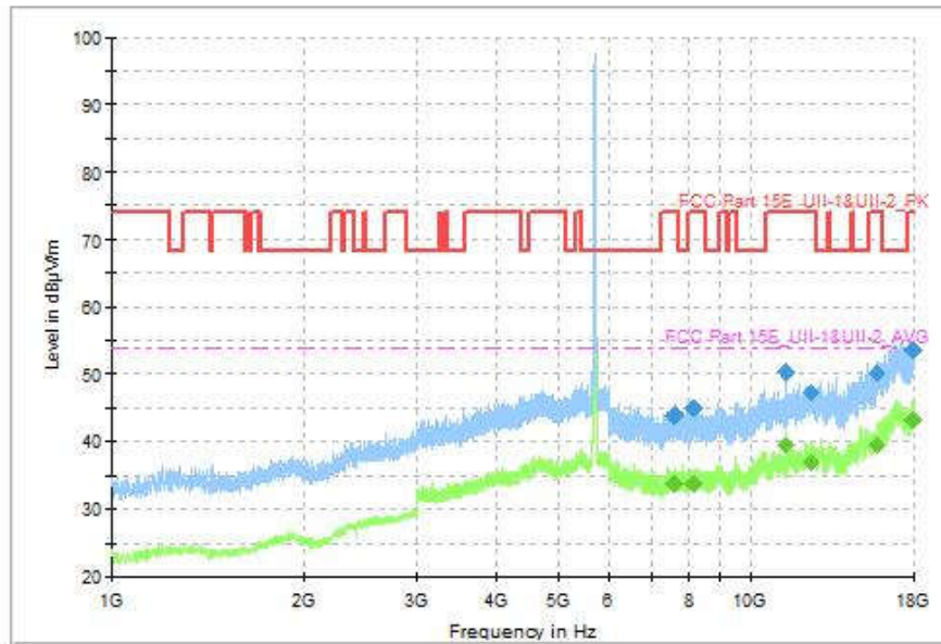
Fig. 117 Transmitter Spurious Emission (802.11a, CH140 5700MHz, 1GHz-18GHz)
