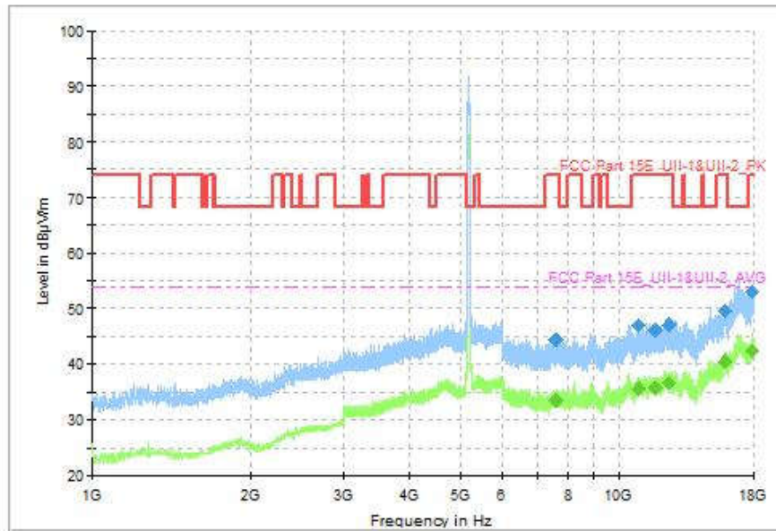
Fig. 121 Transmitter Spurious Emission (802.11ax-HE40, CH38 5190MHz, 1GHz-18GHz)
