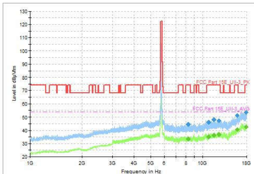
Fig. 128 Transmitter Spurious Emission (802.11ax-HE40, CH151 5755MHz, 1GHz-18GHz)
