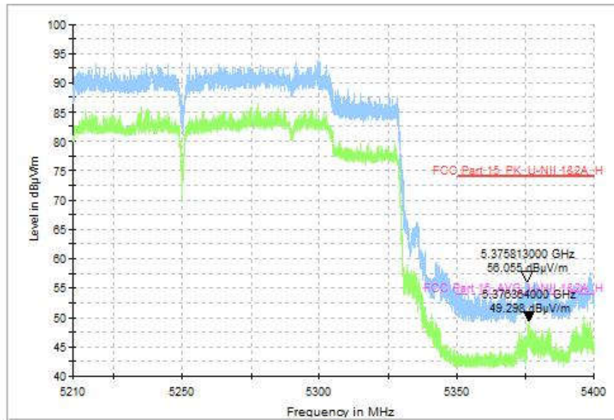
Fig. 85 Band Edges (802.11ax-HE160, CH50 5250MHz)
