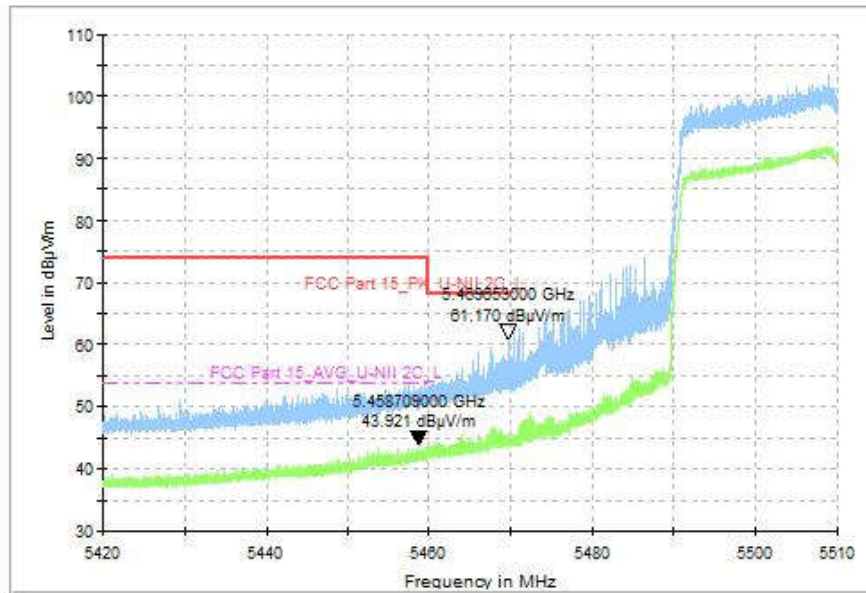
Fig. 75 Band Edges (802.11ax-HE40, CH102 5510MHz)
