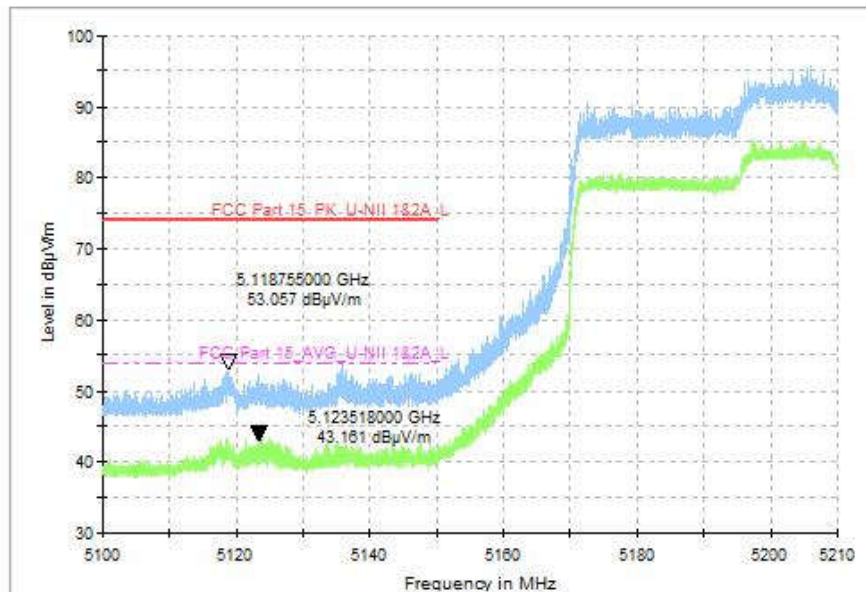
Fig. 84 Band Edges (802.11ax-HE160, CH50 5250MHz)
