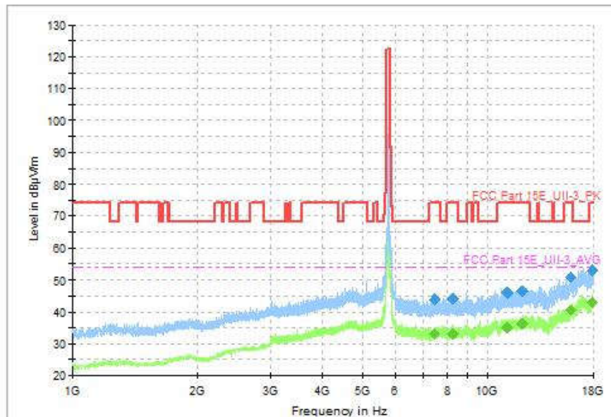
Fig. 134 Transmitter Spurious Emission (802.11ax-HE80, CH155 5775MHz, 1GHz-18GHz)
