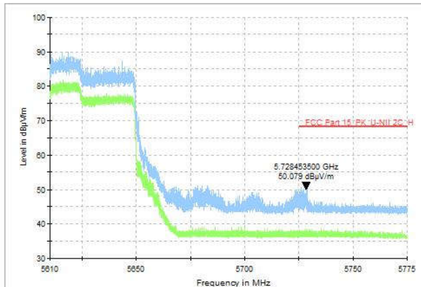
Fig. 108 Band Edges (802.11ax-HE160, CH114 5570MHz), MIMO
