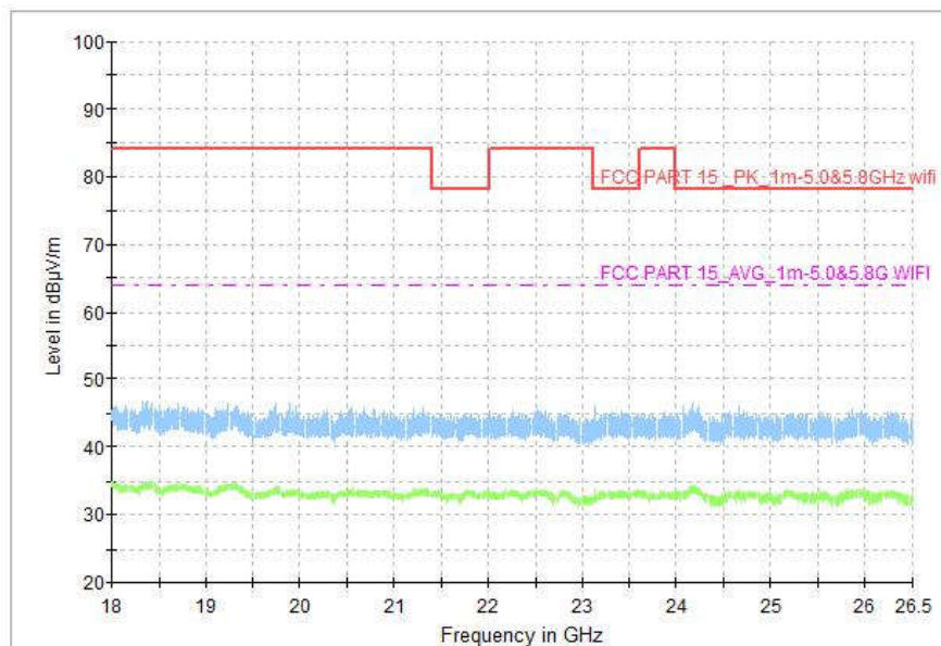
Fig. 138 Transmitter Spurious Emission (All channel, 18GHz~26.5GHz)
