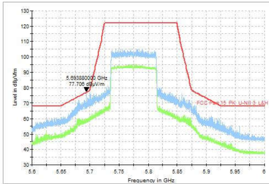
Fig. 83 Band Edges (802.11ax-HE80, CH155 5775MHz)
