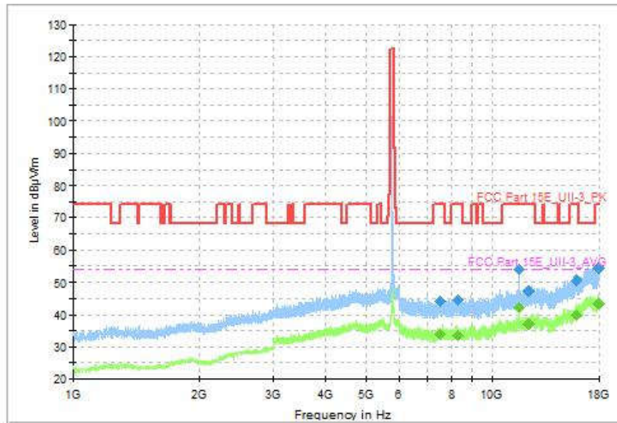
Fig. 119 Transmitter Spurious Emission (802.11a, CH157 5785MHz, 1GHz-18GHz)
