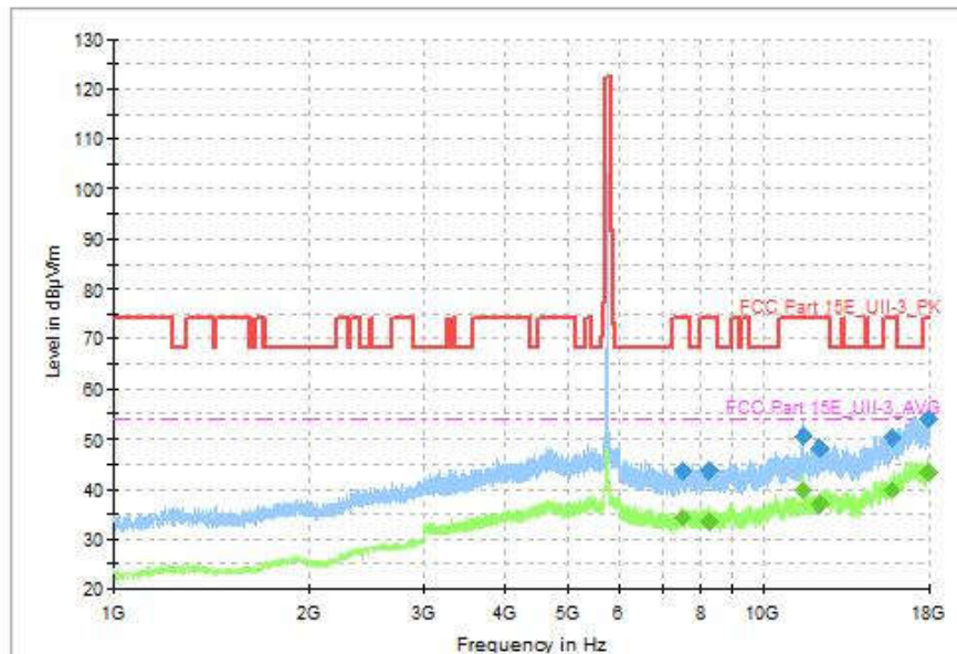
Fig. 118 Transmitter Spurious Emission (802.11a, CH149 5745MHz, 1GHz-18GHz)
