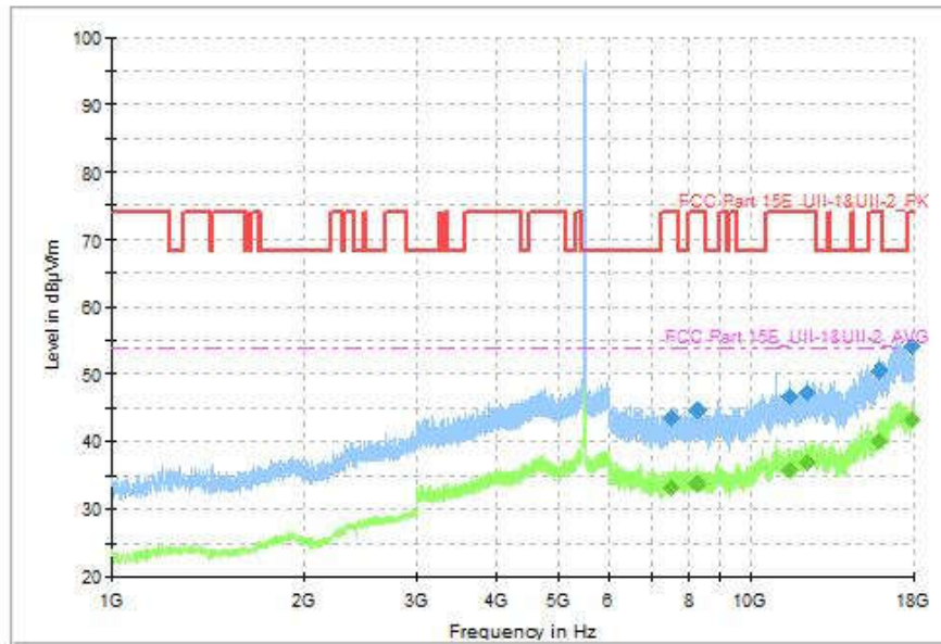
Fig. 115 Transmitter Spurious Emission (802.11a, CH100 5500MHz, 1GHz-18GHz)
