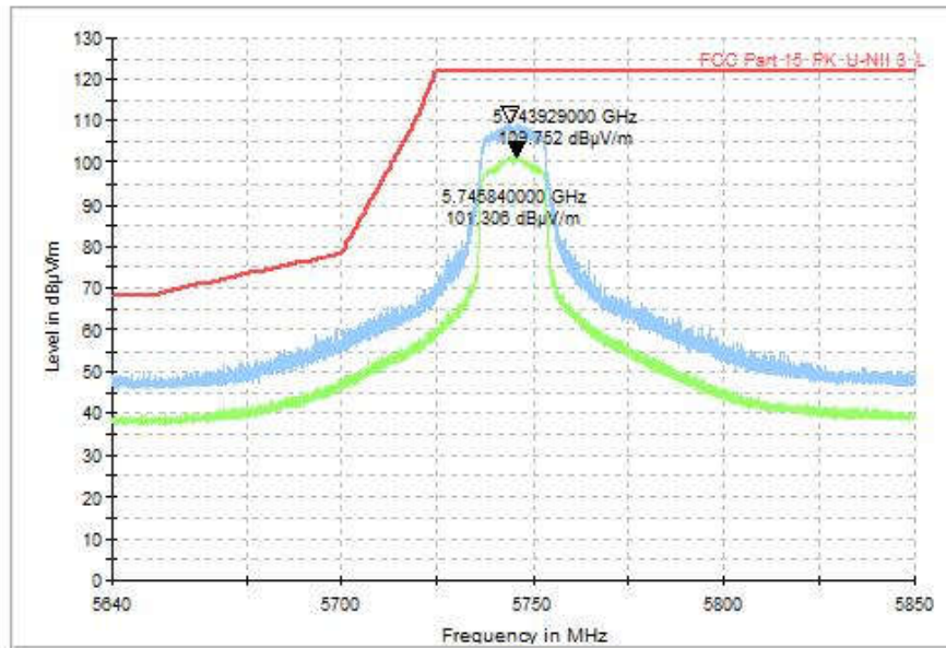
Fig. 71 Band Edges (802.11a, CH149 5745MHz)
