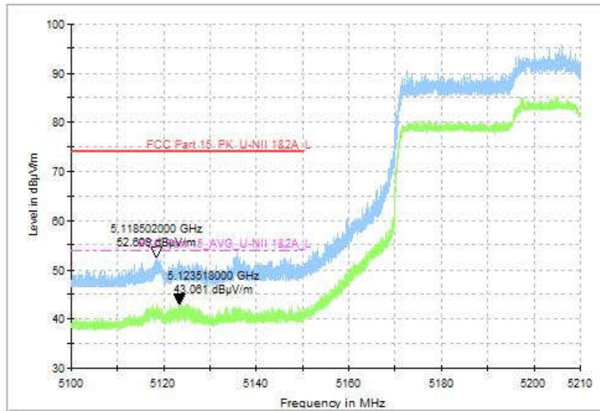
Fig. 105 Band Edges (802.11ax-HE160, CH50 5250MHz), MIMO
