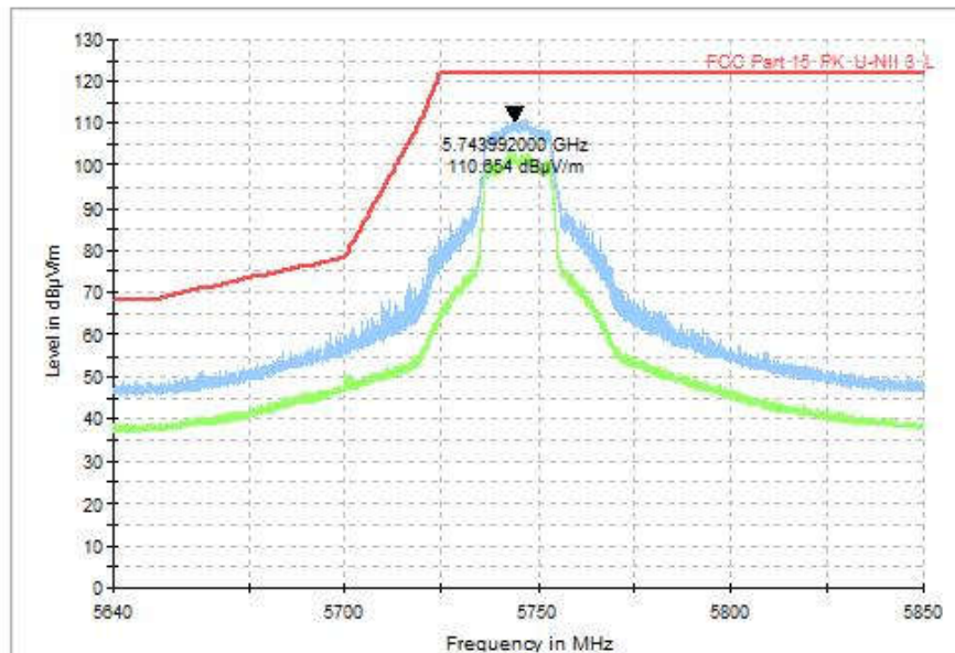
Fig. 92 Band Edges (802.11n-HT20, CH149 5745MHz), MIMO
