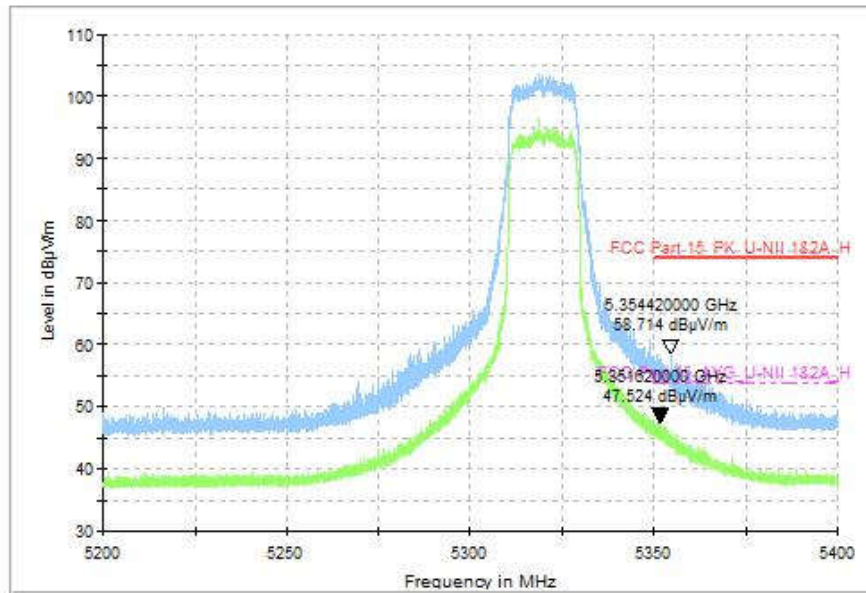
Fig. 89 Band Edges (802.11n-HT20, CH64 5320MHz), MIMO
