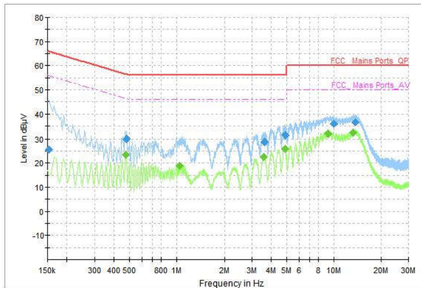
Fig. 174 AC Power line Conducted Emission (Idle)
