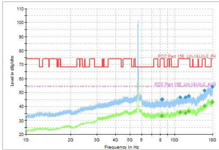
Fig. 127 Transmitter Spurious Emission (802.11ax-HE40, CH134 5670MHz, 1GHz-18GHz)
