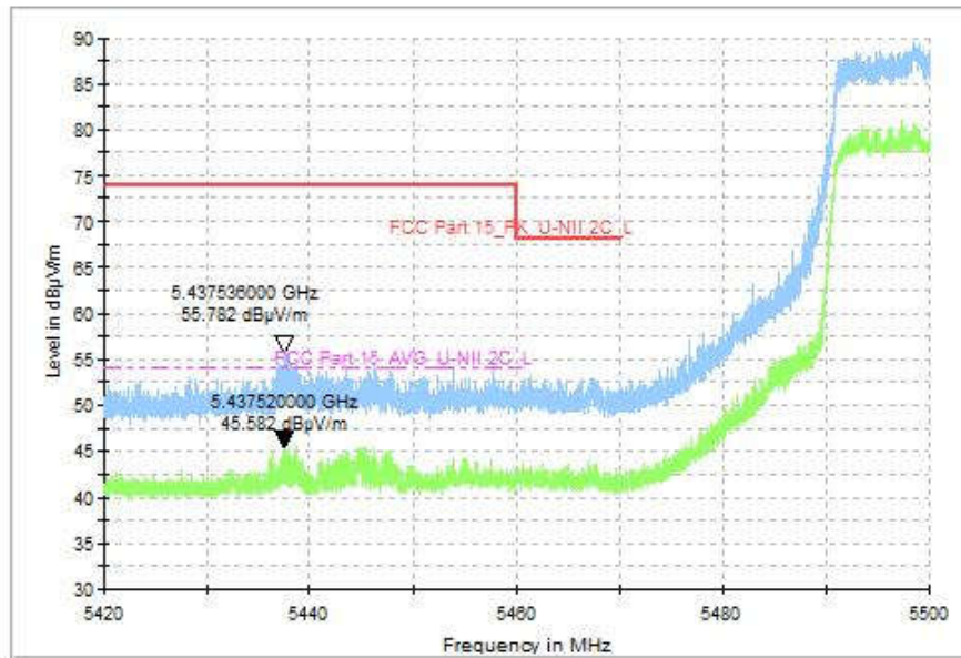
Fig. 107 Band Edges (802.11ax-HE160, CH114 5570MHz), MIMO
