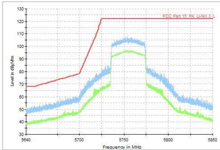
Fig. 77 Band Edges (802.11ax-HE40, CH151 5755MHz)
