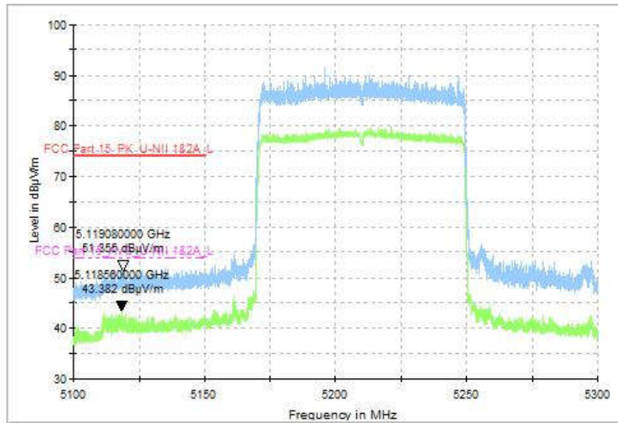
Fig. 79 Band Edges (802.11ax-HE80, CH42 5210MHz)
