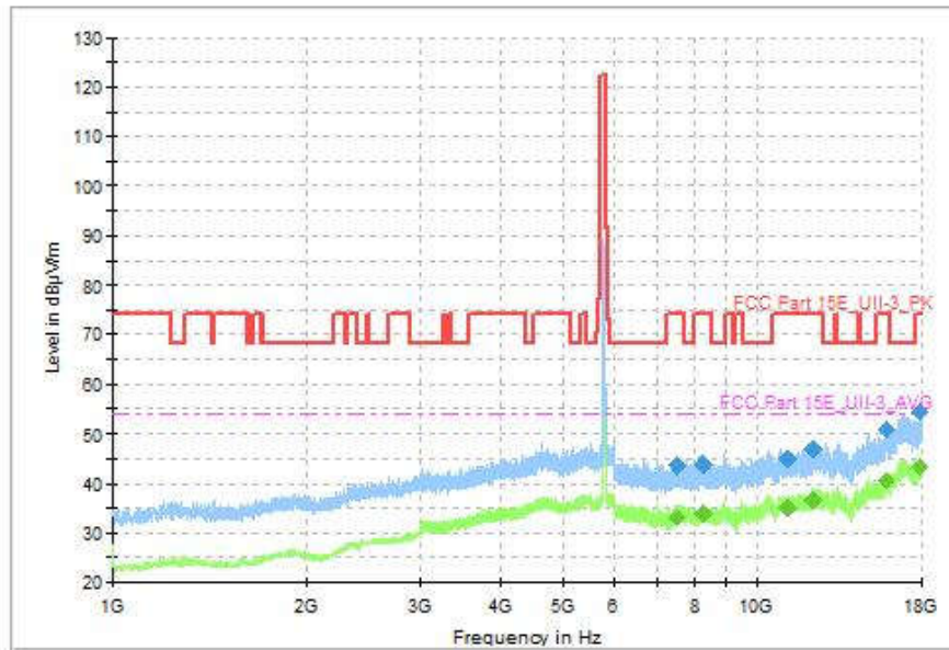
Fig. 129 Transmitter Spurious Emission (802.11ax-HE40, CH159 5795MHz, 1GHz-18GHz)
