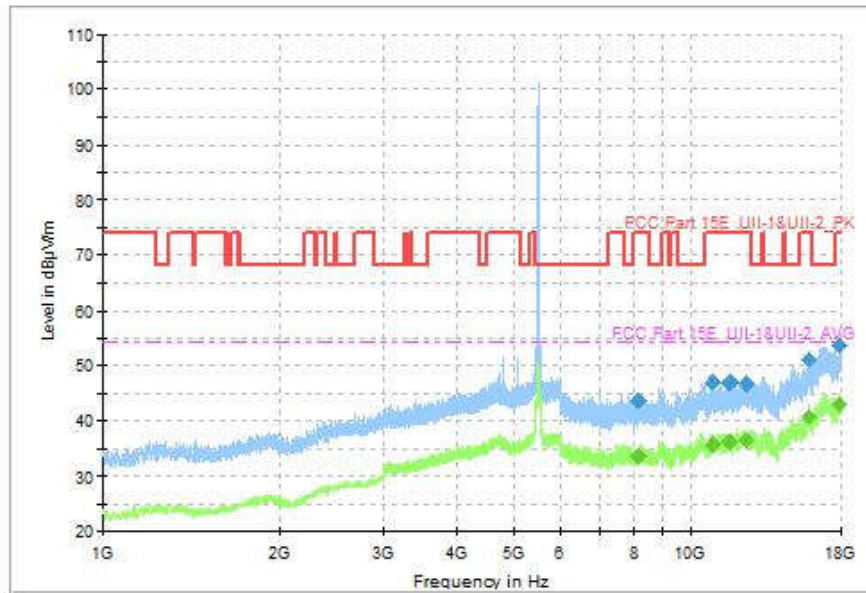
Fig. 125 Transmitter Spurious Emission (802.11ax-HE40, CH102 5510MHz, 1GHz-18GHz)
