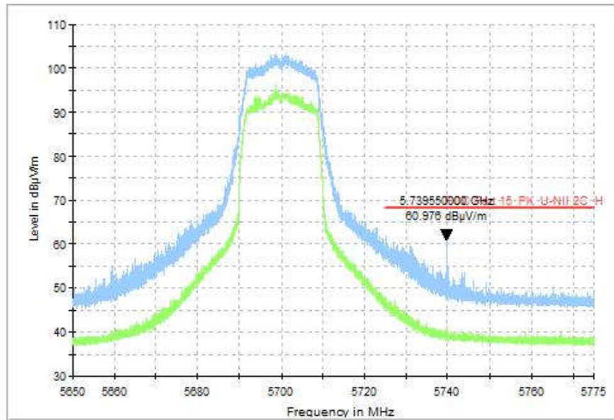
Fig. 91 Band Edges (802.11n-HT20, CH140 5700MHz), MIMO
