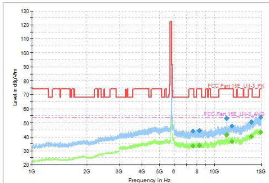
Fig. 120 Transmitter Spurious Emission (802.11a, CH165 5825MHz, 1GHz-18GHz)
