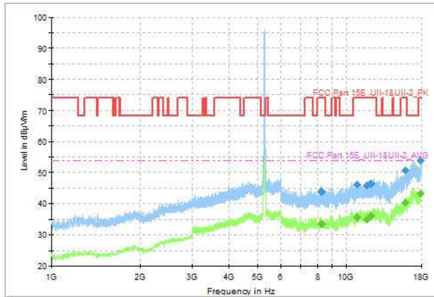
Fig. 123 Transmitter Spurious Emission (802.11ax-HE40, CH54 5270MHz, 1GHz-18GHz)
