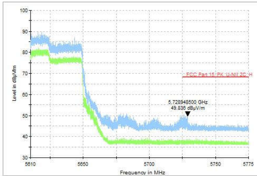
Fig. 87 Band Edges (802.11ax-HE160, CH114 5570MHz)
