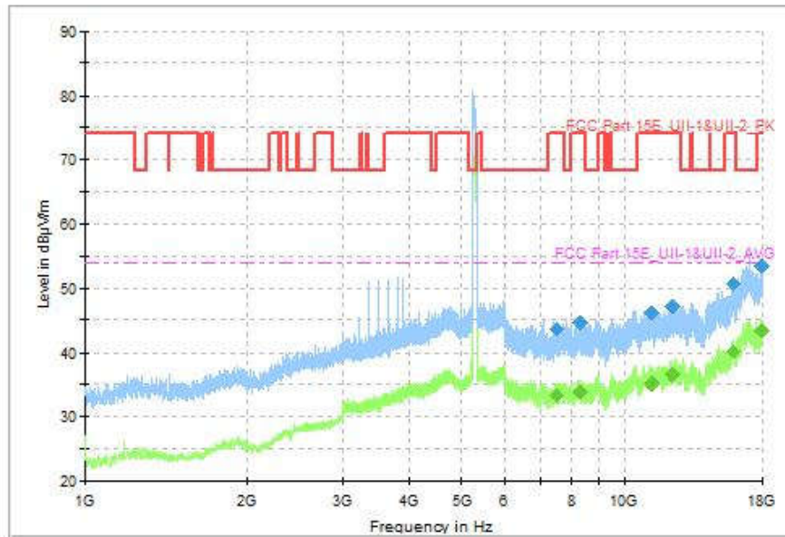
Fig. 131 Transmitter Spurious Emission (802.11ax-HE80, CH58 5290MHz, 1GHz-18GHz)
