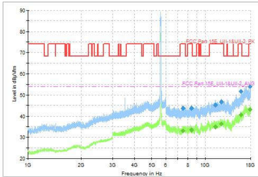
Fig. 133 Transmitter Spurious Emission (802.11ax-HE80, CH122 5610MHz, 1GHz-18GHz)
