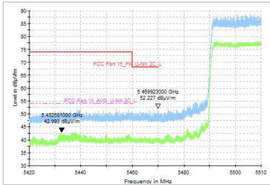
Fig. 81 Band Edges (802.11ax-HE80, CH106 5530MHz)
