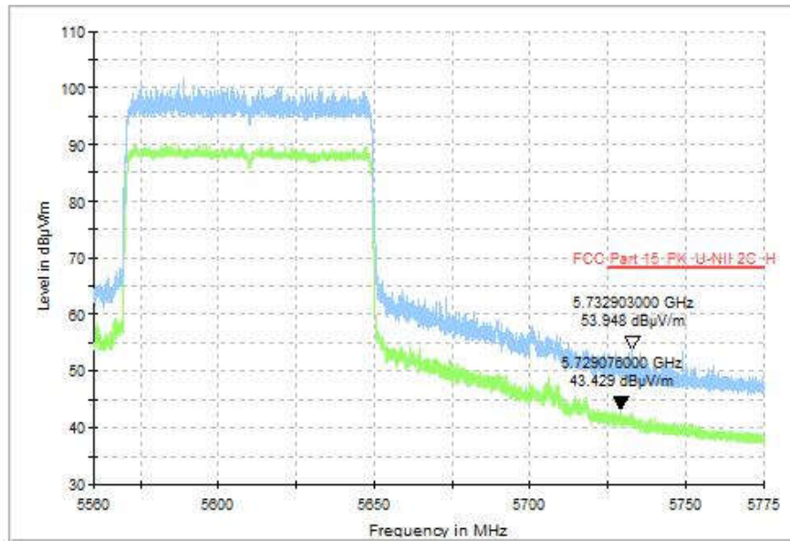
Fig. 103 Band Edges (802.11ax-HE80, CH122 5610MHz), MIMO
