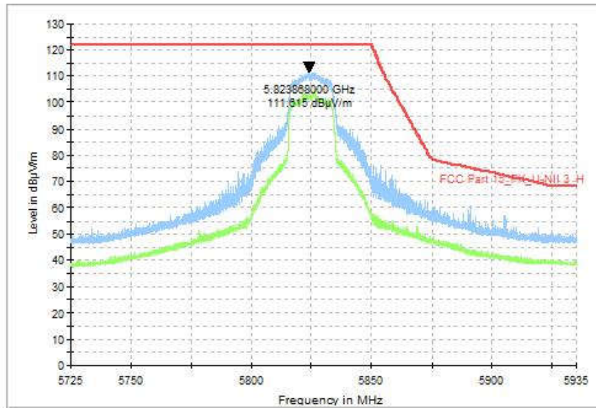
Fig. 93 Band Edges (802.11n-HT20, CH165 5825MHz), MIMO
