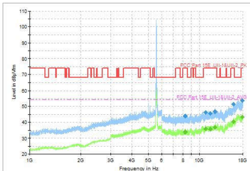
Fig. 126 Transmitter Spurious Emission (802.11ax-HE40, CH118 5580MHz, 1GHz-18GHz)
