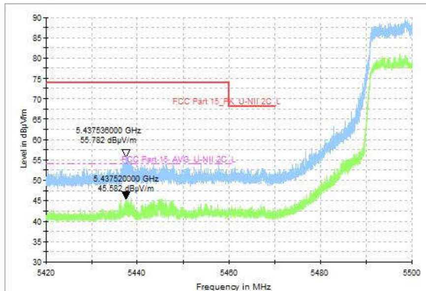
Fig. 86 Band Edges (802.11ax-HE160, CH114 5570MHz)
