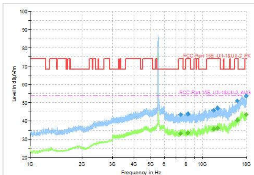
Fig. 132 Transmitter Spurious Emission (802.11ax-HE80, CH106 5530MHz, 1GHz-18GHz)
