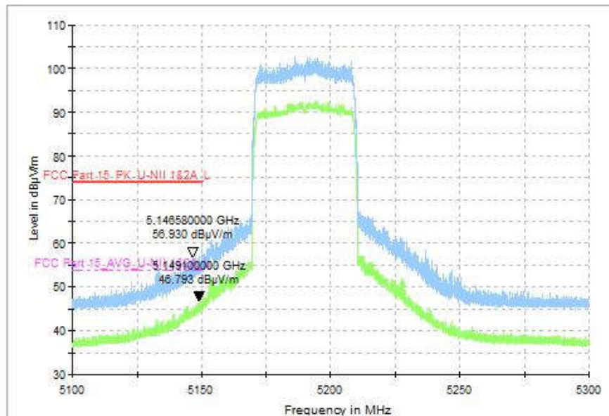
Fig. 94 Band Edges (802.11ax-HE40, CH38 5190MHz), MIMO
