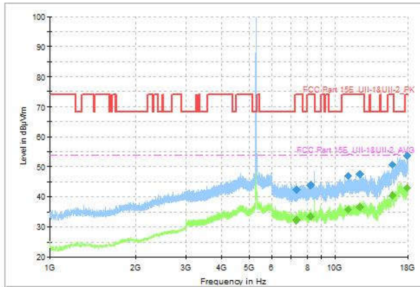
Fig. 113 Transmitter Spurious Emission (802.11a, CH56 5280MHz, 1GHz-18GHz)
