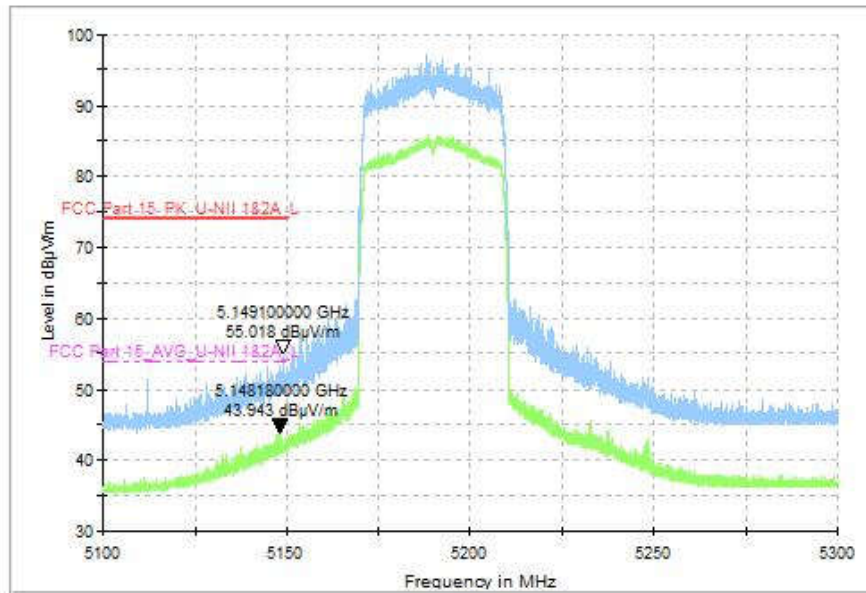
Fig. 73 Band Edges (802.11ax-HE40, CH38 5190MHz)
