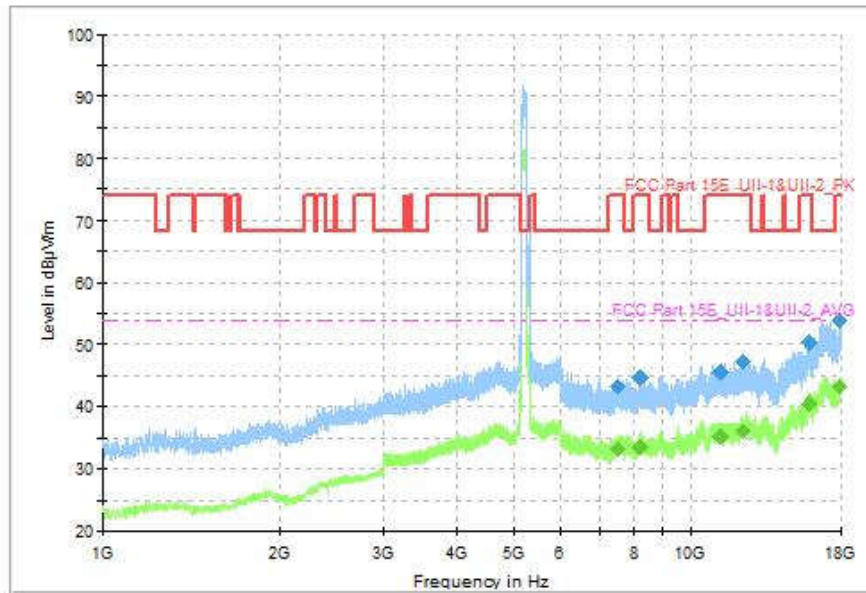
Fig. 135 Transmitter Spurious Emission (802.11ax-HE160, CH50 5250MHz, 1GHz-18GHz)
