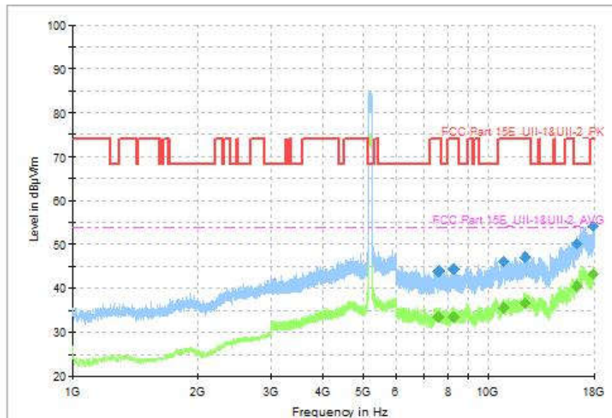
Fig. 130 Transmitter Spurious Emission (802.11ax-HE80, CH42 5210MHz, 1GHz-18GHz)
