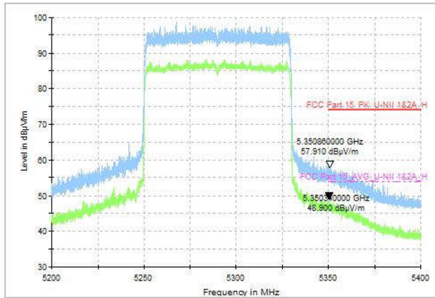
Fig. 101 Band Edges (802.11ax-HE80, CH58 5290MHz), MIMO
