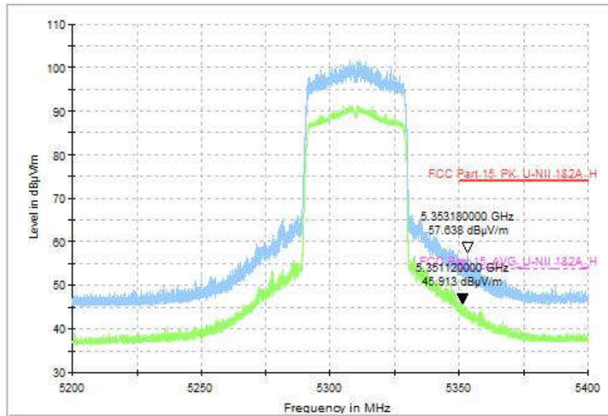
Fig. 95 Band Edges (802.11ax-HE40, CH62 5310MHz), MIMO
