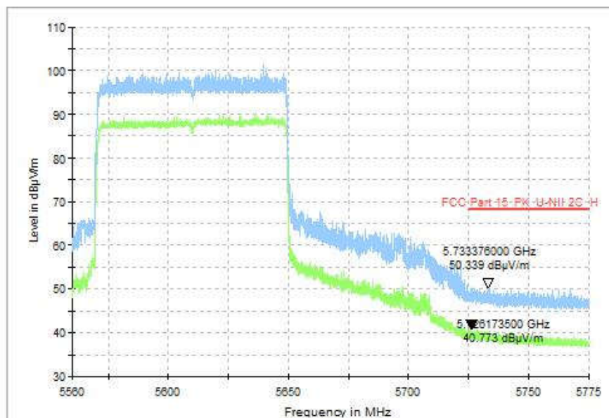
Fig. 82 Band Edges (802.11ax-HE80, CH122 5610MHz)
