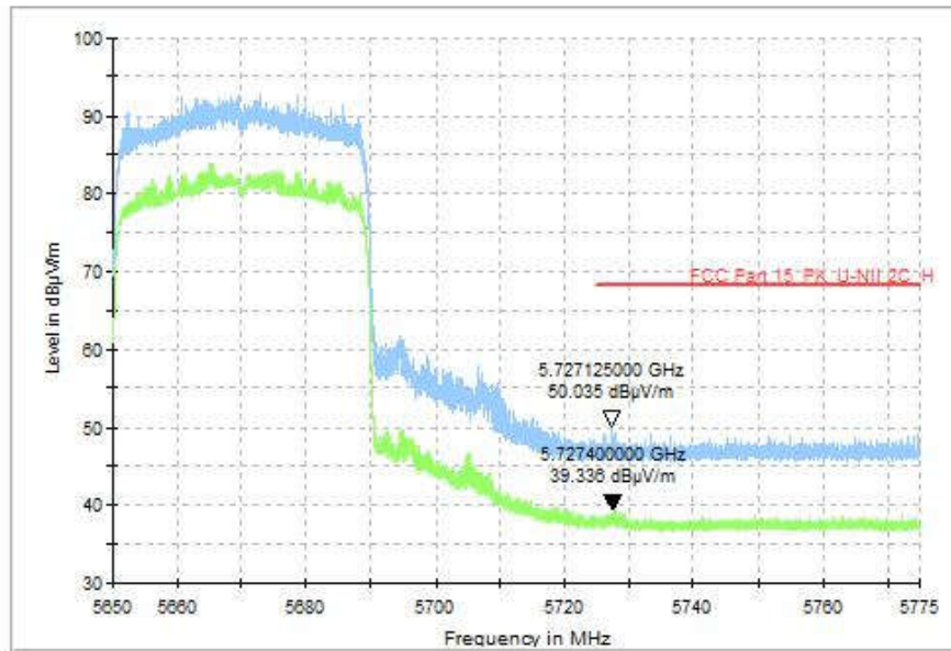
Fig. 97 Band Edges (802.11ax-HE40, CH134 5670MHz), MIMO
