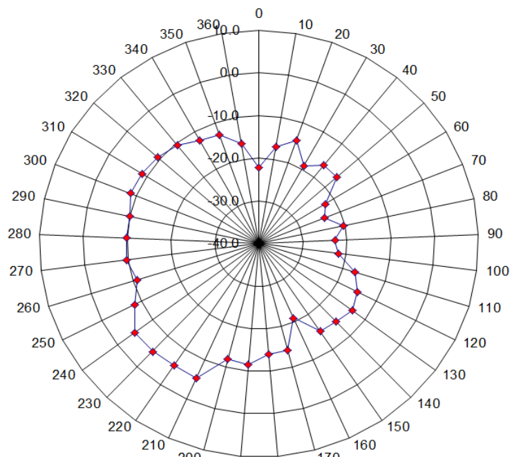
Vertical at 2405MHz
