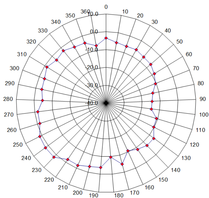
Horizontal at 2480MHz
