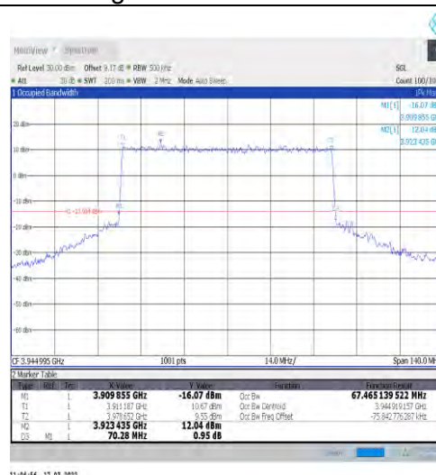
1-N77-3700-3980-30-70-H-7-CP-16QAM-Outer_Full- 189@0-Ant1-67.465-70.280-≤70-PASS
