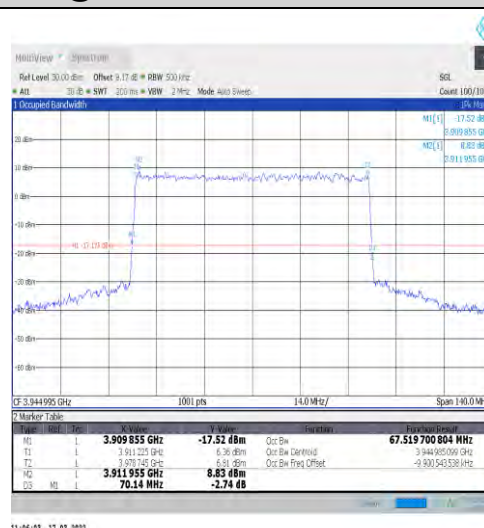
1-N77-3700-3980-30-70-H-9-CP-256QAM-Outer_Full I-189@0-Ant1-67.52-70.140-≤70-PASS
