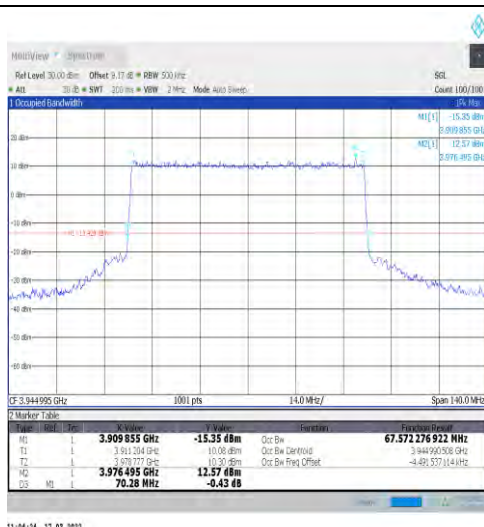
1-N77-3700-3980-30-70-H-6-CP-QPSK-Outer_Full-1 89@0-Ant1-67.572-70.280-≤70-PASS
