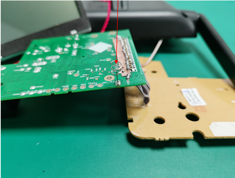
Bluetooth Antenna
