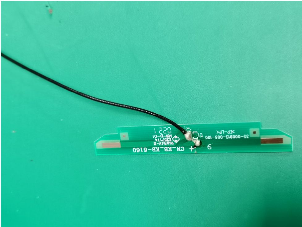
DECT Antenna 0
