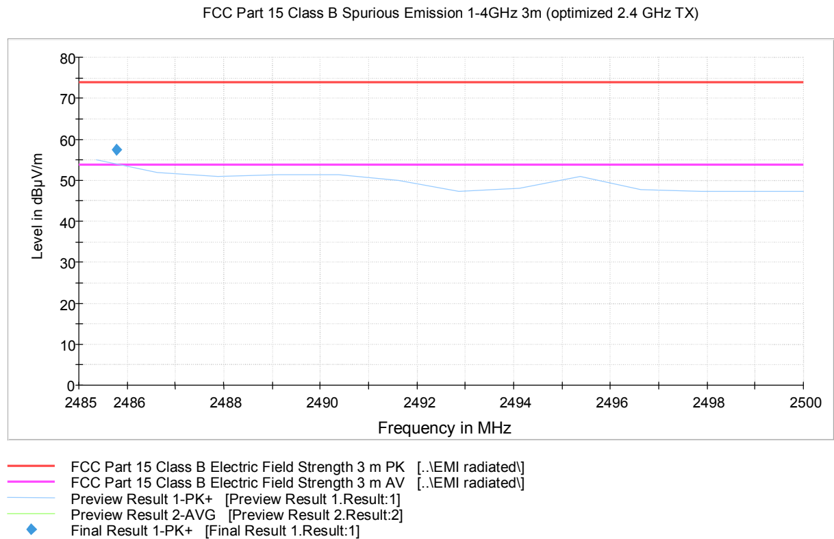
Figure 34. Radiated higher band edge measured with peak detector (WT11u-A)
