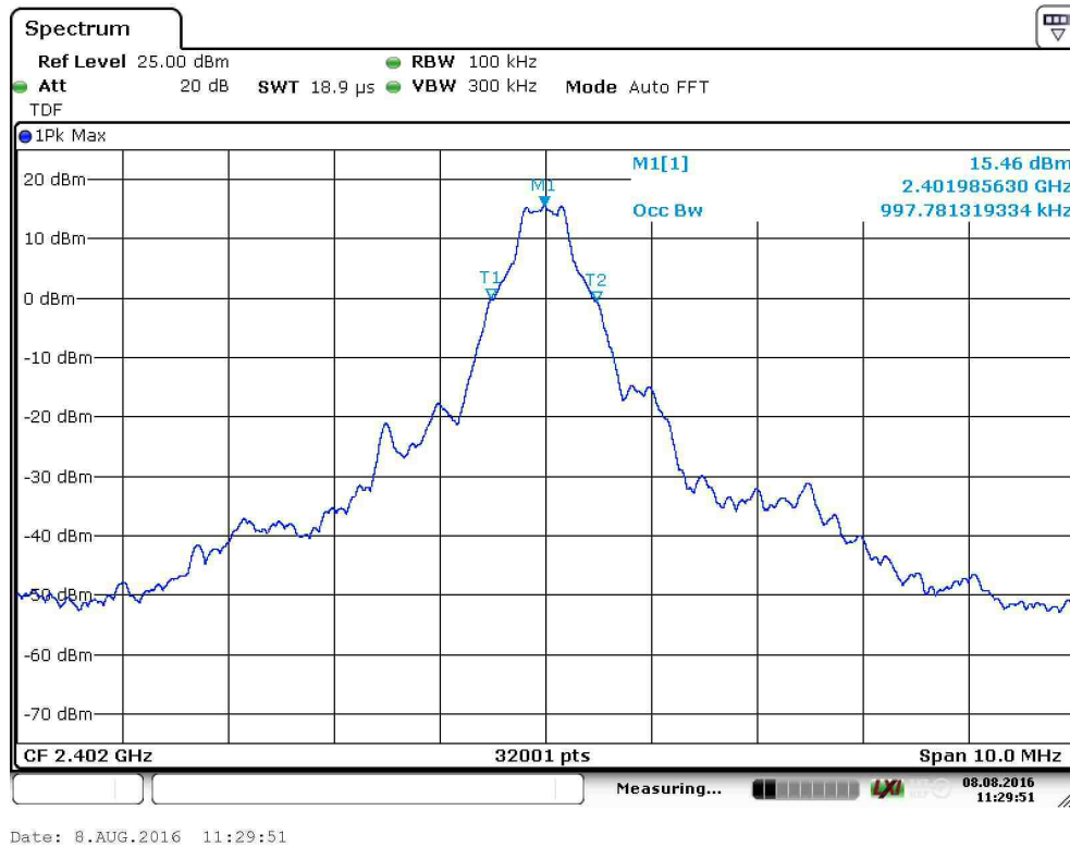
Figure 37. 99 % OBW channel low (1 Mbps).
