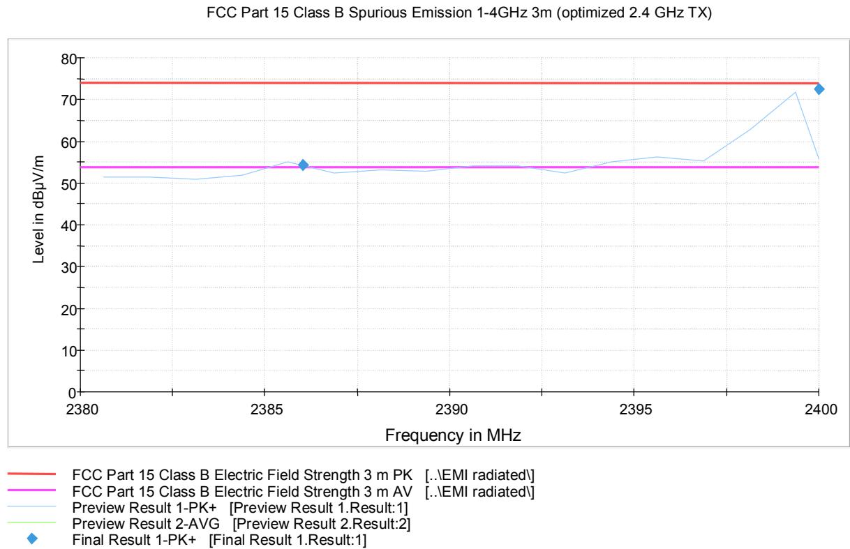
Figure 33. Radiated channel low band edge measured with peak detector (WT11u-A)
