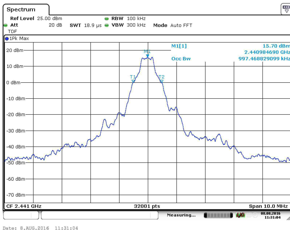
Figure 38. 99 % OBW channel mid (1 Mbps).
