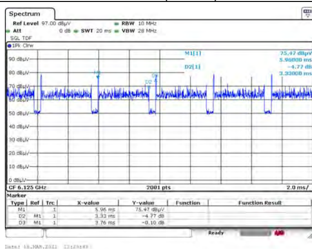
802.11ax (40MHz)
