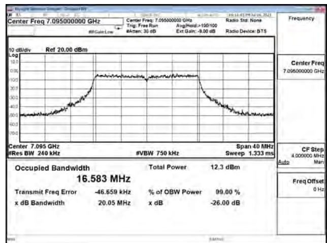
802.11a / Ant. 3 / 7095 MHz (U-NII-8)
