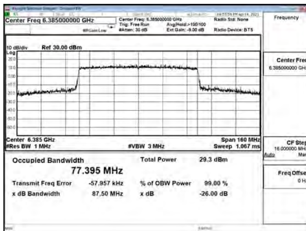
802.11ax (80MHz) / Ant. 1 / 6385 MHz (U-NII-5)
