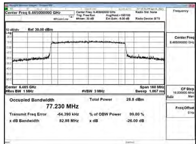
802.11ax (80MHz) / Ant. 1 / 6465 MHz (U-NII-6)
