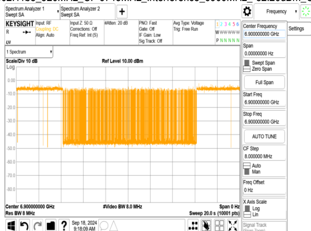
802.11be_320MHz_CF 6745MHz_Interference_6900MHz_-82.26dBm_ON
