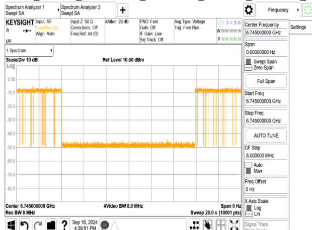
802.11be_320MHz_CF 6745MHz_Interference_6745MHz_-78.25dBm_Minimal
