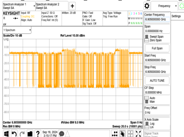
802.11be_320MHz_CF 6905MHz_Interference_6905MHz_-82.65dBm_ON
