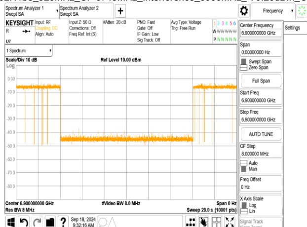
802.11be_320MHz_CF 6745MHz_Interference_6900MHz_-80.26dBm_Minimal
