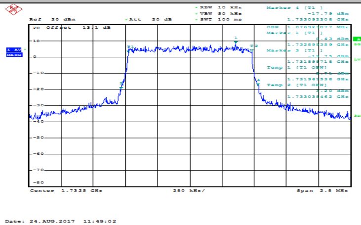
(Channel Bandwidth: 1.4 MHz)_MCH_16QAM_6RB#0
