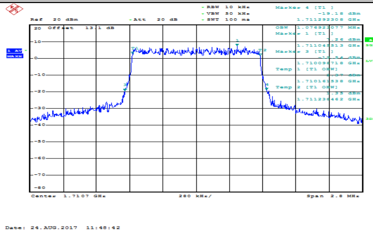
(Channel Bandwidth: 1.4 MHz)_LCH_16QAM_6RB#0
