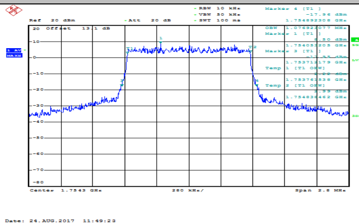
(Channel Bandwidth: 1.4 MHz)_HCH_16QAM_6RB#0
