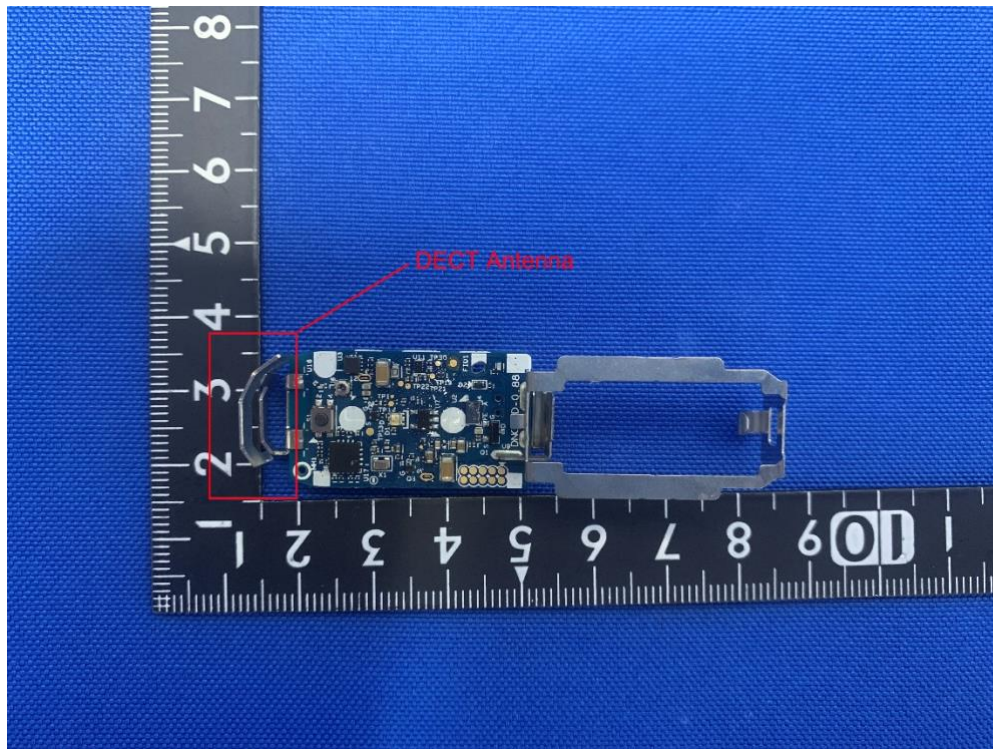
(7) EUT Photo – SSHX5R0-29
