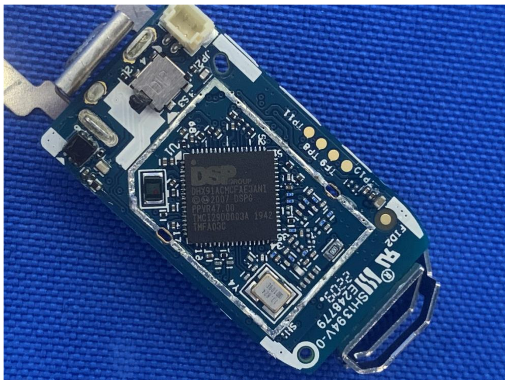
(8) EUT Photo – SSHX5R0-29
