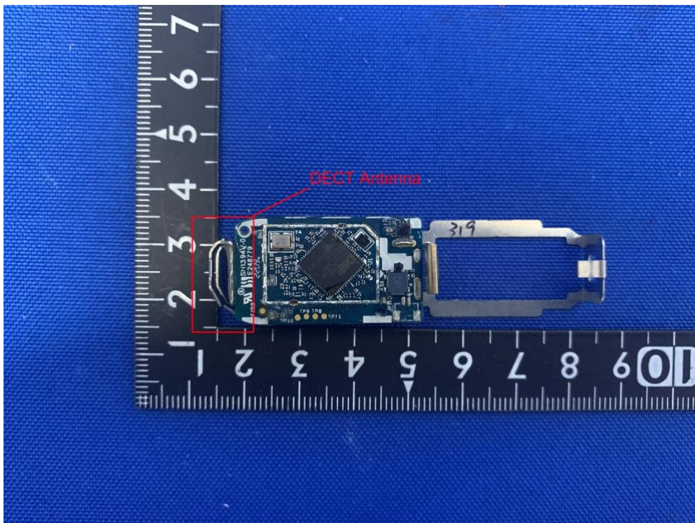
(16) EUT Photo – SSH5R0-29
