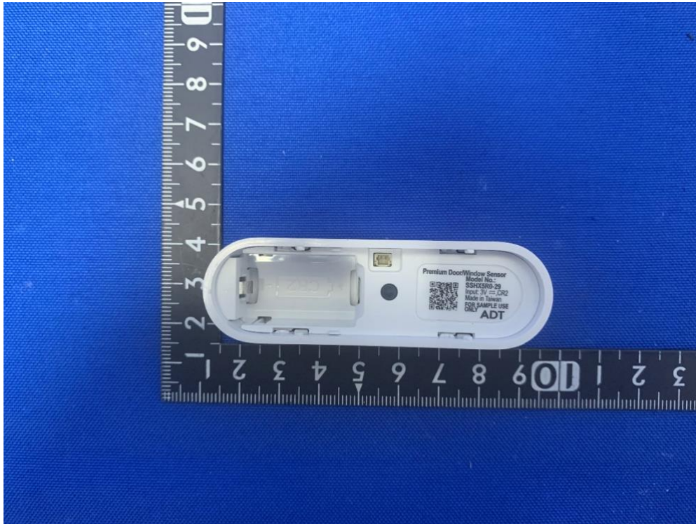
(4) EUT Photo – SSHX5R0-29
