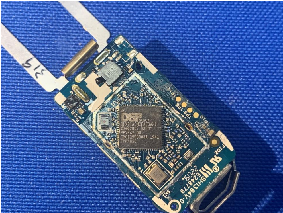
(17) EUT Photo – SSH5R0-29
