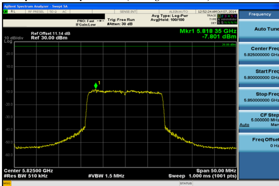
Peak Power Spectral Density Data Plot (CH High 5825 MHz)
