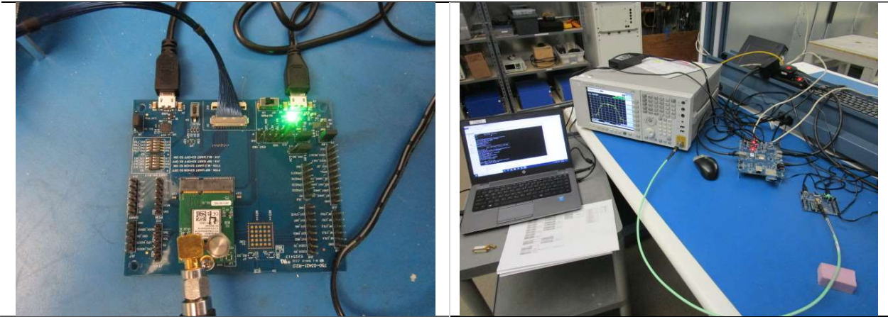
Conducted RF Setup Photos
