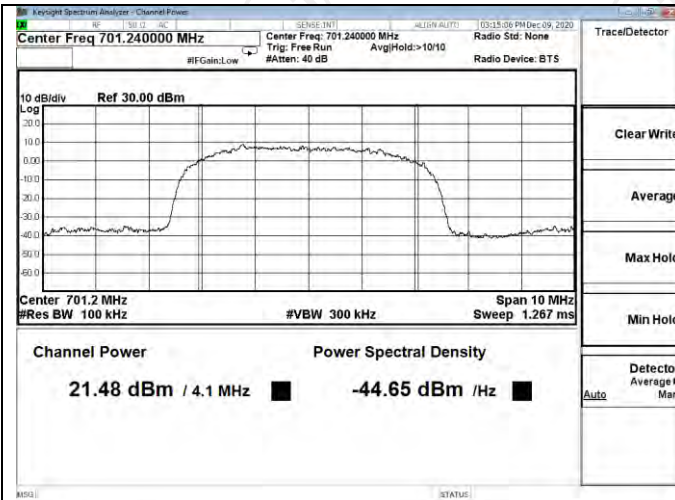
Uplink, AWGN, Above-AGC, Output Power
