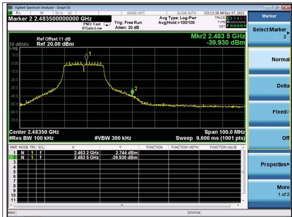
(Band Edge, Channel 11, 802.11n (HT20))
