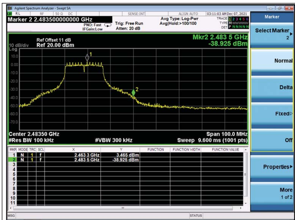
(Band Edge, Channel 11, 802.11g)
