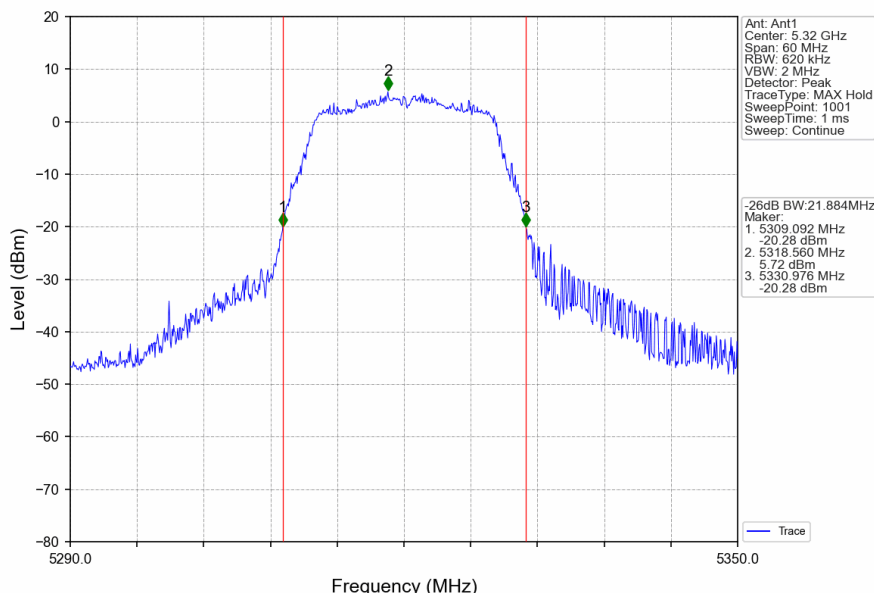
802.11a_HCH_5320MHz_Ant1_NTNV
