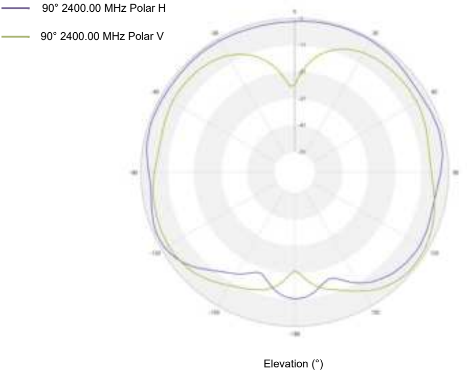
Figure 2-18. Antenna Radiation Elevated Plane Pattern @ \Phi = 90^\circ
