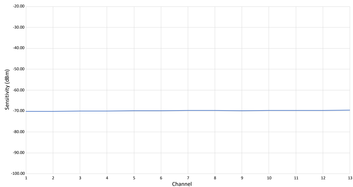
Figure 3-12. RX Sensitivity vs Channel, MCS7, 3.3V, 25°C
