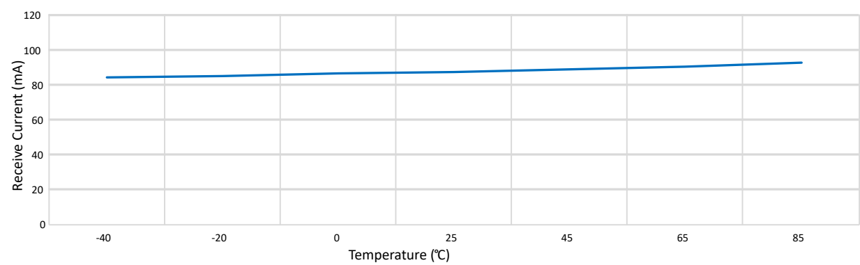
Figure 3-4. Receive Current vs Temperature, MCS7, Channel 7, 3.3V
