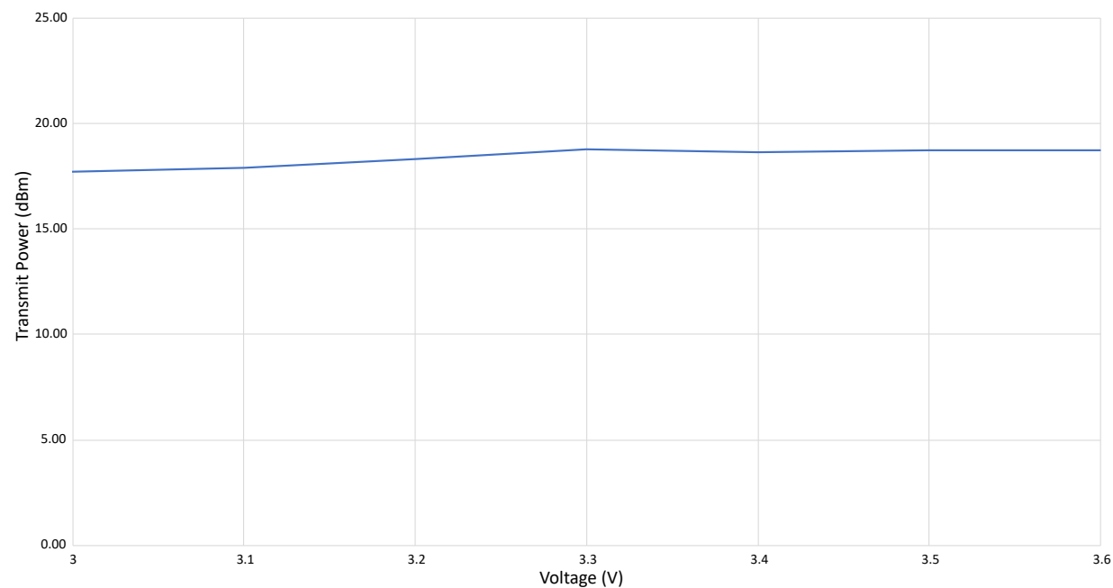
Figure 3-8. Transmit Power vs Voltage, 1M, Channel 7, 3.3V, 25°C
