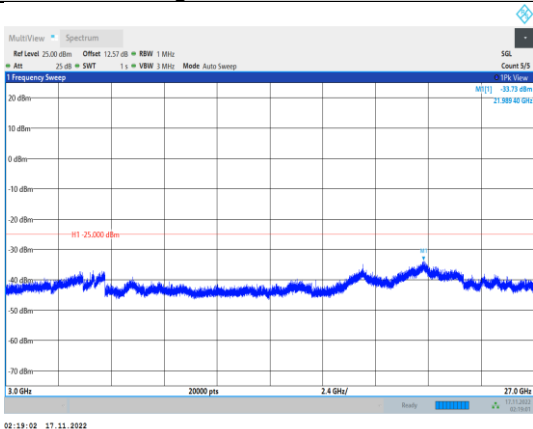
Band41-5MHz-64QAM-41215-1RB#0- Range3:3000~27000MHz
