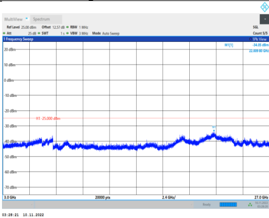
Band41-10MHz-16QAM-40090-1RB#0- Range3:3000~27000MHz
