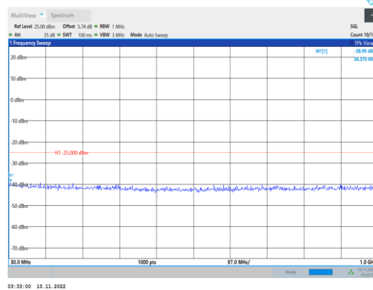
Band41-5MHz-16QAM-40065-1RB#0- Range1:30~1000MHz
