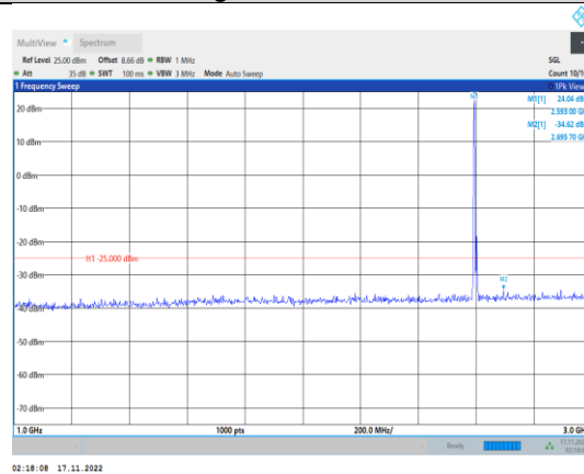
Band41-5MHz-64QAM-40640-1RB#0- Range2:1000~3000MHz
