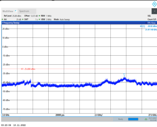
Band41-15MHz-QPSK-40115-1RB#0- Range3:3000~27000MHz
