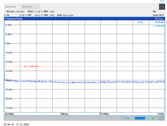
Band38-20MHz-64QAM-37850-1RB#0- Range1:30~1000MHz
