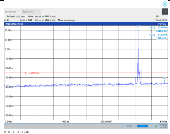
Band41-20MHz-64QAM-41140-1RB#0- Range2:1000~3000MHz
