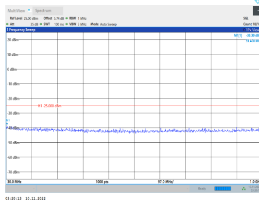
Band41-20MHz-16QAM-40640-1RB#0- Range1:30~1000MHz
