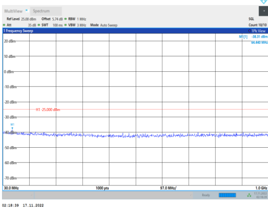
Band41-5MHz-64QAM-41215-1RB#0- Range1:30~1000MHz
