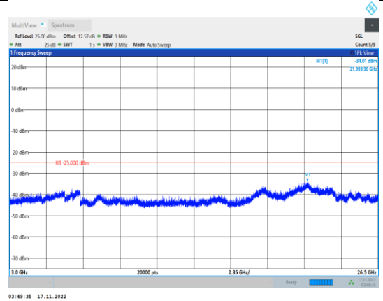
Band38-20MHz-64QAM-37850-1RB#0- Range3:3000~26500MHz
