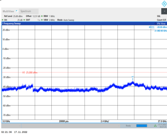
Band41-15MHz-64QAM-41165-1RB#0- Range3:3000~27000MHz
