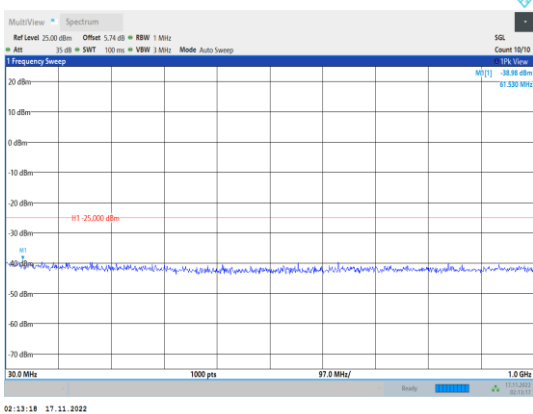
Band41-10MHz-64QAM-40640-1RB#0- Range1:30~1000MHz
