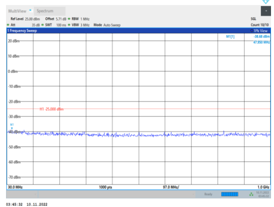
Band38-20MHz-QPSK-38150-1RB#0- Range1:30~1000MHz
