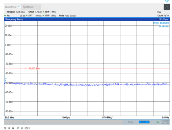
Band41-10MHz-64QAM-40090-1RB#0- Range1:30~1000MHz
