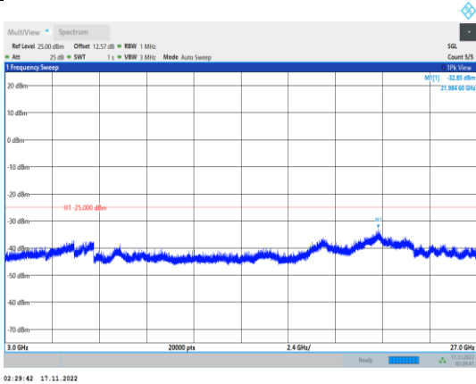
Band41-20MHz-64QAM-40640-1RB#0- Range3:3000~27000MHz
