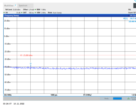
Band41-15MHz-QPSK-40640-1RB#0- Range1:30~1000MHz
