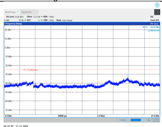
Band41-10MHz-64QAM-40090-1RB#0- Range3:3000~27000MHz
