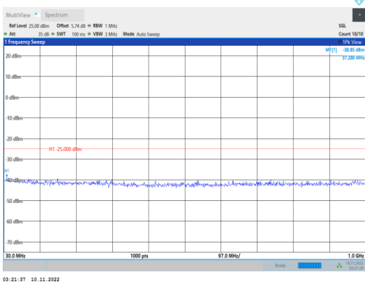
Band41-20MHz-16QAM-41140-1RB#0- Range1:30~1000MHz
