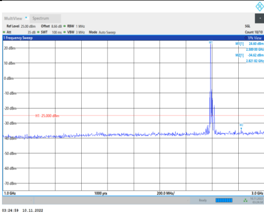
Band41-15MHz-16QAM-40640-1RB#0- Range2:1000~3000MHz
