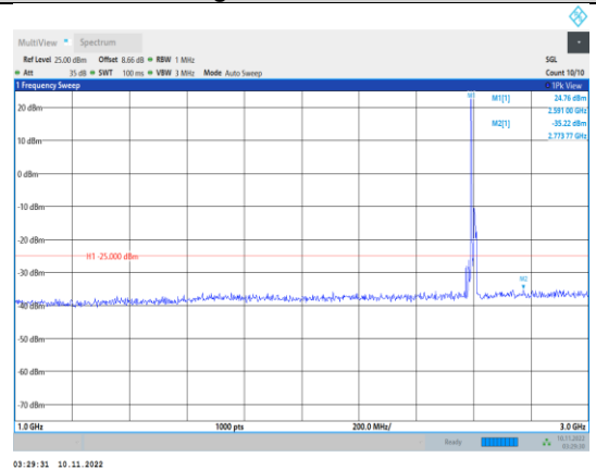
Band41-10MHz-16QAM-40640-1RB#0- Range2:1000~3000MHz
