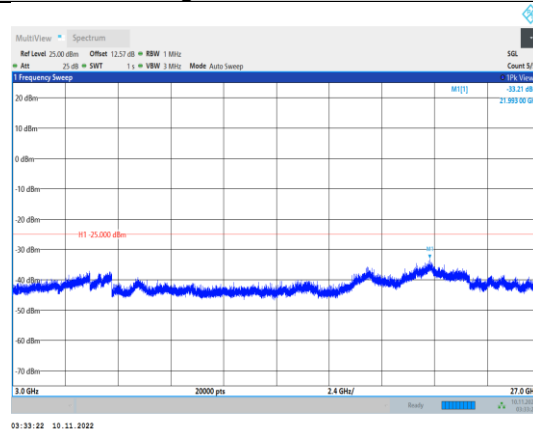
Band41-5MHz-16QAM-40065-1RB#0- Range3:3000~27000MHz
