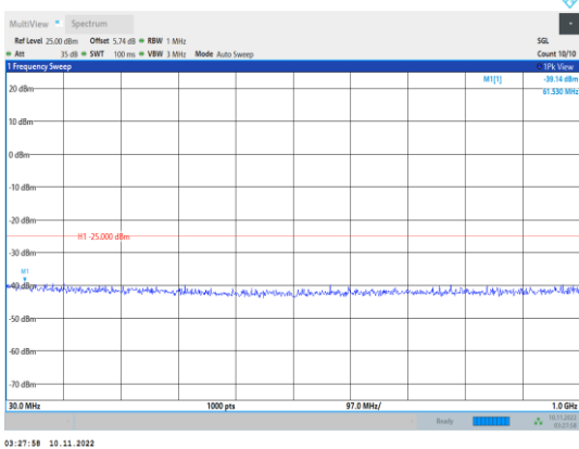
Band41-10MHz-16QAM-40090-1RB#0- Range1:30~1000MHz
