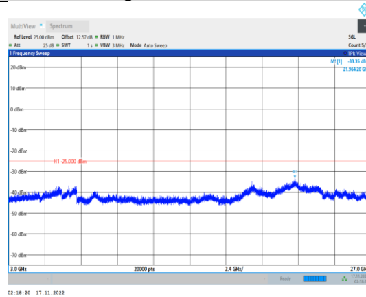
Band41-5MHz-64QAM-40640-1RB#0- Range3:3000~27000MHz
