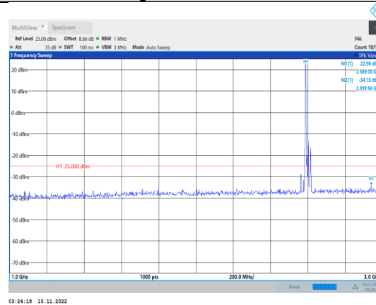
Band41-15MHz-QPSK-40640-1RB#0- Range2:1000~3000MHz
