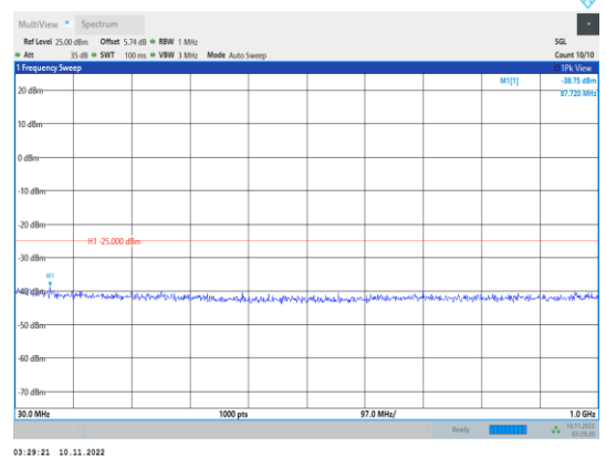
Band41-10MHz-16QAM-40640-1RB#0- Range1:30~1000MHz
