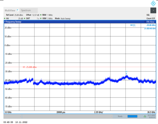
Band38-20MHz-QPSK-38150-1RB#0- Range3:3000~26500MHz
