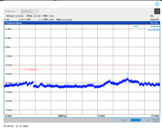
Band41-10MHz-16QAM-40640-1RB#0- Range3:3000~27000MHz
