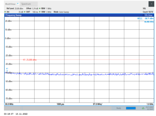
Band41-20MHz-QPSK-40140-1RB#0- Range1:30~1000MHz
