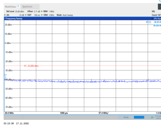
Band38-15MHz-64QAM-38000-1RB#0- Range1:30~1000MHz
