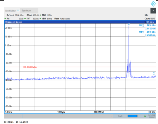
Band41-15MHz-16QAM-41165-1RB#0- Range2:1000~3000MHz
