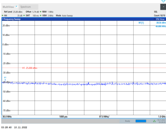
Band41-10MHz-QPSK-40640-1RB#0- Range1:30~1000MHz
