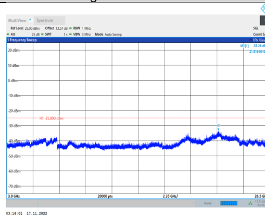
Band38-15MHz-64QAM-38000-1RB#0- Range3:3000~26500MHz
