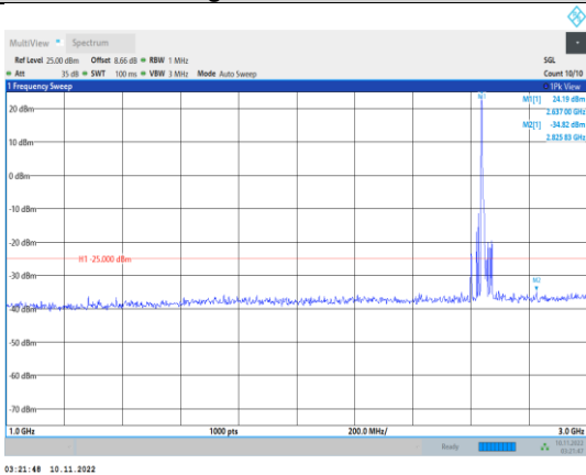
Band41-20MHz-16QAM-41140-1RB#0- Range2:1000~3000MHz
