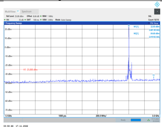
Band38-20MHz-64QAM-38150-1RB#0- Range2:1000~3000MHz
