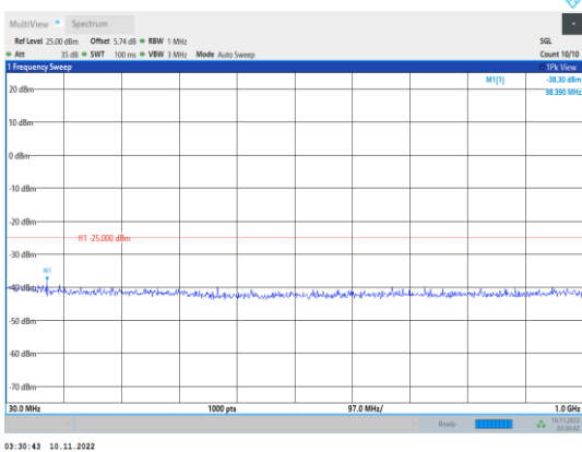
Band41-10MHz-16QAM-41190-1RB#0- Range1:30~1000MHz
