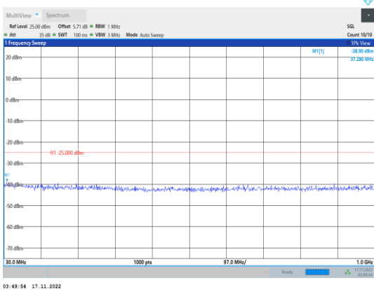
Band38-20MHz-64QAM-38000-1RB#0- Range1:30~1000MHz
