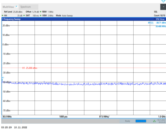
Band41-15MHz-QPSK-41165-1RB#0- Range1:30~1000MHz
