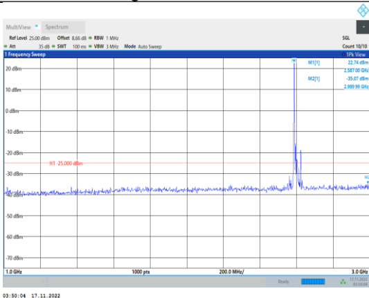
Band38-20MHz-64QAM-38000-1RB#0- Range2:1000~3000MHz
