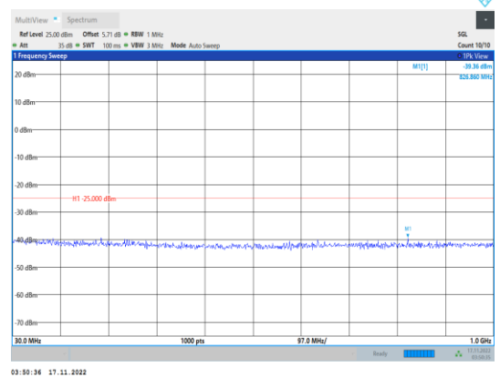
Band38-20MHz-64QAM-38150-1RB#0- Range1:30~1000MHz
