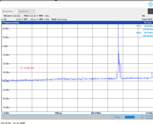
Band41-20MHz-16QAM-40140-1RB#0- Range2:1000~3000MHz
