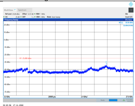
Band41-15MHz-64QAM-40640-1RB#0- Range3:3000~27000MHz
