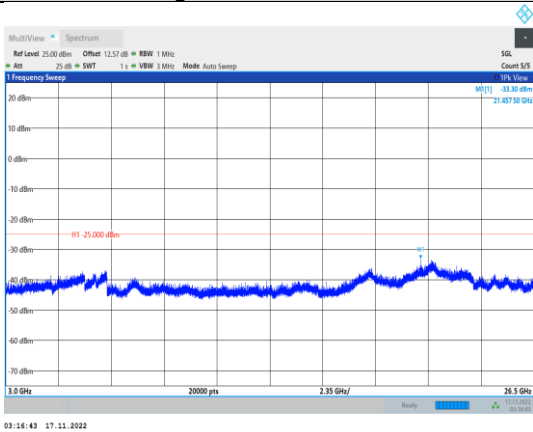
Band38-15MHz-64QAM-38175-1RB#0- Range3:3000~26500MHz
