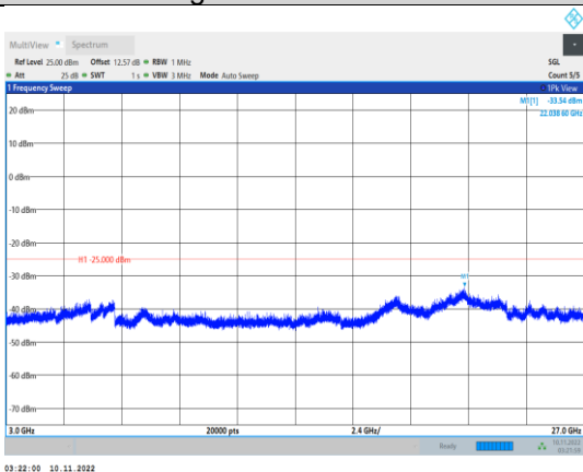
Band41-20MHz-16QAM-41140-1RB#0- Range3:3000~27000MHz
