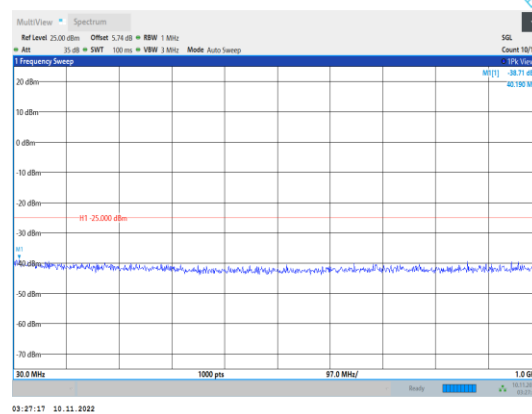
Band41-10MHz-QPSK-40090-1RB#0- Range1:30~1000MHz
