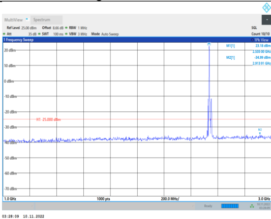
Band41-10MHz-16QAM-40090-1RB#0- Range2:1000~3000MHz
