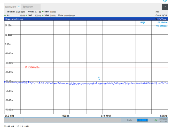
Band38-20MHz-QPSK-37850-1RB#0- Range1:30~1000MHz
