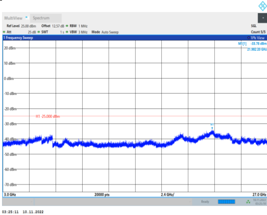
Band41-15MHz-16QAM-40640-1RB#0- Range3:3000~27000MHz
