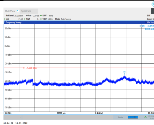
Band41-15MHz-QPSK-40640-1RB#0- Range3:3000~27000MHz
