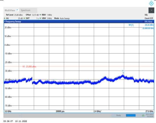
Band41-5MHz-16QAM-41215-1RB#0- Range3:3000~27000MHz
