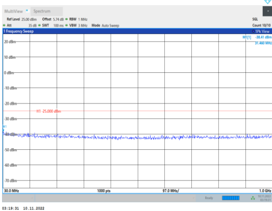
Band41-20MHz-QPSK-40640-1RB#0- Range1:30~1000MHz
