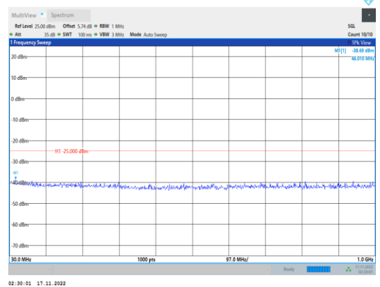
Band41-20MHz-64QAM-41140-1RB#0- Range1:30~1000MHz
