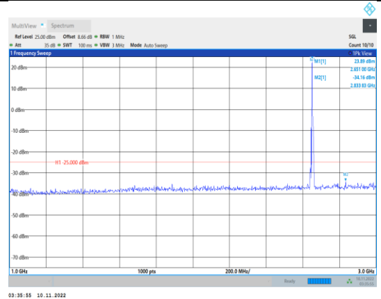
Band41-5MHz-16QAM-41215-1RB#0- Range2:1000~3000MHz
