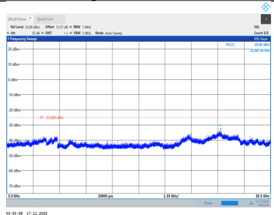
Band38-20MHz-64QAM-38150-1RB#0- Range3:3000~26500MHz
