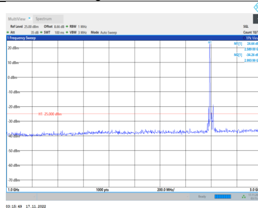
Band38-15MHz-64QAM-38000-1RB#0- Range2:1000~3000MHz
