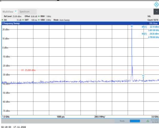
Band41-5MHz-64QAM-41215-1RB#0- Range2:1000~3000MHz
