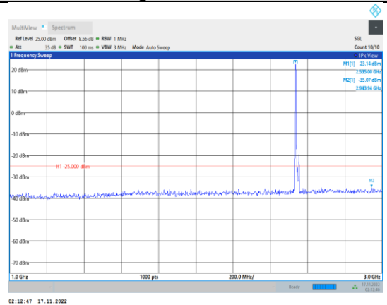
Band41-10MHz-64QAM-40090-1RB#0- Range2:1000~3000MHz
