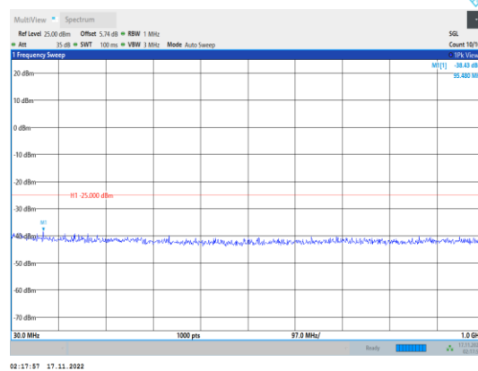
Band41-5MHz-64QAM-40640-1RB#0- Range1:30~1000MHz
