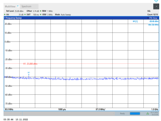
Band41-5MHz-16QAM-41215-1RB#0- Range1:30~1000MHz
