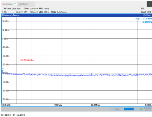
Band41-15MHz-64QAM-41165-1RB#0- Range1:30~1000MHz
