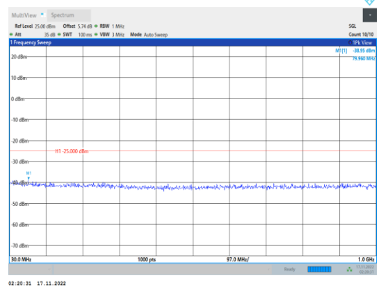
Band41-15MHz-64QAM-40640-1RB#0- Range1:30~1000MHz
