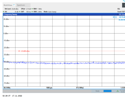
Band41-20MHz-64QAM-40140-1RB#0- Range1:30~1000MHz
