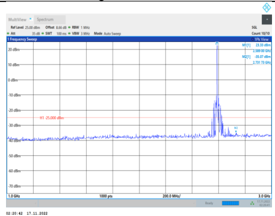
Band41-15MHz-64QAM-40640-1RB#0- Range2:1000~3000MHz
