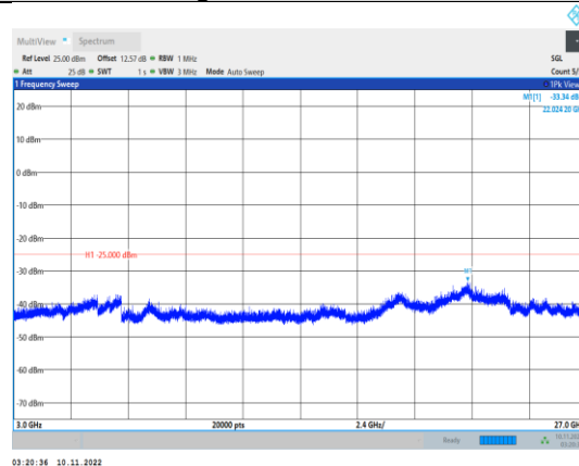
Band41-20MHz-16QAM-40640-1RB#0- Range3:3000~27000MHz
