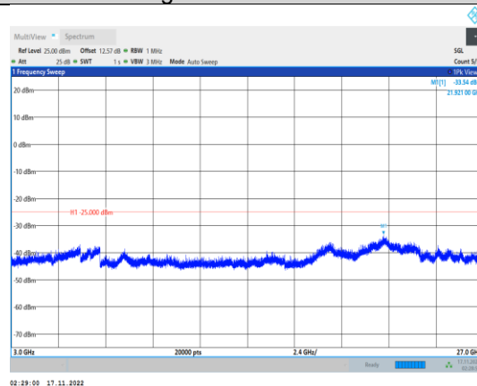
Band41-20MHz-64QAM-40140-1RB#0- Range3:3000~27000MHz
