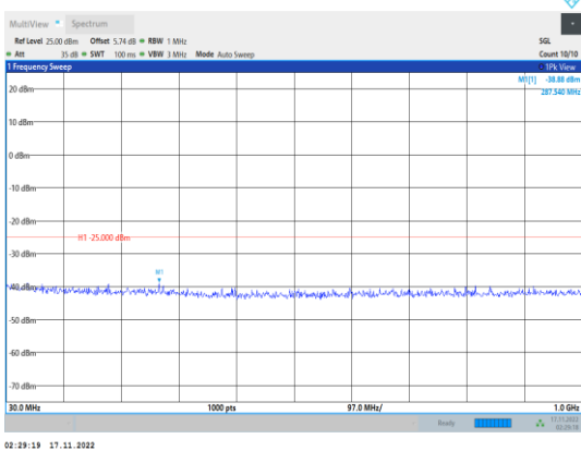
Band41-20MHz-64QAM-40640-1RB#0- Range1:30~1000MHz
