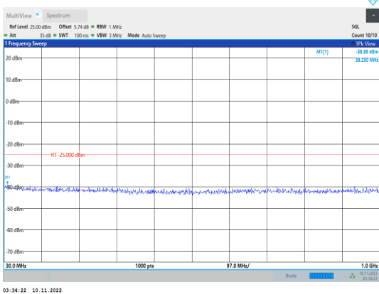
Band41-5MHz-16QAM-40640-1RB#0- Range1:30~1000MHz
