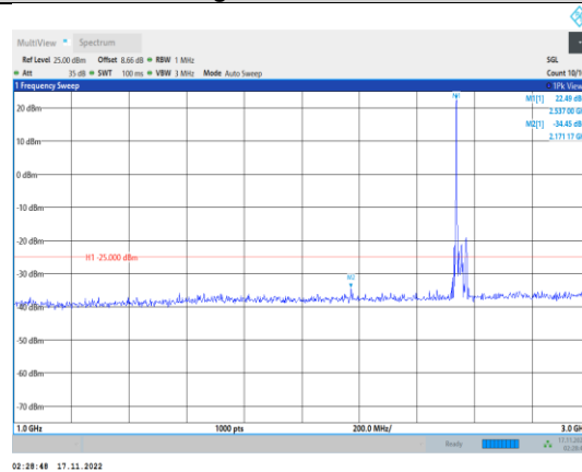
Band41-20MHz-64QAM-40140-1RB#0- Range2:1000~3000MHz
