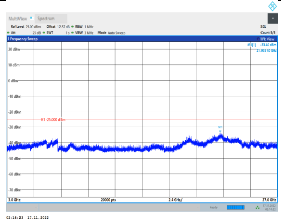
Band41-10MHz-64QAM-41190-1RB#0- Range3:3000~27000MHz
