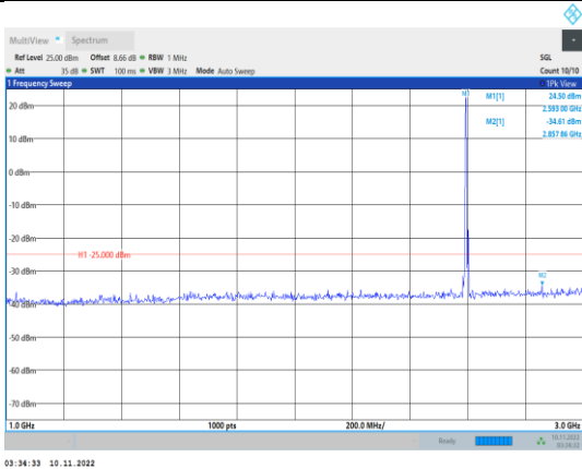
Band41-5MHz-16QAM-40640-1RB#0- Range2:1000~3000MHz
