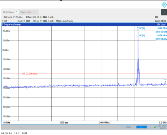
Band41-10MHz-16QAM-41190-1RB#0- Range2:1000~3000MHz
