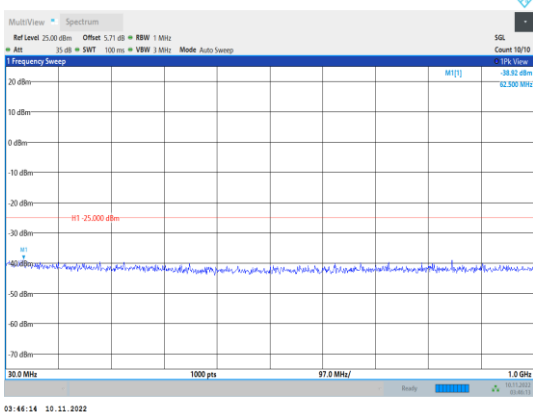
Band38-20MHz-16QAM-38150-1RB#0- Range1:30~1000MHz
