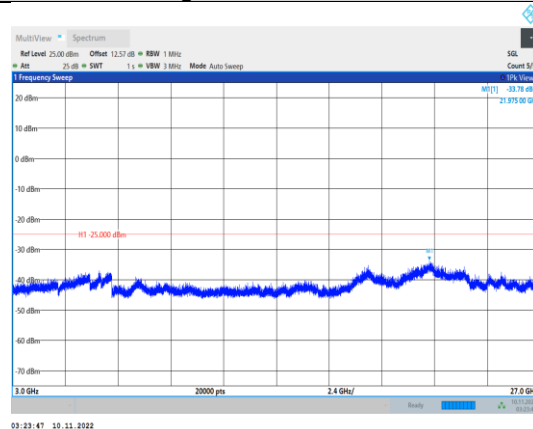
Band41-15MHz-16QAM-40115-1RB#0- Range3:3000~27000MHz
