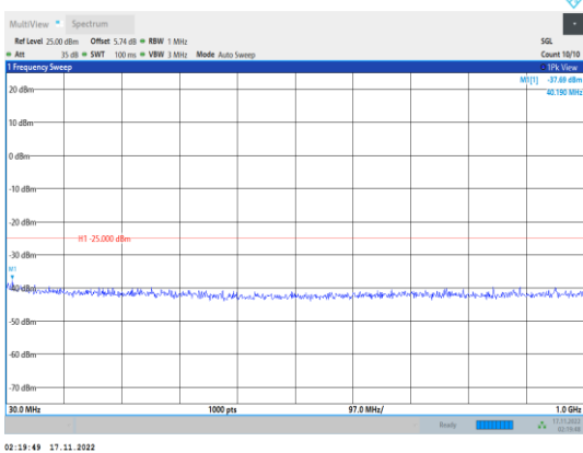
Band41-15MHz-64QAM-40115-1RB#0- Range1:30~1000MHz
