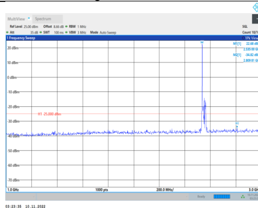
Band41-15MHz-16QAM-40115-1RB#0- Range2:1000~3000MHz
