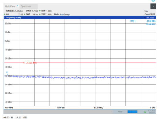
Band41-5MHz-QPSK-40640-1RB#0- Range1:30~1000MHz
