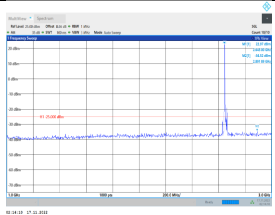
Band41-10MHz-64QAM-41190-1RB#0- Range2:1000~3000MHz
