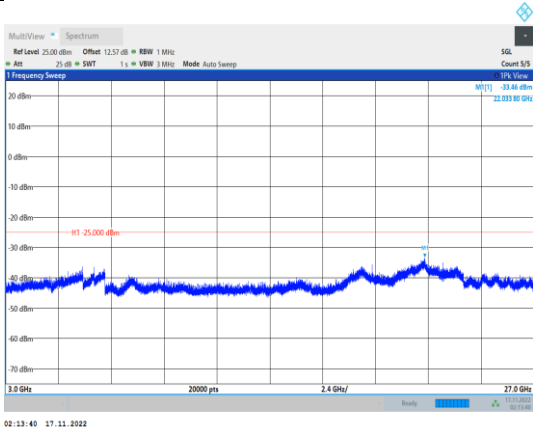
Band41-10MHz-64QAM-40640-1RB#0- Range3:3000~27000MHz
