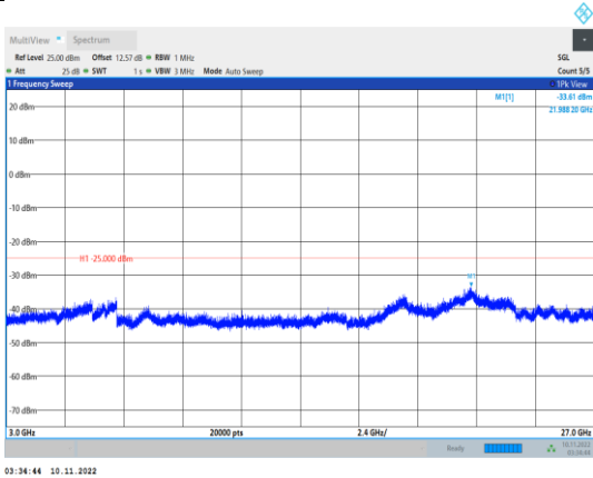
Band41-5MHz-16QAM-40640-1RB#0- Range3:3000~27000MHz
