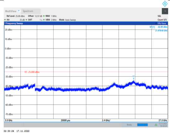
Band41-20MHz-64QAM-41140-1RB#0- Range3:3000~27000MHz
