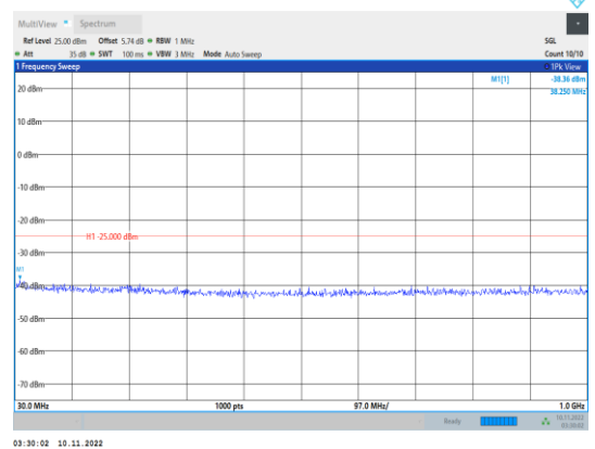
Band41-10MHz-QPSK-41190-1RB#0- Range1:30~1000MHz
