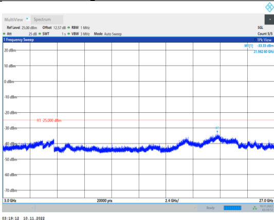
Band41-20MHz-16QAM-40140-1RB#0- Range3:3000~27000MHz
