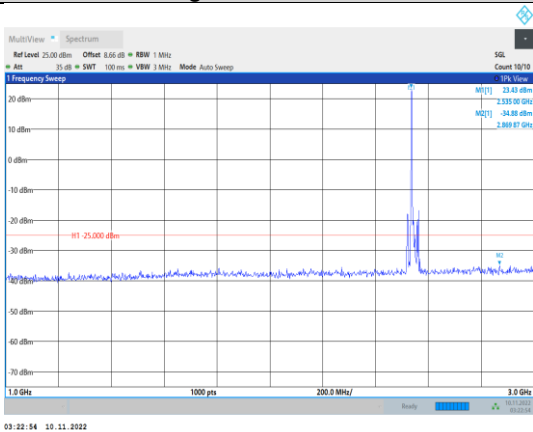
Band41-15MHz-QPSK-40115-1RB#0- Range2:1000~3000MHz
