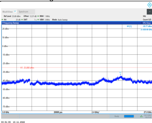
Band41-10MHz-16QAM-41190-1RB#0- Range3:3000~27000MHz
