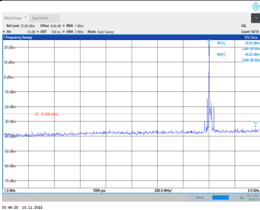
Band38-20MHz-16QAM-38150-1RB#0- Range2:1000~3000MHz
