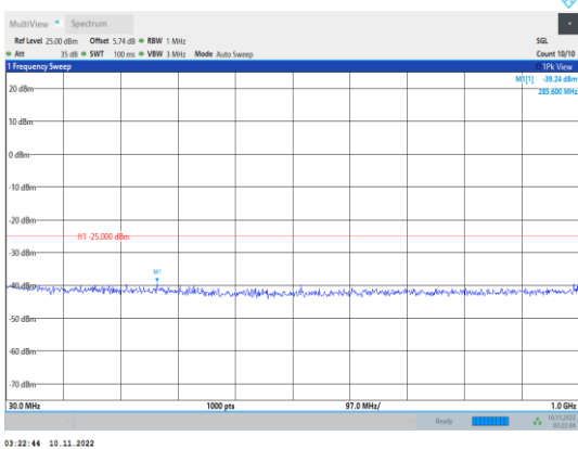
Band41-15MHz-QPSK-40115-1RB#0- Range1:30~1000MHz
