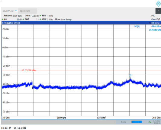
Band38-20MHz-16QAM-38150-1RB#0- Range3:3000~26500MHz
