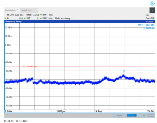
Band41-15MHz-16QAM-41165-1RB#0- Range3:3000~27000MHz
