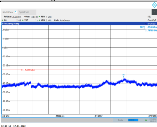
Band41-15MHz-64QAM-40115-1RB#0- Range3:3000~27000MHz
