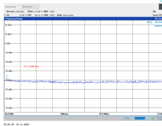
Band41-20MHz-QPSK-41140-1RB#0- Range1:30~1000MHz
