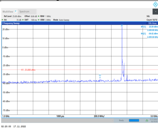
Band41-15MHz-64QAM-40115-1RB#0- Range2:1000~3000MHz
