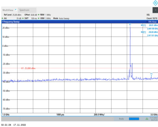
Band41-15MHz-64QAM-41165-1RB#0- Range2:1000~3000MHz
