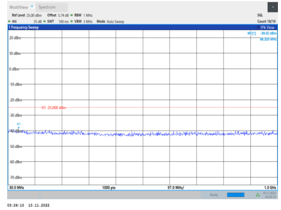
Band41-15MHz-16QAM-41165-1RB#0- Range1:30~1000MHz
