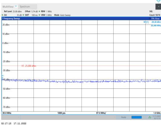
Band41-5MHz-64QAM-40065-1RB#0- Range1:30~1000MHz
