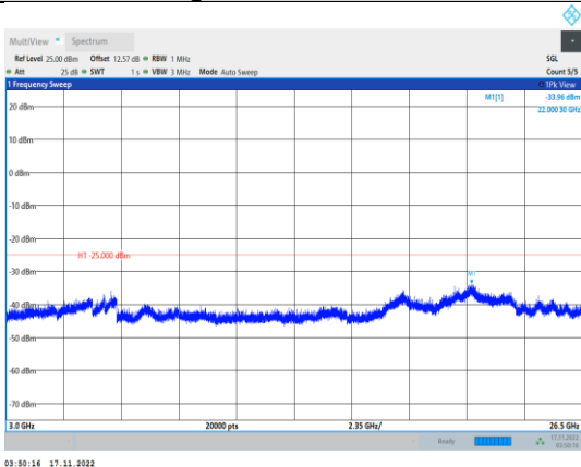
Band38-20MHz-64QAM-38000-1RB#0- Range3:3000~26500MHz
