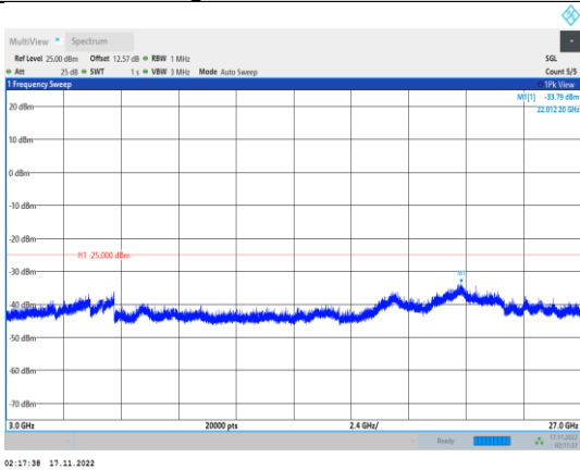
Band41-5MHz-64QAM-40065-1RB#0- Range3:3000~27000MHz
