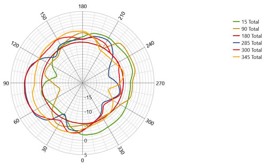
Radiation Pattern for 2.4G Antenna (2445MHz)
