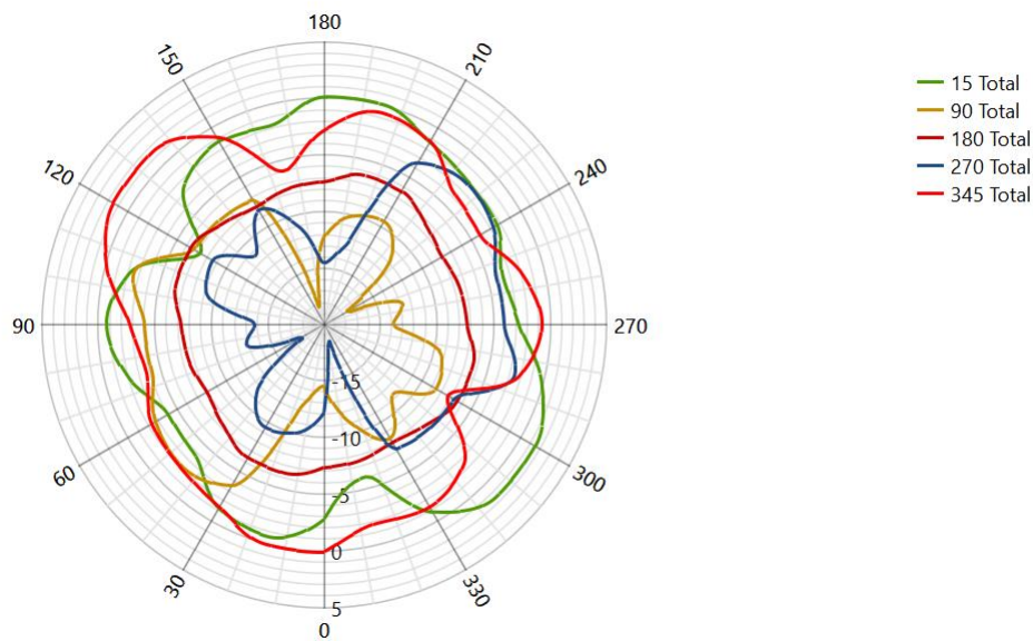
Radiation Pattern for 5G Antenna (5210MHz)
